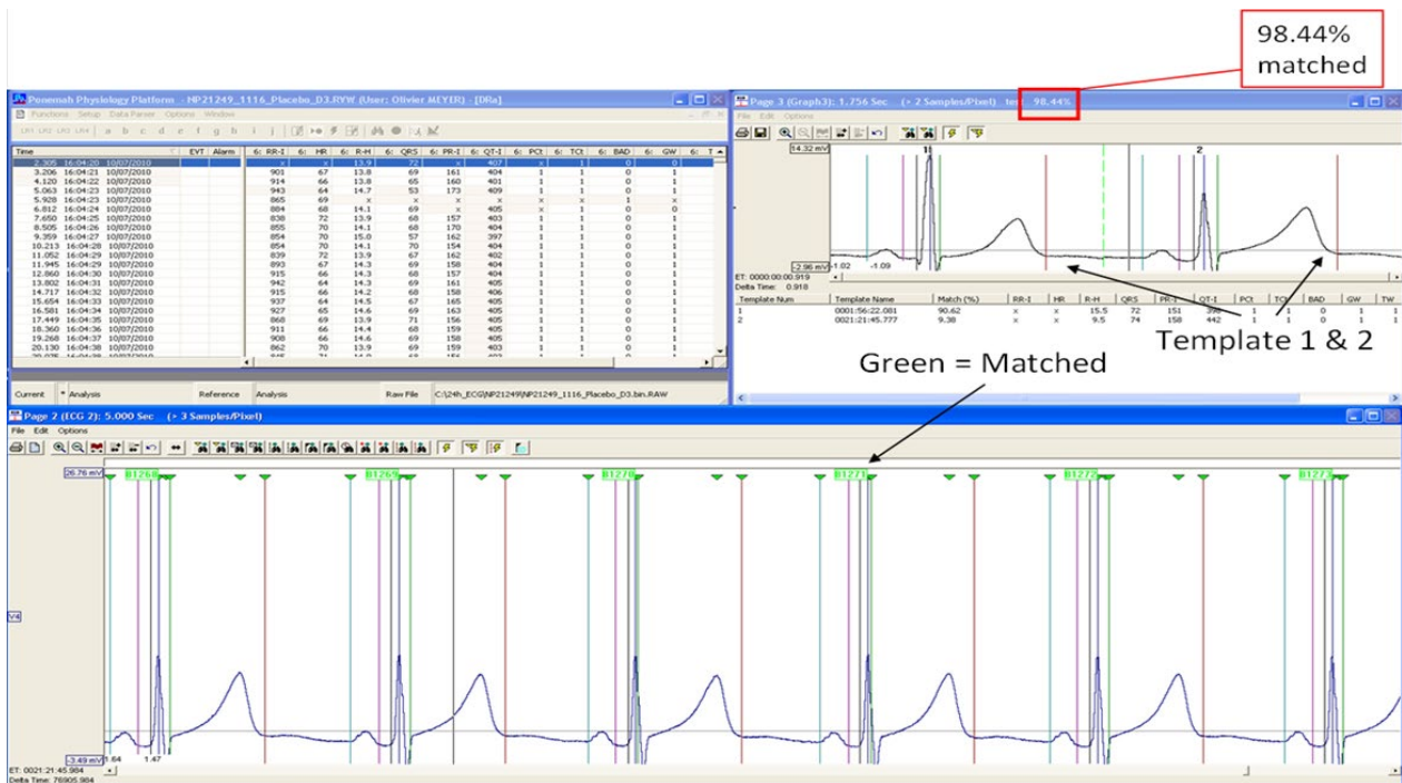
Figure 31. Ponemah's pattern recognition module. The subject-specific library (top right) includes templates which serve as the basis to measure the 24 h continuous ECG recording (bottom). In this example, 2 templates were sufficient for the recognition of 98.44% of all waveforms. When the pattern recognition process is completed, the ECG intervals are saved in the new DRa file (top left).
