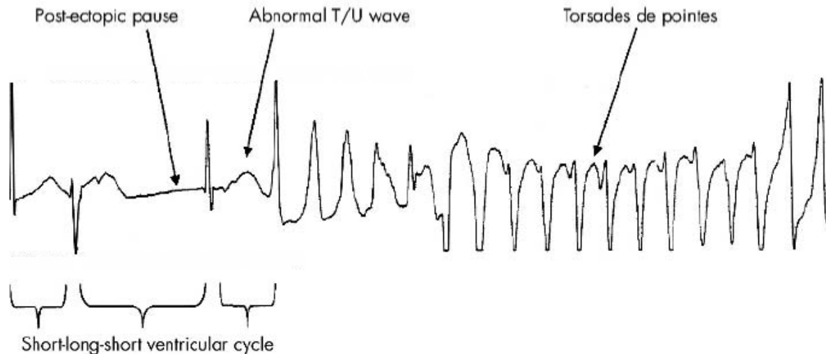
Figure 11. Drug-induced TdP with the typical short-long-short initiating ventricular cycle (from Yap 2003).
