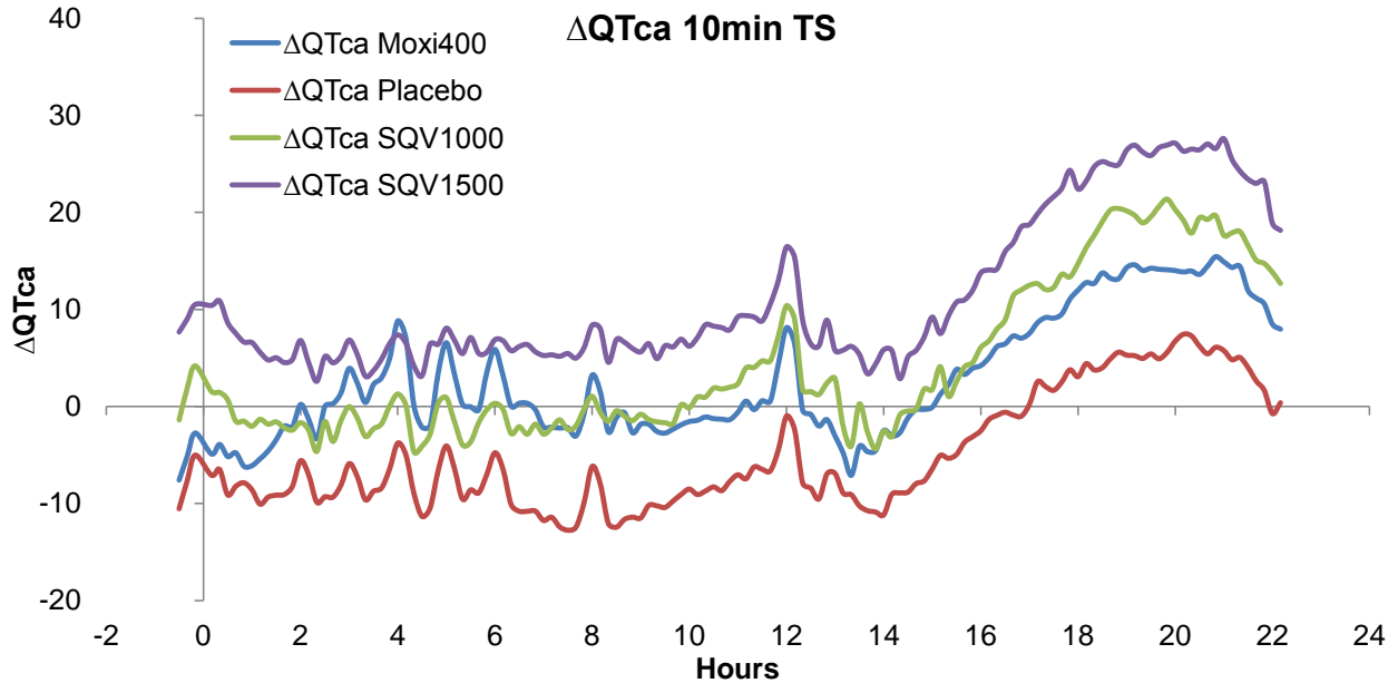
Figure 52A. PRO-derived \Delta QTca for each treatment with 10 min time segments. The fast protocol-induced effects are smoothed by the 10-min time segments.
