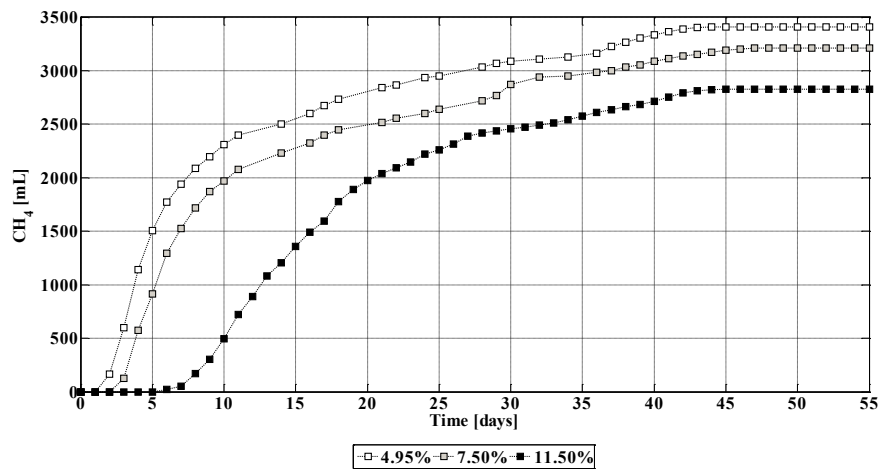
Figure 5. Effect of TS on the cumulated methane production from anaerobic digestion of carrots waste.
