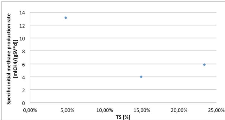
Figure 25. Not linear correlation between specific methane production and TS content.
