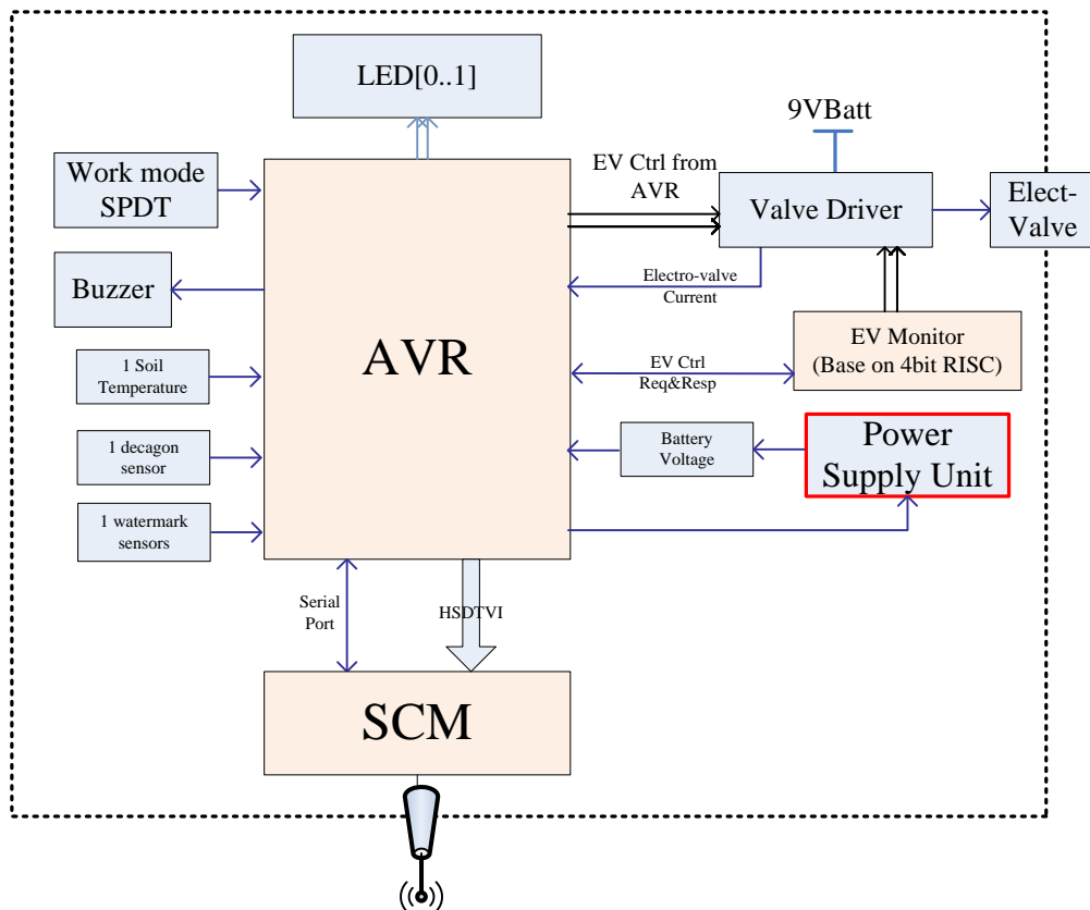
Figure 5-8 Example Multicore WSN Architecture Diagram
