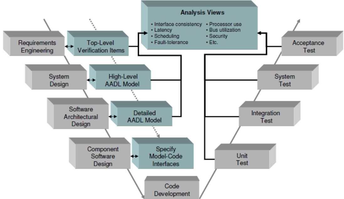
Figure 5-9 Early Validation Based on AADL
