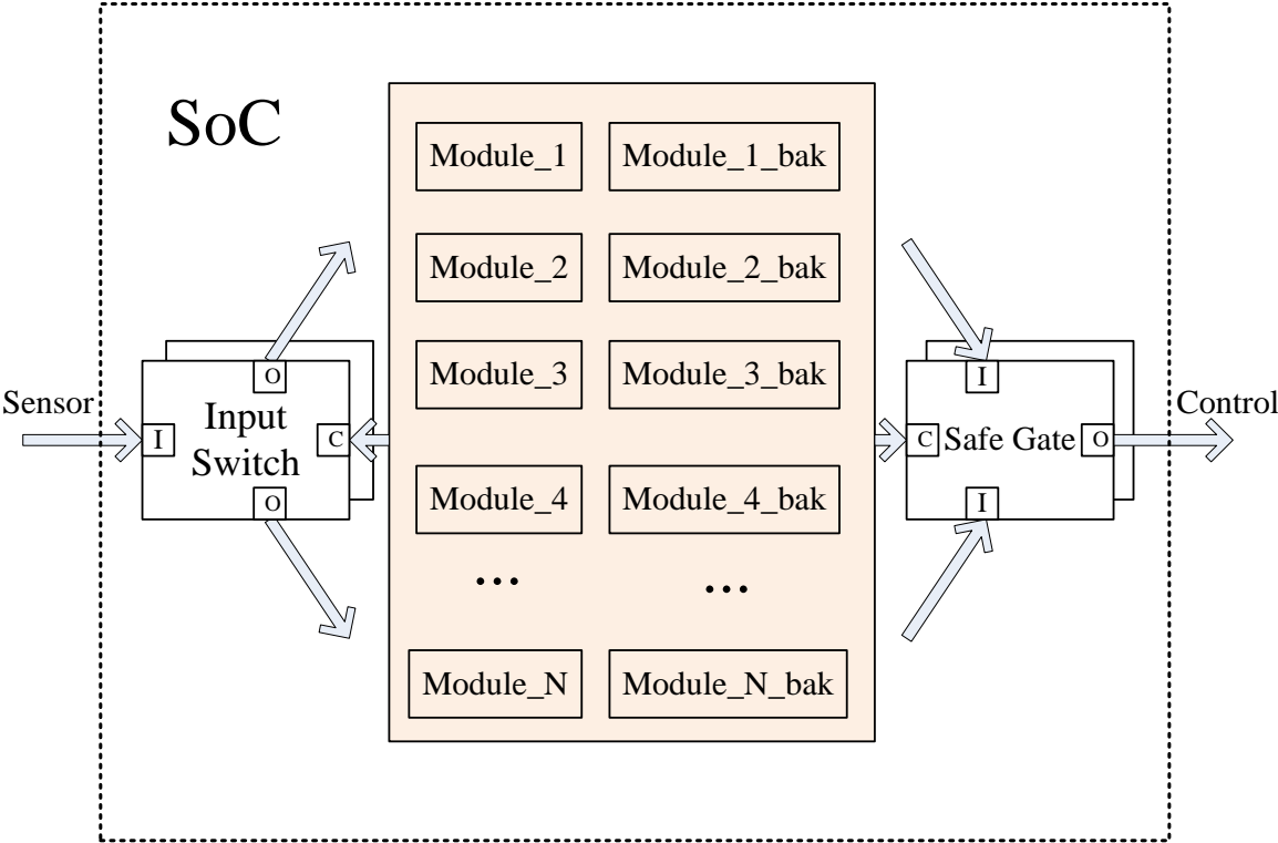
Figure 7-4 FSMOS Modules based the Multicore SoC
