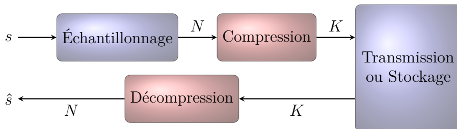
FIGURE 1.5 – Paradigme classique
