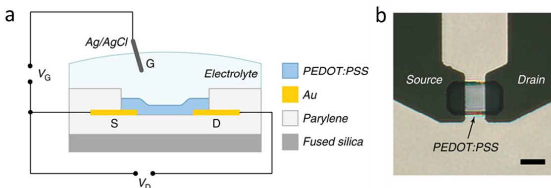
Figure 1.16: (a) Schematic of an OECT cross-section and the wiring diagram for device operation. (b) Optical micrograph of an individual transistor. Scale bar, 10 \mu\text{m} . Adapted from [1.85].
