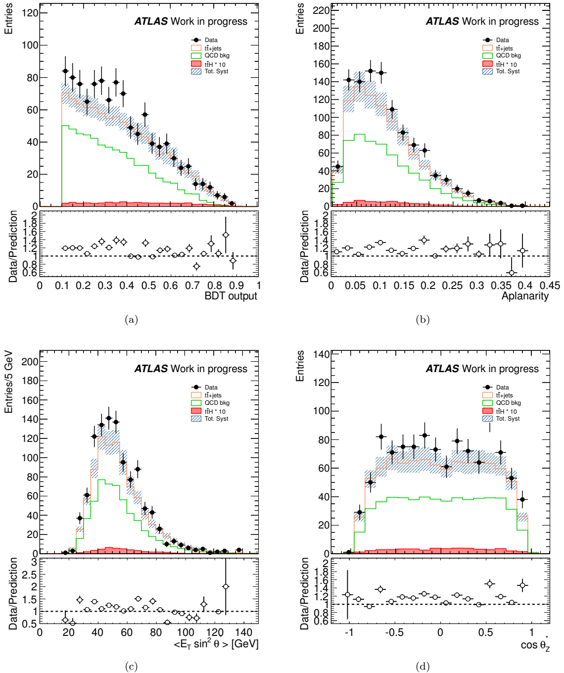
FIGURE 5.18 Data and background prediction in the exclusive three b -tagged jets region for the BDT output variable 5.18(a) as well as for the BDT input variables: aplanarity 5.18(b), average of the transverse energy multiply by \sin \theta^* 5.18(c) and \cos \theta^* not boosted in the x and y axes 5.18(d). The shaded area represents the total systematic uncertainty (see Section 5.11 for the systematic uncertainties estimation). Data are represented with black markers. The orange and green histograms represent t\bar{t}+\text{jets} and QCD respectively. The red histogram represents the t\bar{t}H(H \rightarrow b\bar{b}) . To better visualize it the signal contribution is multiplied by a factor of 10. The bottom panel displays the ratio between data and background prediction.
