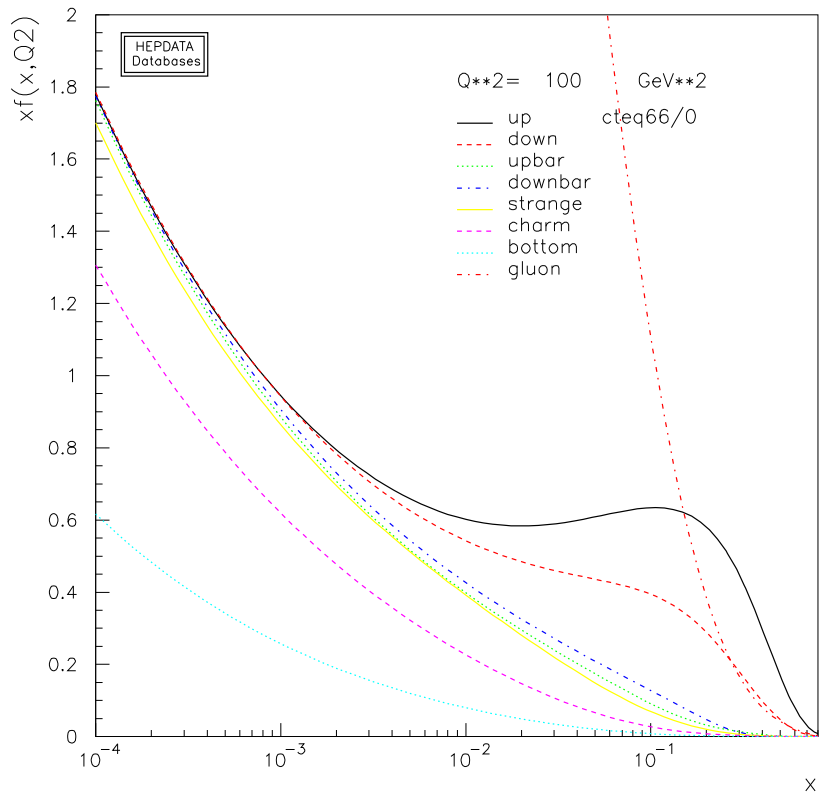
FIGURE 1.12 Parton distribution function for protons in the CTEQ66 PDF set [44] at Q^2 = 100 GeV [45].
