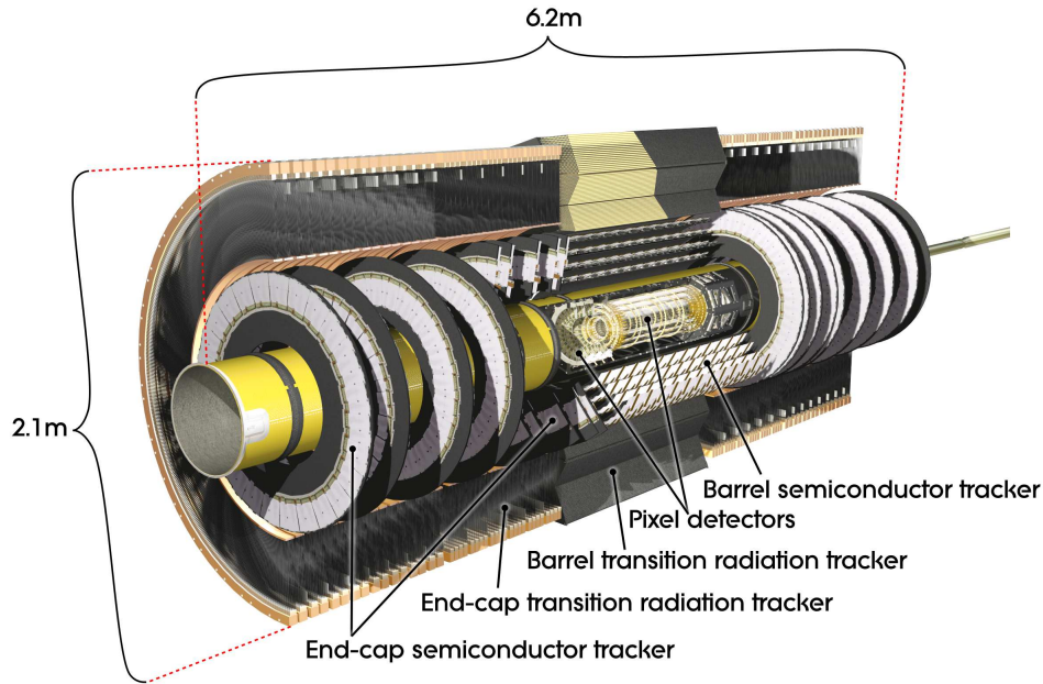
FIGURE 2.4 Cut-away view of the ATLAS Inner Detector [71, 72].
