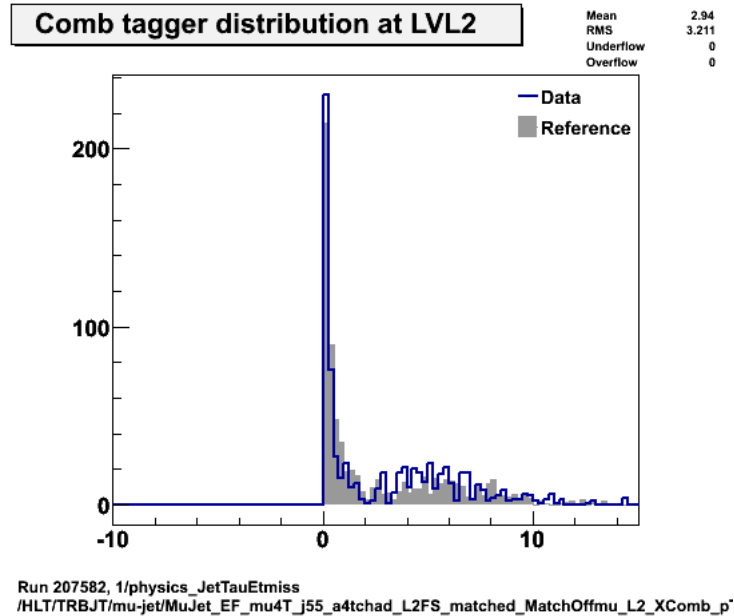
FIGURE 3.19 Histograms taken from the web display of Tier-0 offline monitoring. Core distribution of the XComb tagger weight for all the events passing a \mu -jet trigger criteria and a cut on p_T^{rel} > 2 GeV. The blue line represents the selected data run to be check, whereas the filled histogram represents the reference.
