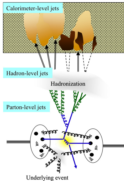
FIGURE 4.2 pp scattering in different phases. The initial pair of partons forms jets. The image shows the phase just before the hadronization (parton jets), after the hadronization (particle jets) and the calorimeter jets reconstructed from the particles energy deposition in the calorimeter.
