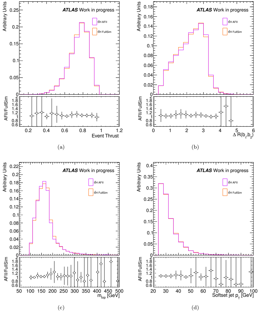
FIGURE 5.11 Comparison of AFII and FullSim for the fully hadronic t\bar{t}H ( H \rightarrow b\bar{b} ) sample. Four BDT input variables are presented: for event thrust (5.11(a)), \Delta R(b_1, b_2) (5.11(b)), top floating mass (5.11(c)) and softest jet p_T (5.11(d)). The purple histograms represent AFII simulation, the orange ones represent FullSim. The uncertainties on the ratio are statistical only.
