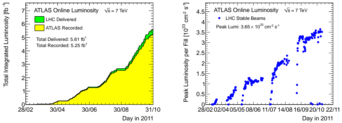
FIGURE 2.2 Cumulative luminosity versus day delivered to by the LHC (green), and recorded by ATLAS (yellow) during stable beams and for pp collisions at 7 TeV center-of-mass energy in 2011 in the left side. At right side the maximum instantaneous luminosity versus day delivered to ATLAS in the 2011 [66].
