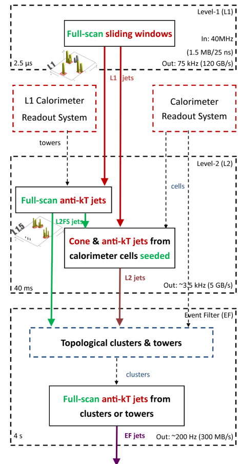
FIGURE 3.3 Architecture of ATLAS Jet Trigger System. The topological cluster label identifies the clusters derived from calorimeter cells by adding the energy in neighbouring cells if they have an energy larger than a pre-defined threshold.
