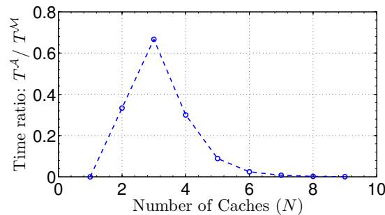
Figure 4.18: Computation time comparison on linear networks
