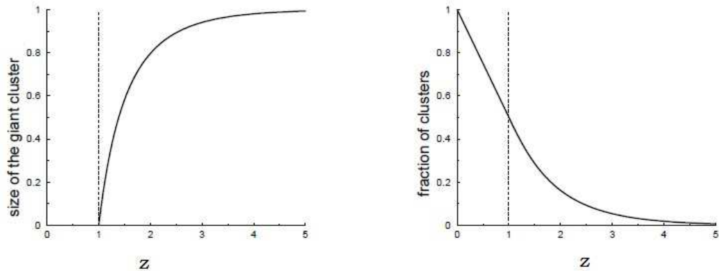
Figure A.2: Size of the largest cluster and fraction of cluster by vertice as a function of the parameter z . a
