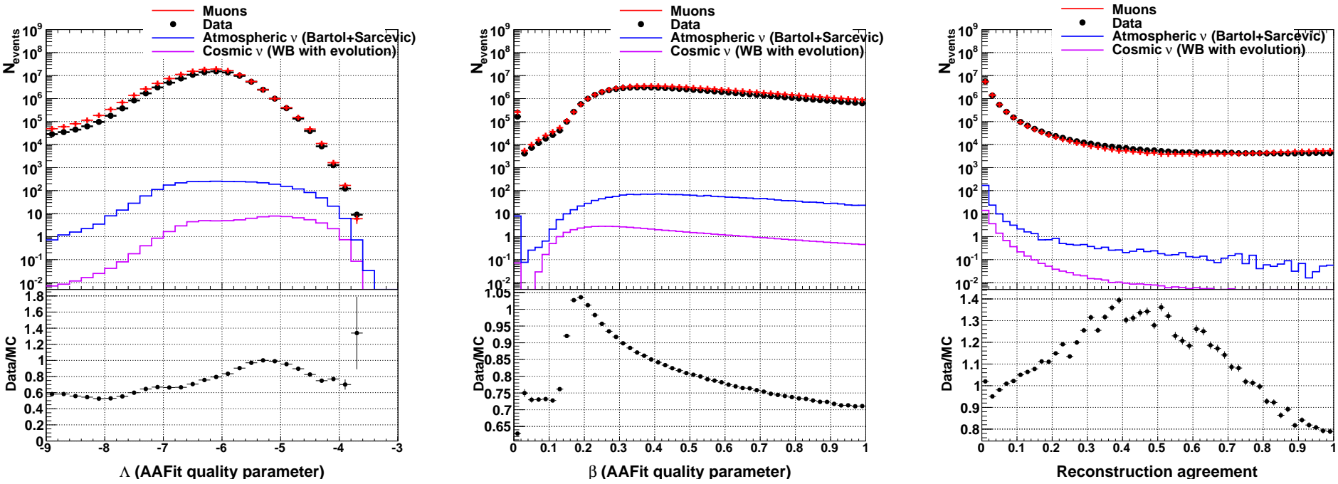
Figure B.1: Left: \Delta : data and Monte Carlo are in a good agreement, reproducing quite the same slope. Center: \beta : globally the agreement between data and simulation is good. Right: reconstruction agreement data and Monte Carlo are compatible, showing an acceptable agreement on the whole range.
