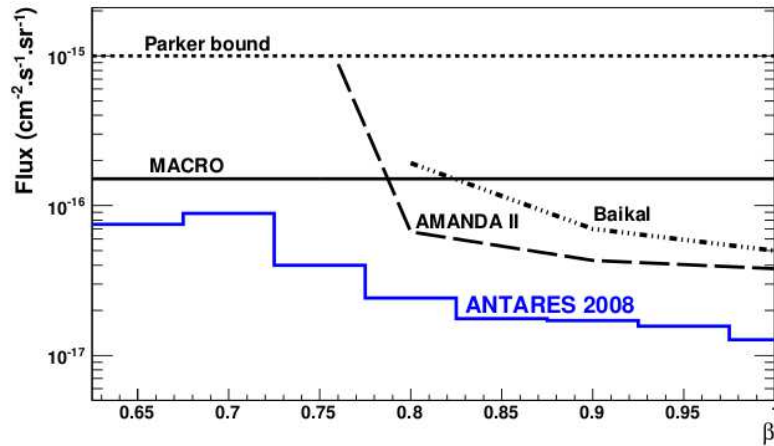
Figure 1.13: The ANTARES 90% C.L. upper limit on upgoing magnetic monopoles, compared to the theoretical Parker bound, the published upper limit obtained by MACRO for an isotropic flux of monopoles as well as the upper limits from Baikal and AMANDA for upgoing monopoles [36].
