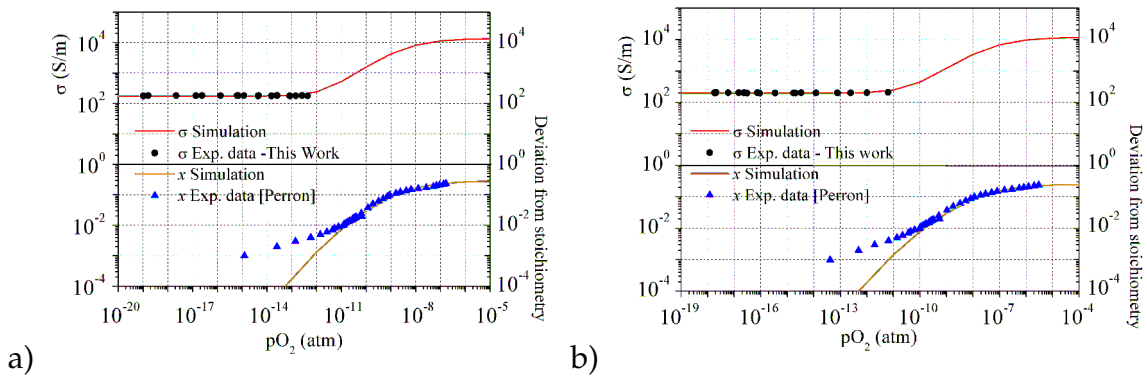
Figure 6.3: Fit of electrical conductivity and deviation from stoichiometry data taken at 893°C (a) and 993°C (b) for chromium doped material.
