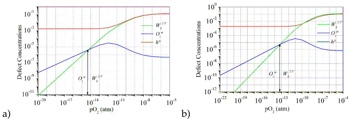
Figure 6.4: Calculated defect concentrations at a temperature equal to 893°C (a) and to 993°C for chromium doped material (b).
