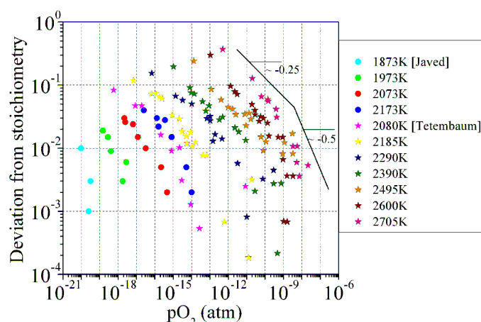
Figure 1.4: Dependence upon oxygen partial pressure of the deviation from stoichiometry x : comparison between data taken at different temperatures reported by Javed [101] and Tettembaum [173].
