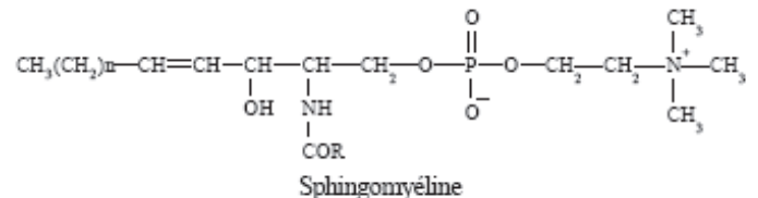
Céramide phosphorylcholine
