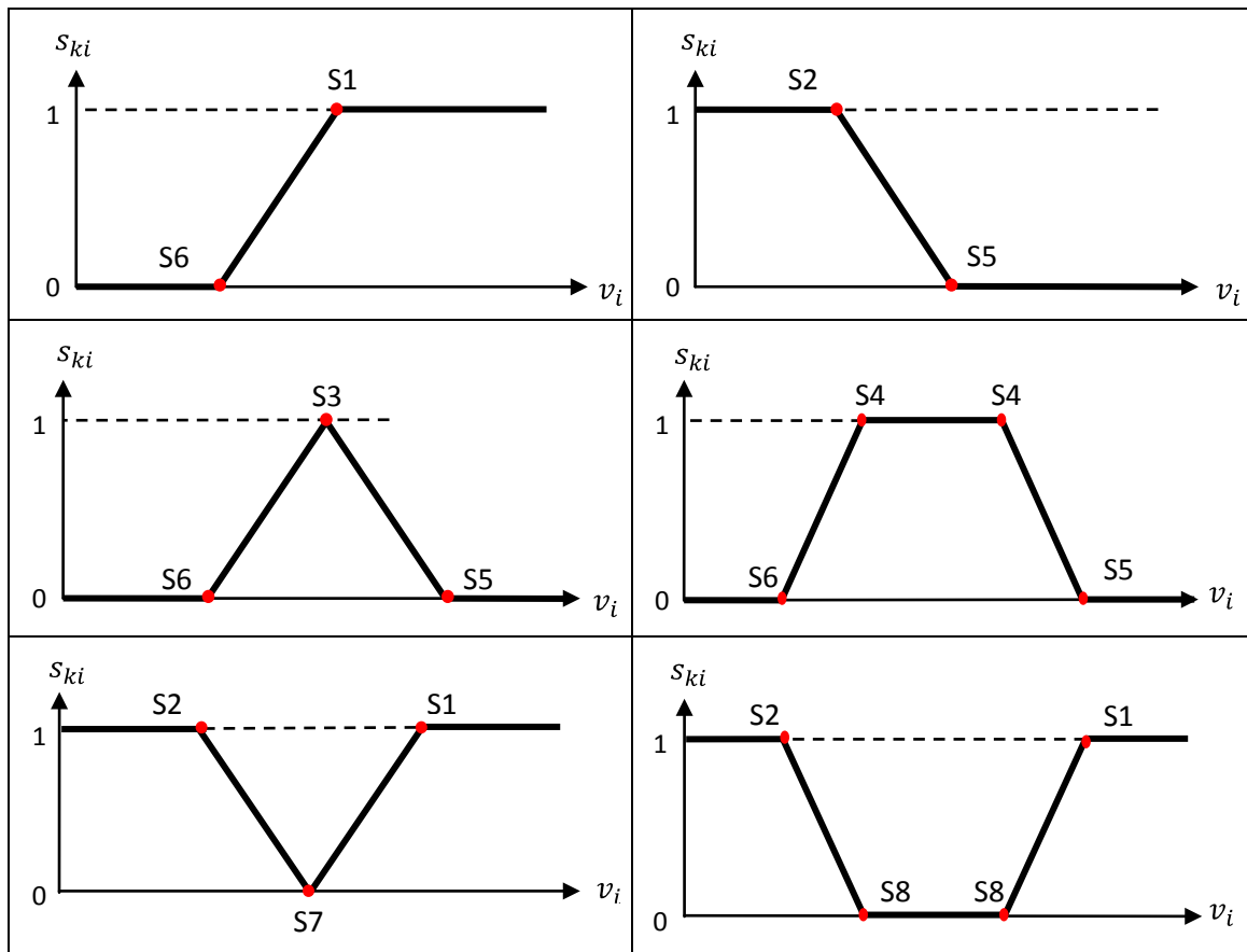
Figure 2.4: Satisfaction functions
