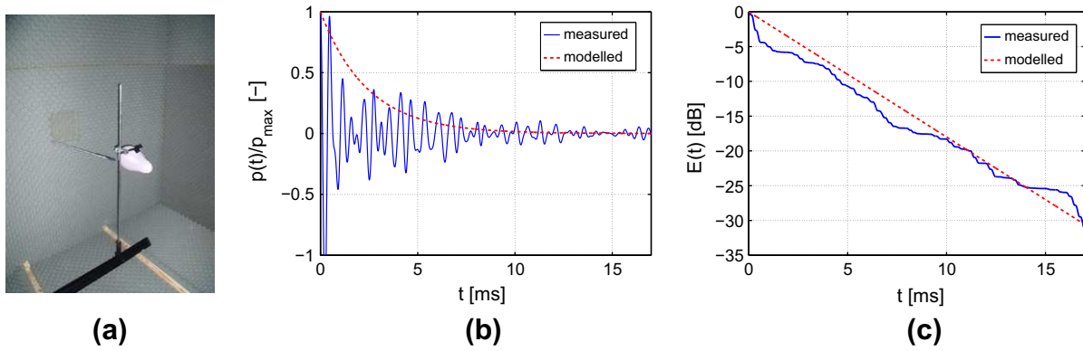
Fig. 6. (a) Illustration of setup used to generate an impulse response in the insulation box due to a balloon burst. A trapdoor is used to cause the balloon burst without an experimenter present. (b) Example of normalised measured impulse response h(t) (full line) and modelled impulse response \hat{h}(t) = e^{-\frac{13.8t}{Tr_m}} (dashed line). (c) Example of Schroeder integral E(t) obtained from the measured (full line) and modelled (dashed line) impulse response.
