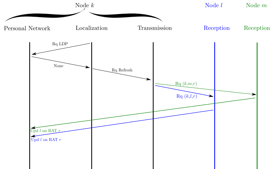
Fig. 4.6: Example of communication process initiated by the localization stage of node k . Because no information are available to estimate its position, the localization stage of node k requests a communication. The transmission stage of node k sends request to node l and m . Both nodes will thus update the personal network of node k .
