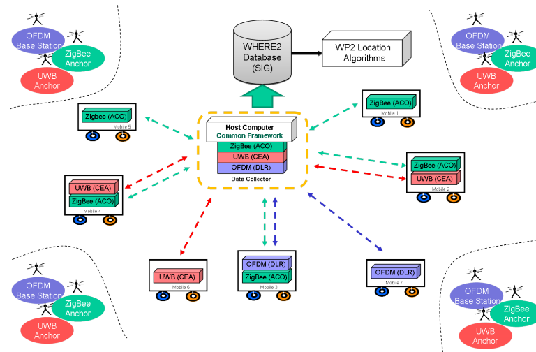
Fig. 5.1: Where 2 measurement platform. Different radio technologies (ZigBee, IR-UWB, OFDM) are embedded on a mobile Trolley
