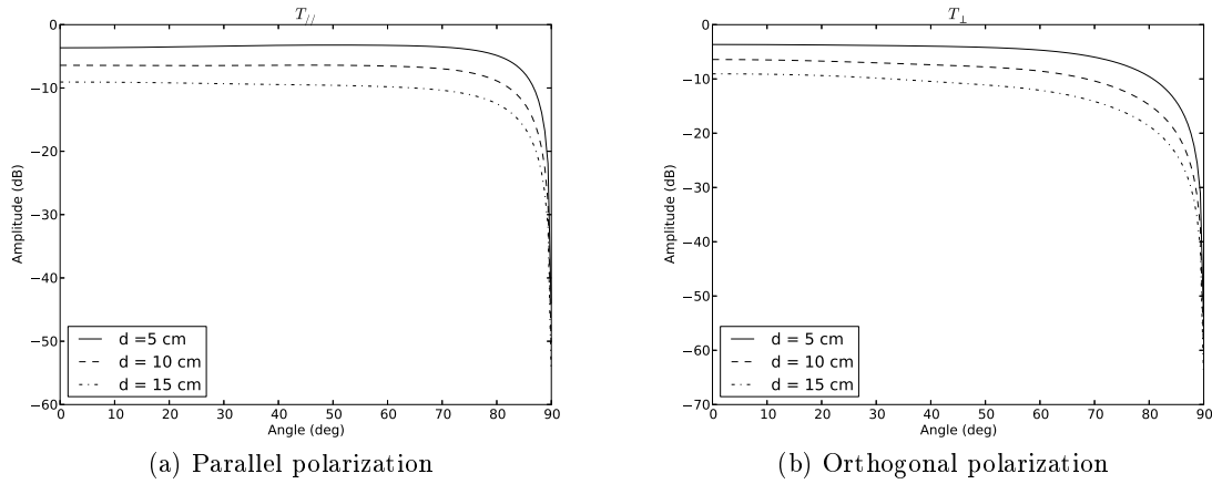
Fig. 2.26: Module of transmission coefficients as a function of the incidence angle for a (a) parallel polarization and an (b) orthogonal polarization with \epsilon_r = 3, \sigma = 0.06S/m and f = 4 GHz .
