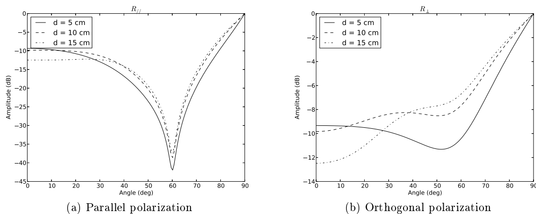
Fig. 2.25: Module of reflection coefficients as a function of the incidence angle for a (a) parallel polarization and an (b) orthogonal polarization with \epsilon_r = 3, \sigma = 0.06S/m and f = 4 GHz .
