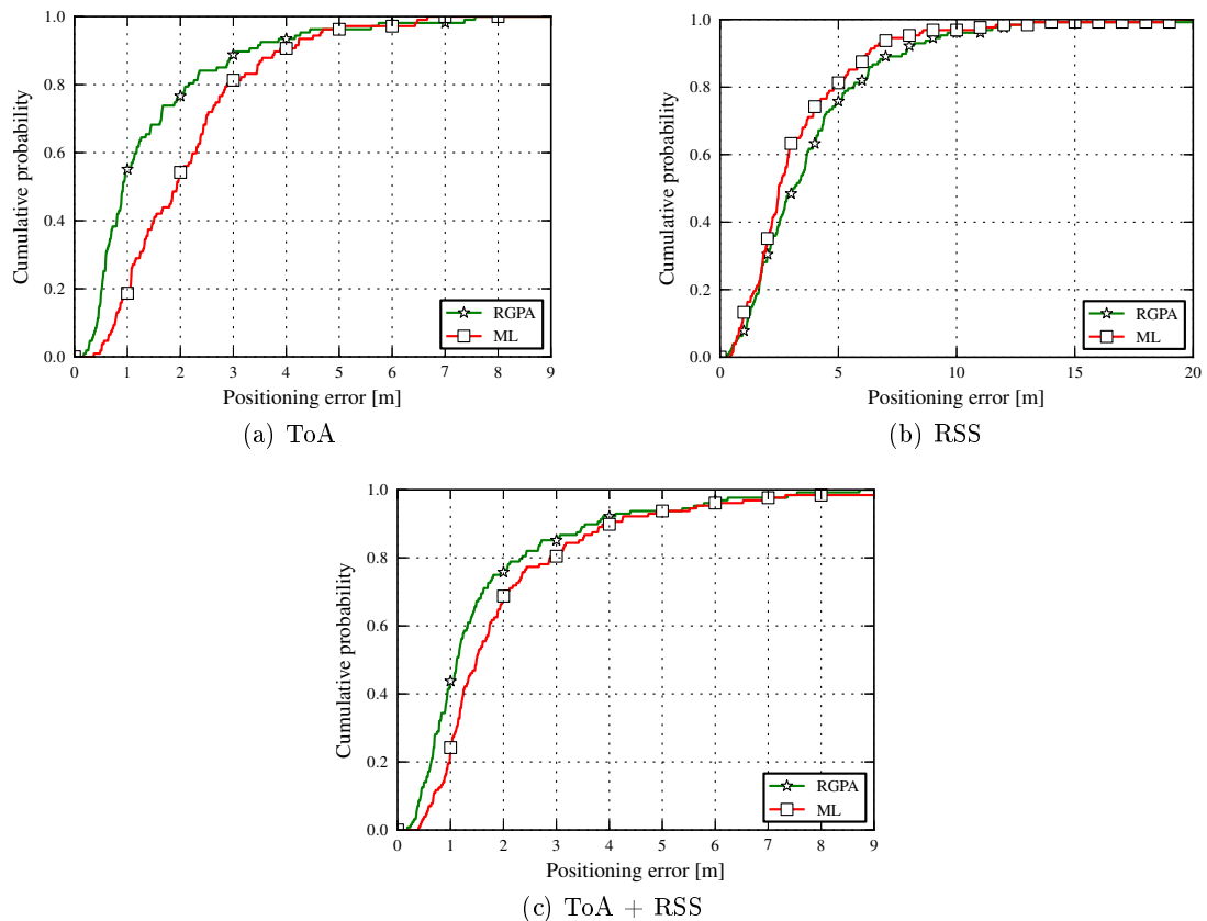
Fig. 5.15: CDFs of positioning error comparison between ML and RGPA algorithms using (a) IR-UWB ToA LDP and (b) Zigbee RSS LDP, (c) fusion of ToA and RSS LDPs.
