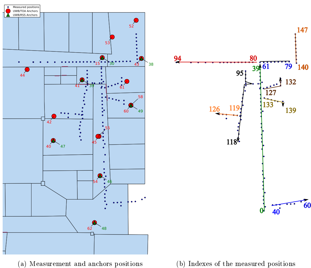
Fig. 5.3: Scenario 4: Both figures represent the Scenario 4 description. In (a) is represented the different trolley positions with blue dots, and the positions and name of ToA and RSS anchor nodes with red dots and green triangles respectively. In (b) is superimposed the measurement indexes of the trolley trajectory. The number associated to the tail and the head corresponds respectively to the first and the last measurement index of the set.
