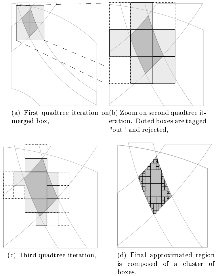
Fig. 3.8: The quadtree approximation to determine the enclosed and ambiguous boxes.
