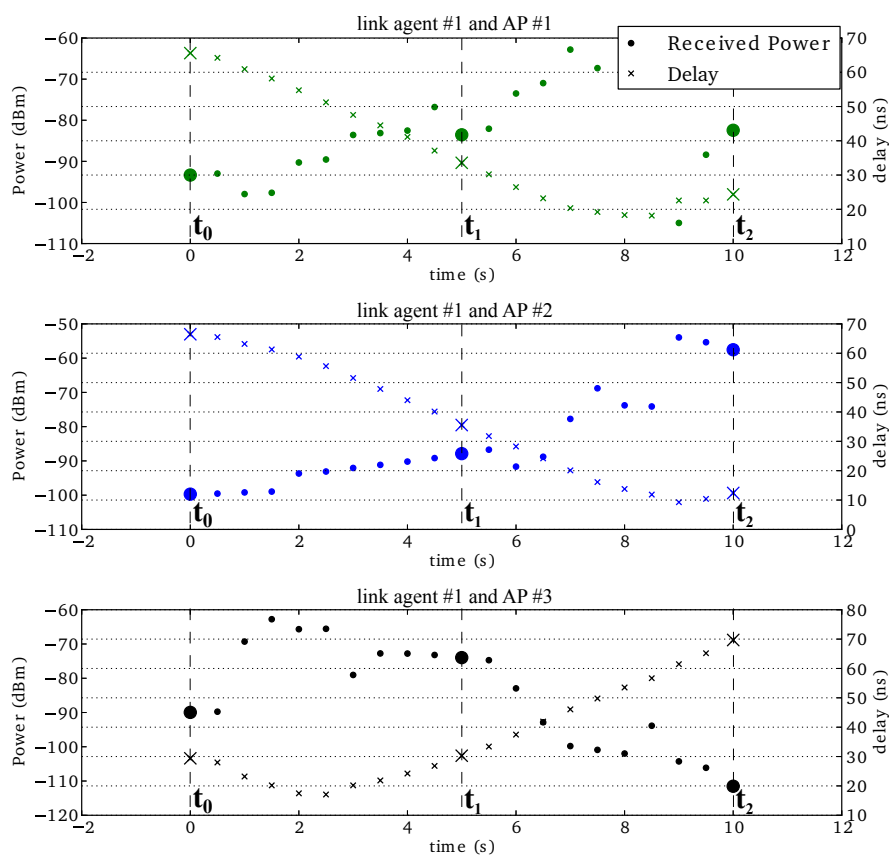
Fig. 4.8: The 3 figures correspond to 3 different radio links. On each figure are plot siulatneously the received power and the estimated delay as a function of the simulation time. Each dot corresponds to an estimation of received power value, whereas each cross correspond to an estimation of the delay .
