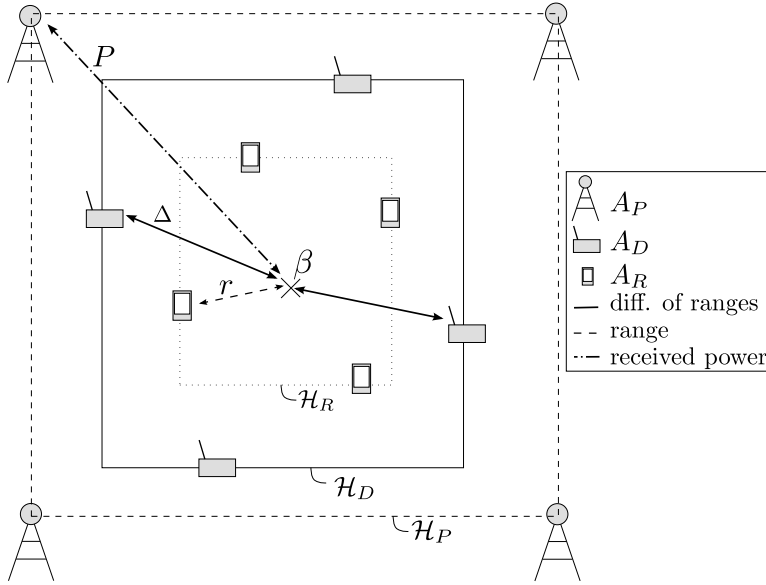
Fig. 3.12: A blind node at position \beta receives range observations \{r\} from anchors at positions \{A_R\} , difference of ranges observations \{\Delta\} from anchors at positions \{A_D\} and received power observations \{P\} from anchors at positions \{A_P\} .
