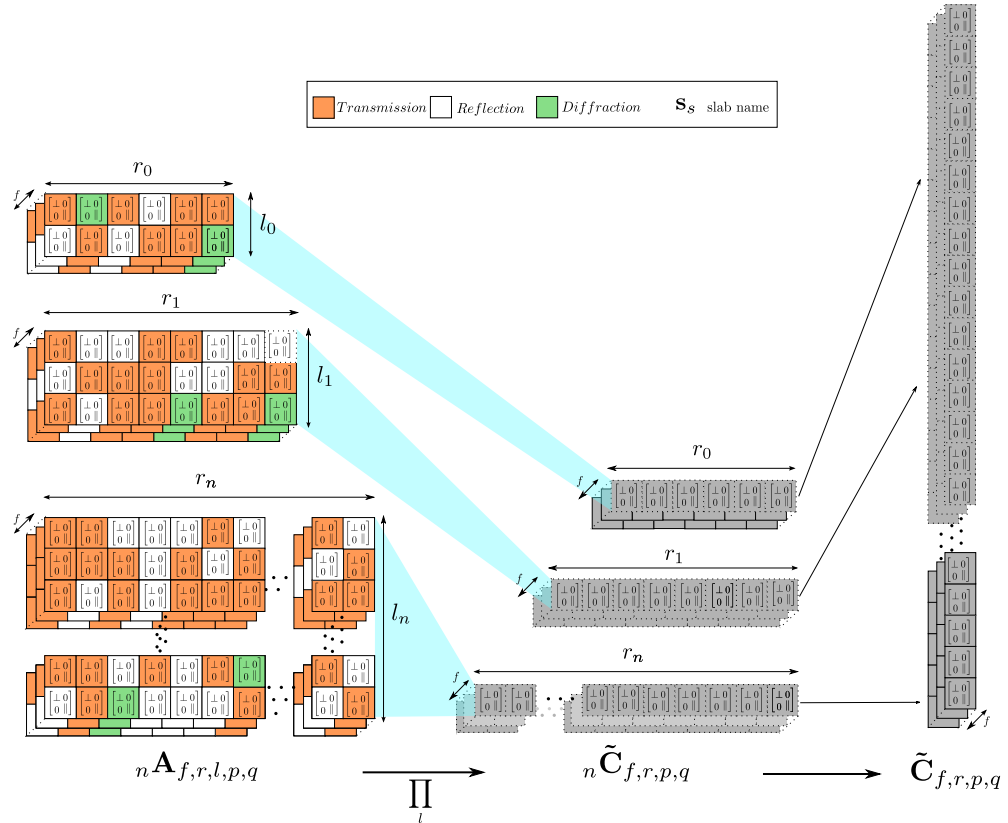
Fig. 2.23: Diagram showing how to obtain the propagation channel {}^{ab} \tilde{\mathbf{C}}_{f,r,p,q} for all the frequency range from the interactions MDA classified by \mathbf{L}_n blocks.
