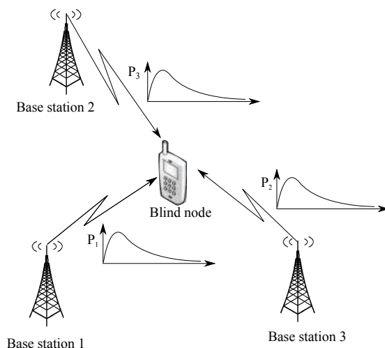
Fig. 3.1: Example of localization based on RSS.
