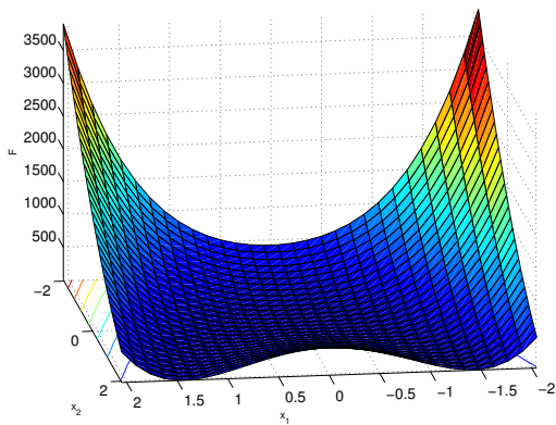
(c) Rosenbrock
