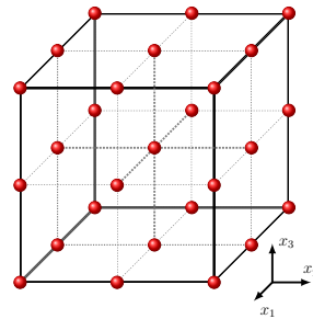
FIGURE 1.20 – Plan factoriel complet 3^3 (27 points)
