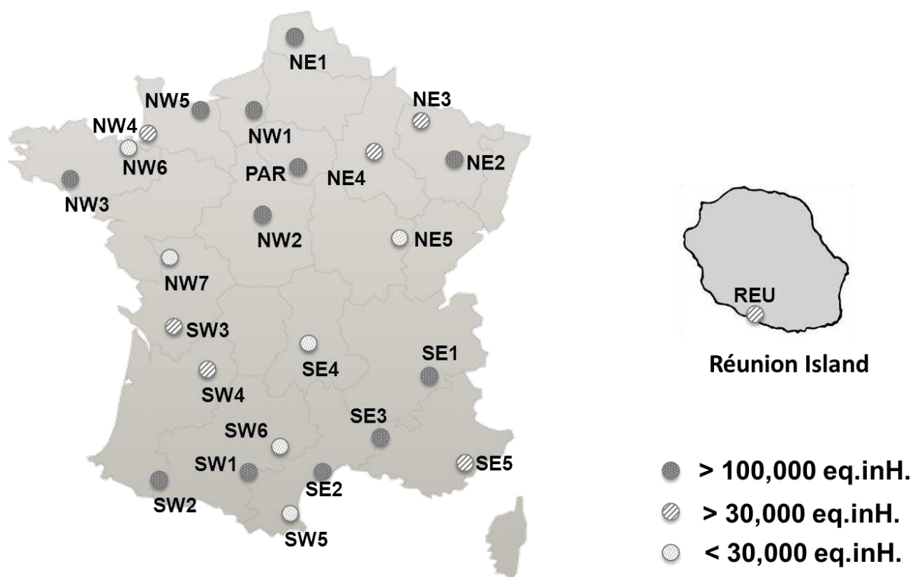
Figure 1 – Location of investigated STPs.
