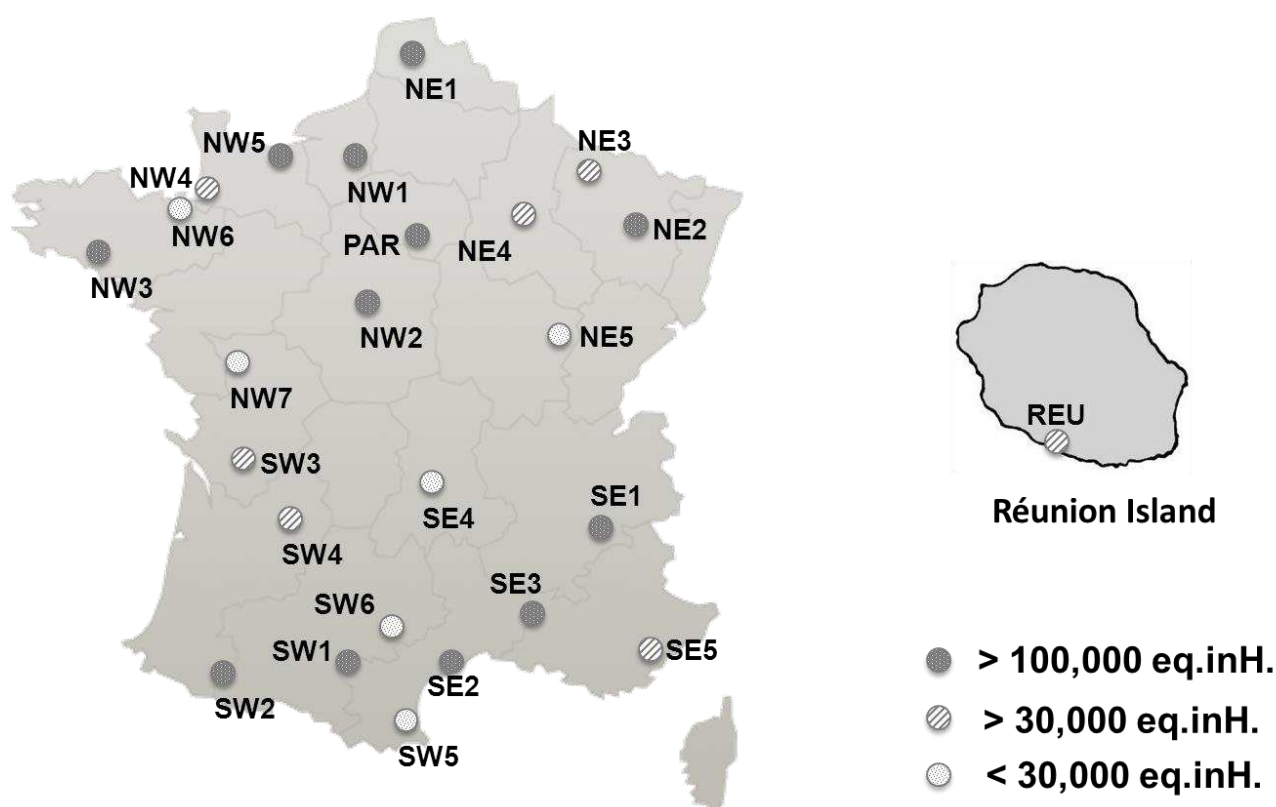
Figure 1 – Location of investigated STPs.
