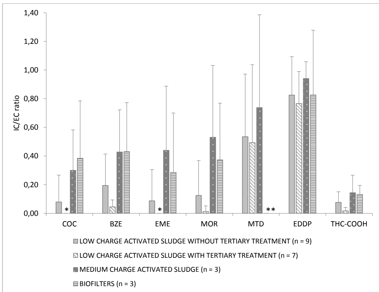
Figure 4 – Mean IC/EC ratio depending on STP treatments.
