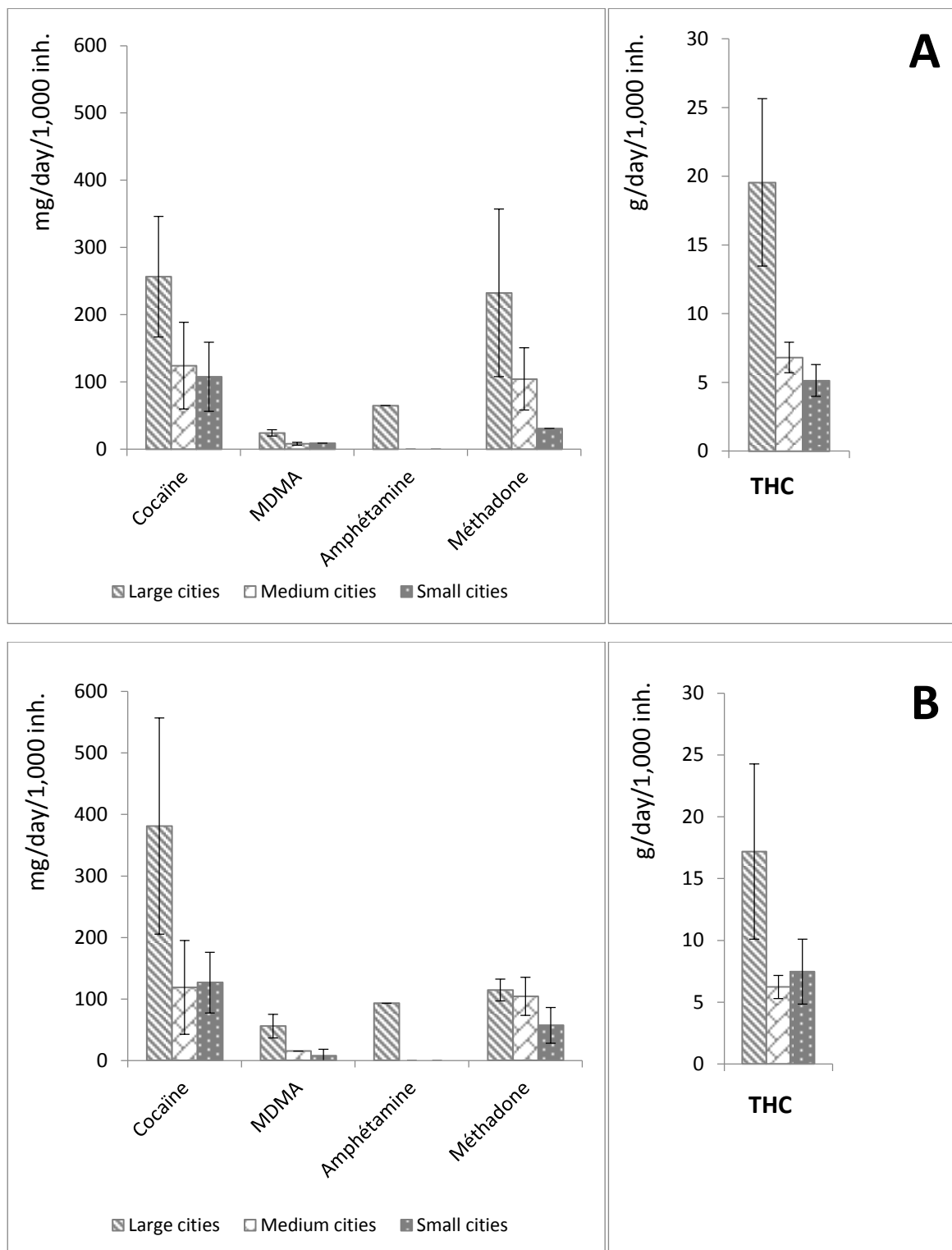
Figure 6: Mean \pm SEM rates of drug consumption depending on the size of cities. A = during week, B = during weekend.
