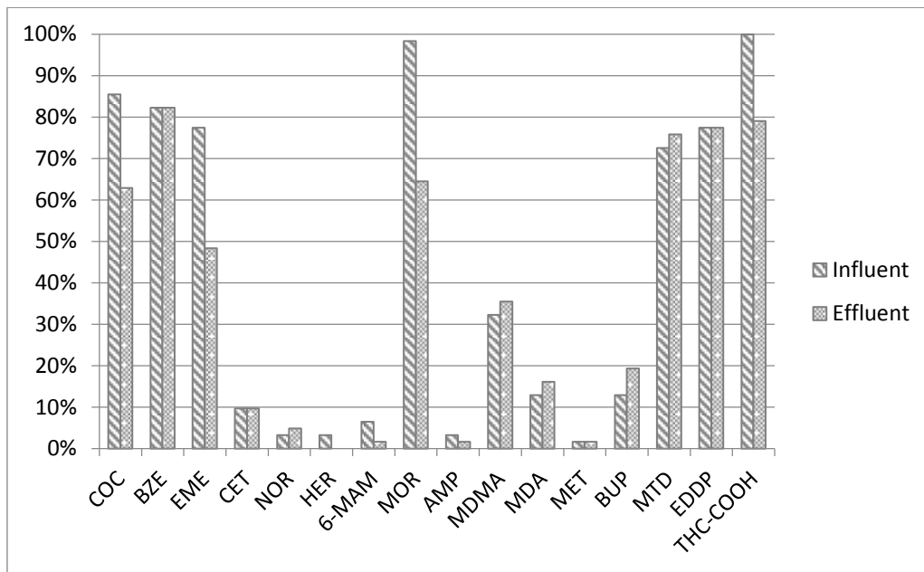
Figure 3 – Frequency of detected analytes in sewage water samples.
