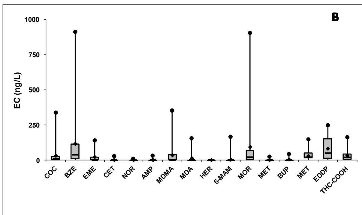
Figure 2 - Box-plot representation of influent (A) and effluent (B) concentrations observed in the 25 STP. For graphic drawing, “no detectable” values have been taken as “0” and “<LOQ” values have been taken as the half of LOQ value for each compound. ♦ mean, — median level.
