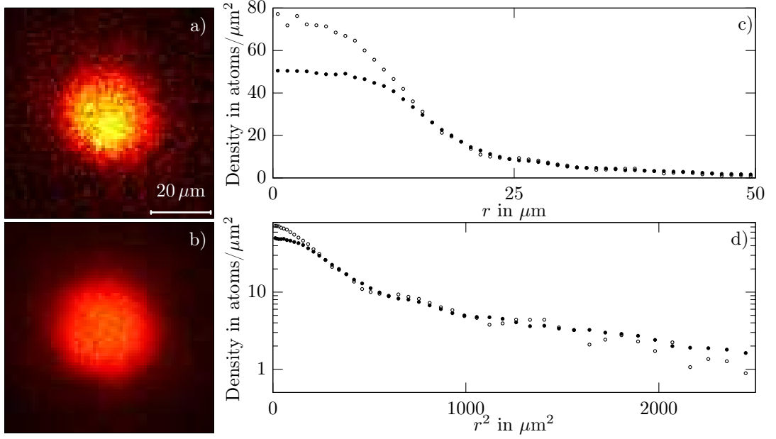
Figure 3.1.: Absorption imaging of quasi-2D clouds of ^{87}\text{Rb} atoms. (a) Image obtained with a short pulse ( \sim 2\ \mu\text{s} ) of an intense probe beam ( I/I_{\text{sat}} = 40 ). (b) Image obtained with a longer pulse ( 50\ \mu\text{s} ) of a weak probe beam ( I/I_{\text{sat}} = 0.5 ). The processing of images (a) and (b) is detailed in the 2.2. (c) and (d) Radial density profiles for image (a) (hollow circles \circ ) and image (b) (filled circles \bullet ) in linear (c) and logarithmic (d) scales. The solid line combines the predictions of the HFMF theory, of [79] in the intermediate regime and of the Thomas–Fermi approximation \mu = \hbar^2 \tilde{g} n / m in the central region ( T = 133\ \text{nK} , \mu/k_B = 47\ \text{nK} ).
