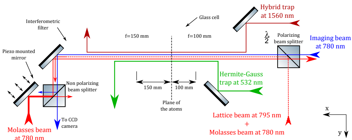
Figure 7.5.: Optical scheme in the xy plane. The hybrid trap and the Hermite-Gauss trap are indicated in dark red and green respectively (see Ch. 2.1). The imaging beam is indicated in blue. The molasses beams and the lattice are indicated in bright red. The two dipole traps are superposed and separated from the other beams with dichroic mirrors, while the lattice beam is retro-reflected on an interferometric filter. A non-polarizing beam splitter must be used to add the second molasses beam orthogonally polarized to the first one.
