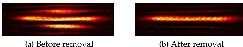
Figure 2.5.: Horizontal absorption images of the atomic distribution, before and after removing atoms in the side wells.
