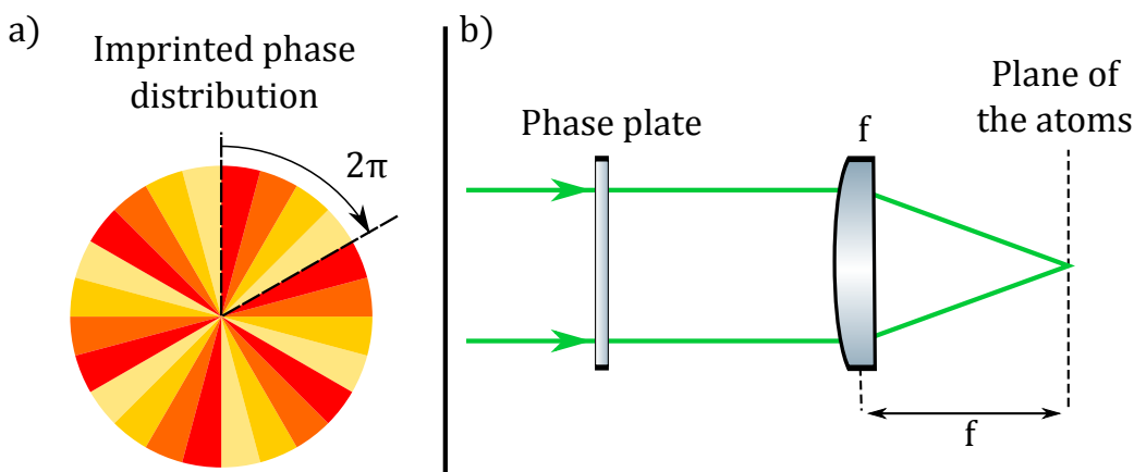
Figure 6.3.: (a) Six-fold phase vortex imprinted by the phase plate. Though only four phase sectors per 2\pi step are represented, our phase plates have 16 sectors per 2\pi step. (b) Experimental setup required to create a stadium with a phase plate.
