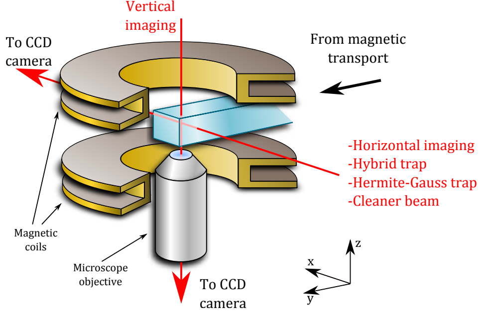
Figure 2.2.: Directions of propagation of the different laser beams used during the sequence.
