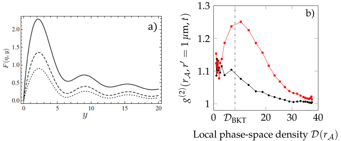
Figure 5.8.: (a) Figure taken from [71]. The function F is directly proportional to \tilde{g}^{(2)}(q, t) , for an argument y = \hbar q^2 t / m . Curves from top to bottom correspond to \eta = 0.25 (solid, the Berezinskii-Kosterlitz-Thouless point), \eta = 0.15 (dashed), and \eta = 0.10 (dotted). (b) Two-body correlation function g^{(2)}(r_{\mathcal{A}}, r' = 1 \mu\text{m}, t = 3 \text{ ms}) , plotted against the local phase-space density, for in-situ images (black circles) and for a 3 ms ToF (red squares).
