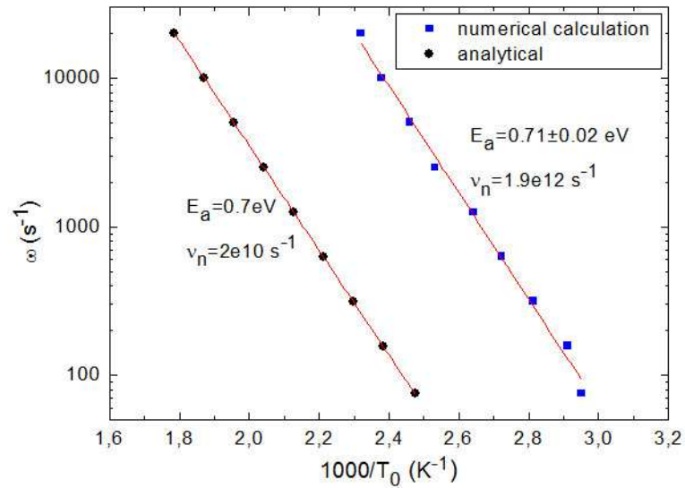
Fig.3.14. Analytically and numerically calculated Arrhenius plot \omega vs 1000/T_0 for E_C - E_F = 0.7 \text{ eV} and N(E_F) = 1 \times 10^{16} \text{ cm}^{-3} \text{ eV}^{-1} .
