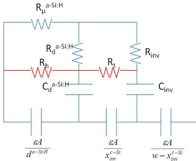
Fig.4.29. Simplified equivalent scheme of a (p) a-Si:H/(n) c-Si heterojunction with tunneling and hopping considered. R_{\mu}^{a-Si:H} is the resistance related to transport, R_d^{a-Si:H} to the time response of the gap states, C_d^{a-Si:H} is the capacitance associated to response of the defects, \epsilon A/L_D^{a-Si:H} . R_{inv} and C_{inv} are the resistance and the capacitance associated to the time response of holes in the strong inversion layer of the width x_{inv} , respectively. R_h and R_t are the resistances associated with tunneling and hopping, respectively.
