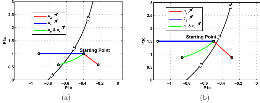
Figure 4.6: Variation of control gains c_1 and c_2 to turn the (a) unstable, (b) stable, dynamical system (represented by starting point P) into (a) a stable, (b) an unstable system for A_c = 1.5 .
