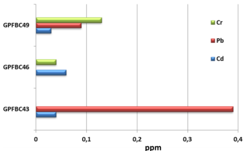
GPFBC43 – 45 REFIOm/45 MIOM/10 Calcin ; GPFBC46 - 40 REFIOm/40 MIOM/20 Calcin ; GPFBC49 - 35 REFIOm/35 MIOM/30 Calcin ; L/S= 1,2 ; séchage T ambiante
