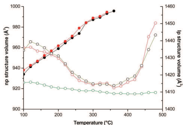
Fig. 8 Evolution of the pore volume of the np and lp phases as a function of temperature. Key: np structure (filled circles) and lp structure (empty circles). Samples (A) (green), B (black) and C (red).
