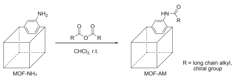
Figure 21. Post-modification of NH 2 -BDC-based MOF through amide coupling to give the amido-functionalized MOF-AM.
