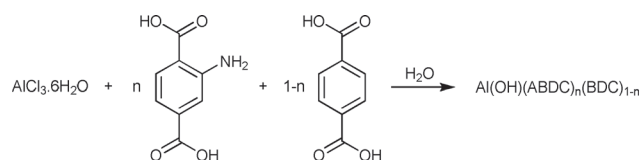
Fig. 1 Synthesis of Al-MIL-53 with different amino contents.
