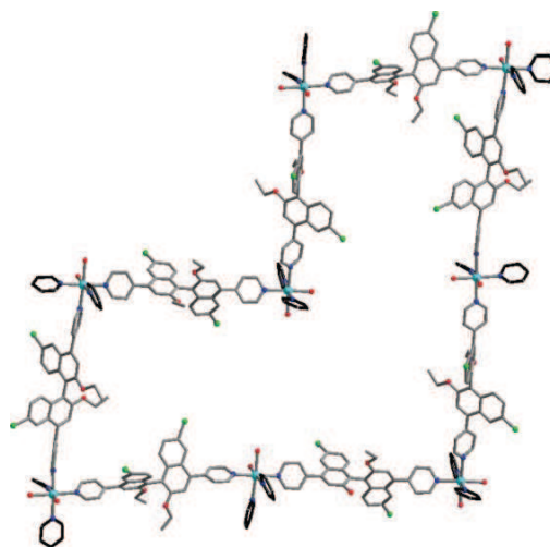
Figure 19. formation of octagons from linking the cis -[Cd(Py) 4 (H 2 O) 2 ] nodes. The Py rings shown in black link the octagon to other polygons 108 .
