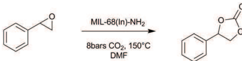
Scheme 30. Synthesis of styrene carbonate from styrene oxide
