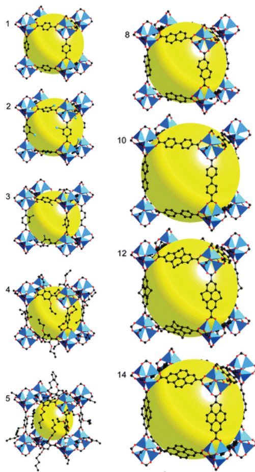
Figure 10. Example of 3D isoreticular compounds (IRMOFs)
