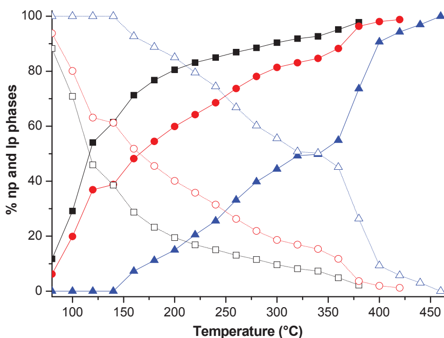
Figure 10. Evolution of the np (empty symbols)-lp (filled symbols) phase ratio as a function of temperature for B (square), C (circle) and D (triangle) samples.
