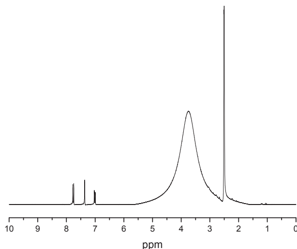
Figure 21. Liquid ^1\text{H} NMR spectra of MIL-68(In)-NH 2 .
