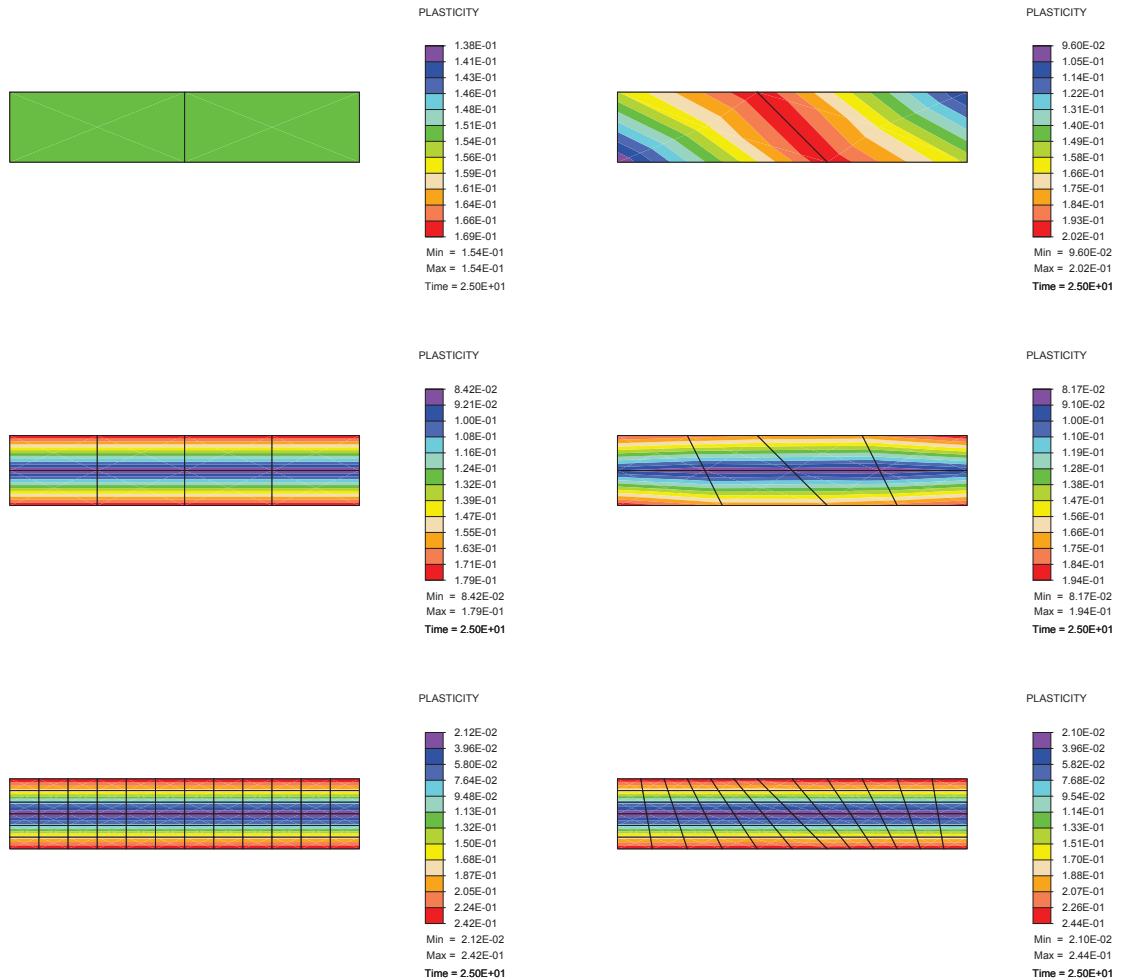
Figure 4.14: Yield contour of plasticity behavior q^P due to imposed bending loading for distorted and undistorted meshes.
