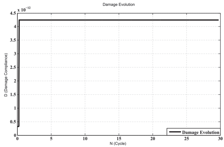
Figure 4.12: Damage Evolution during the loading process in Figure 4.9.
