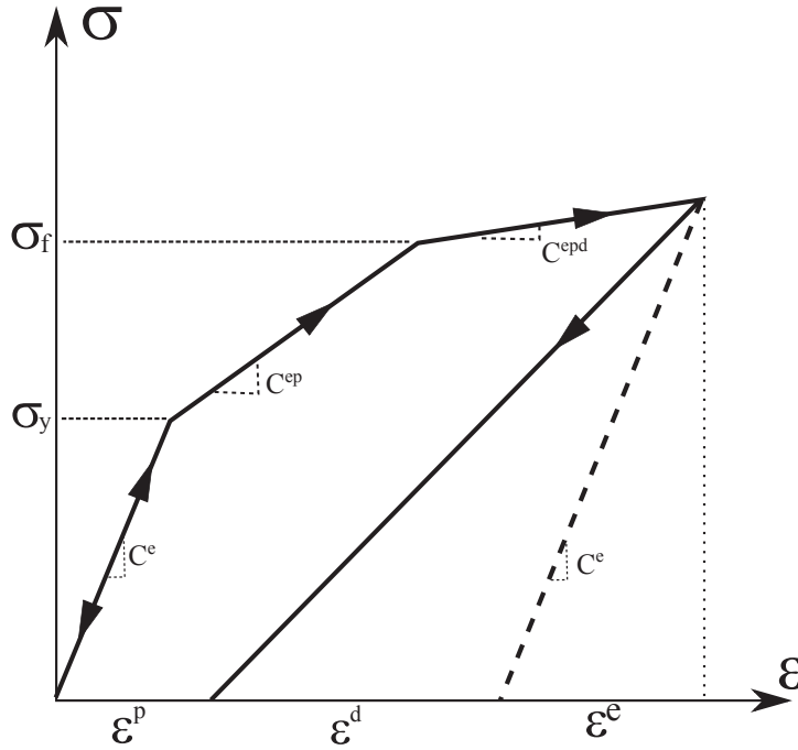
Figure 3.2: Stress-strain diagram for the coupled damage-plasticity model.
