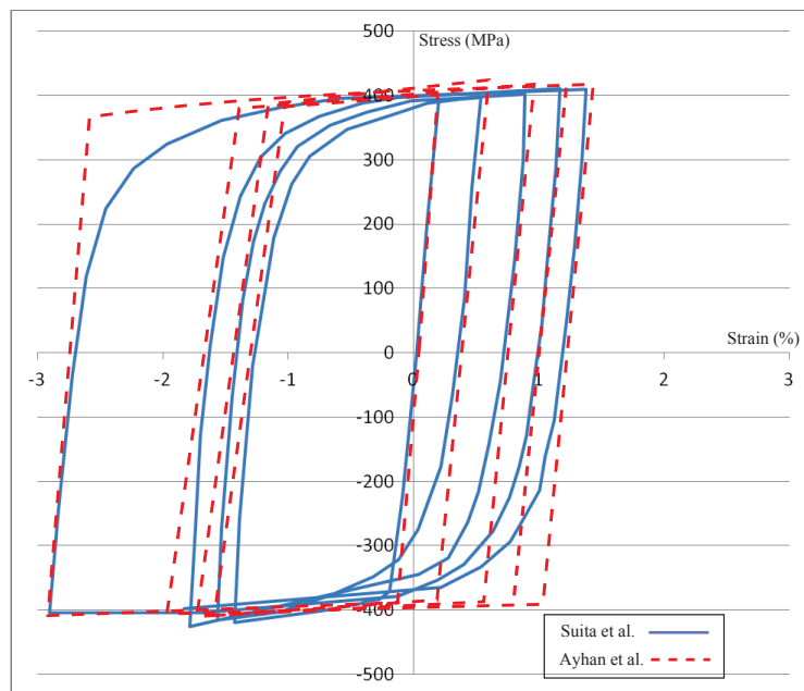
Figure 4.3: Cyclic test on a rectangular member (100*50 cm).
