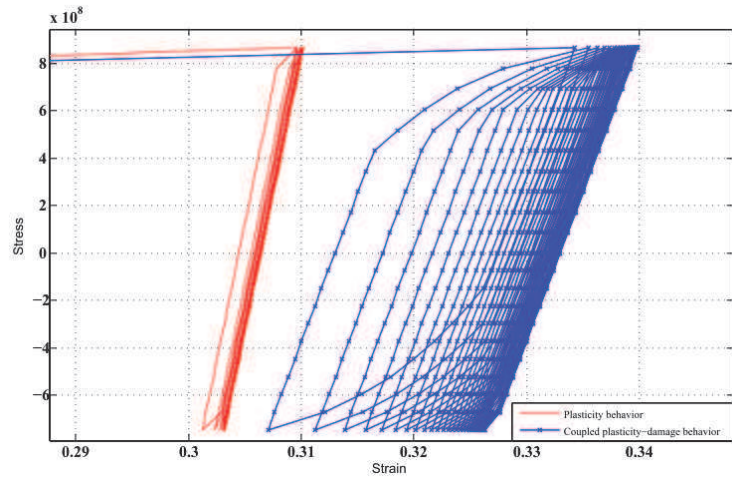
Figure 4.11: Ratcheting behavior of the material due to imposed forces.
