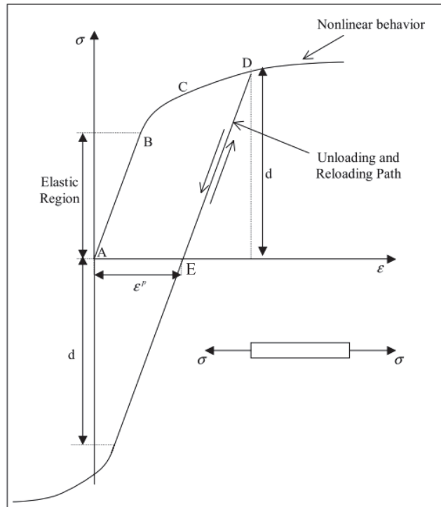
Figure 2.2: Stress-Strain curve for uniaxial loading.
