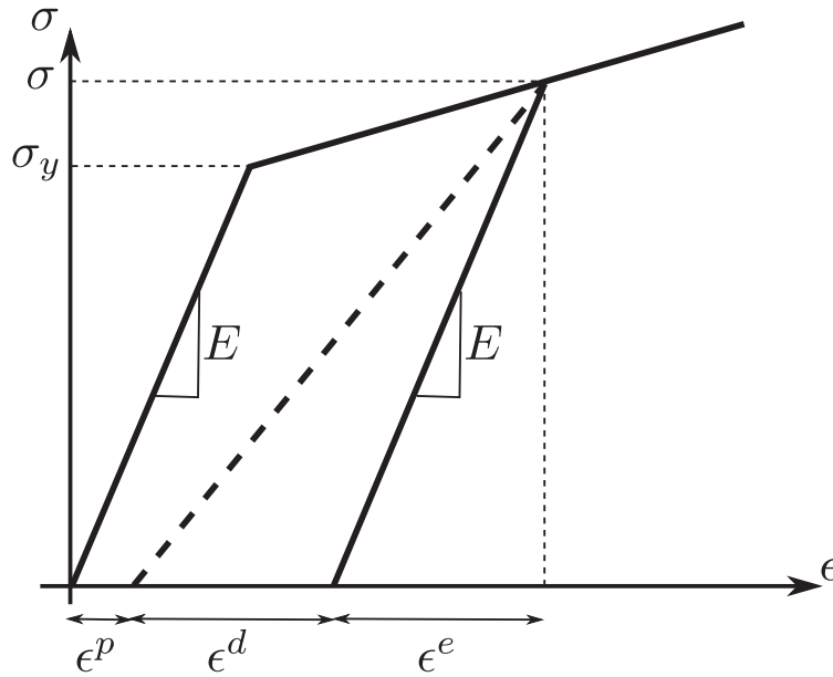
Figure 3.1: Schematic representation of the involved strains for a 1D model.
