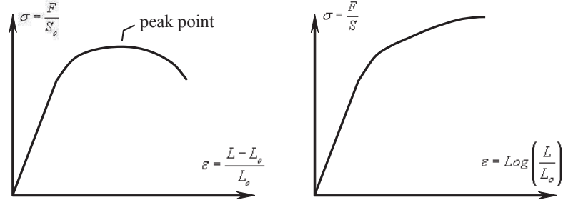
Figure 2.1: Curves in tension, ductile material. At left side, conventional ( nominal) curve At right side rational (real) curve.
