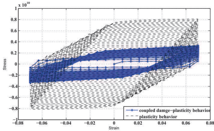
Figure 4.5: Strain-stress diagrams for both proposed coupled damage-plasticity model and plasticity alone.
