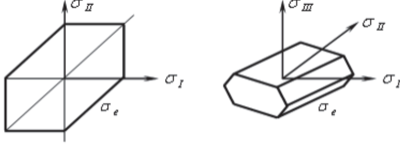
Figure 2.7: Representation of the plasticity surface defined by the Tresca criterion.
