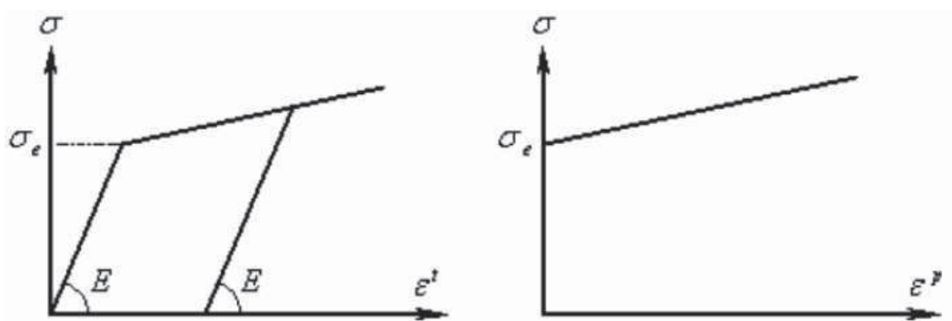
Figure 2.3: Model of elastoplastic behavior.
