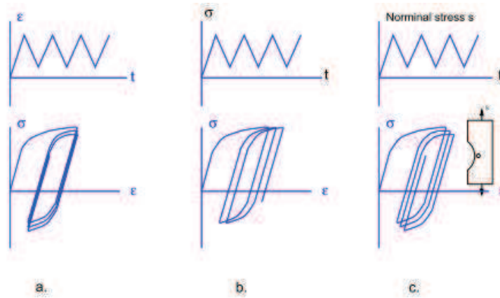
Figure 1.1: Cyclic behavior models.
