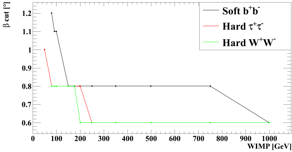
Figure 6.37: Optimal \beta [°] cuts as a function of WIMP mass and annihilation channel.
