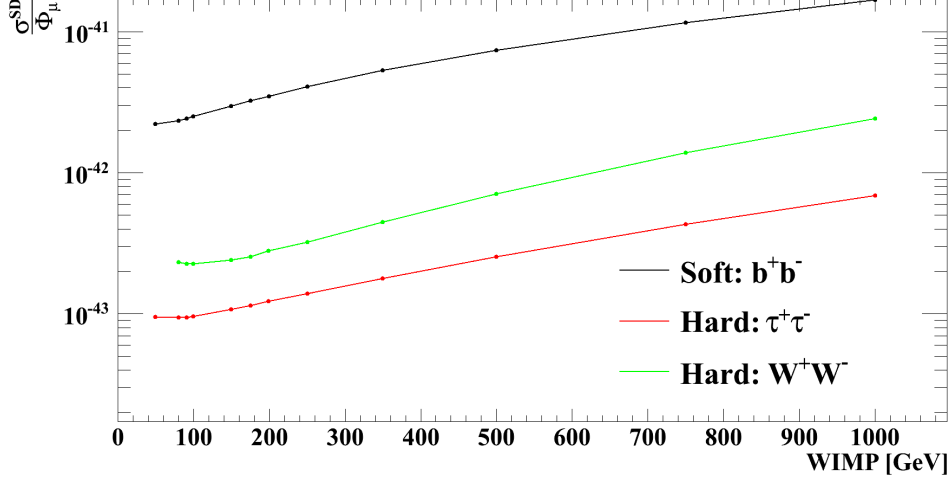
Figure 2.17: Conversion factor from muon flux [ \text{km}^{-2}[\text{year}^{-1}] ] to spin-dependent cross-section [ \text{pb} ] as a function of the annihilation channel and WIMP mass.
