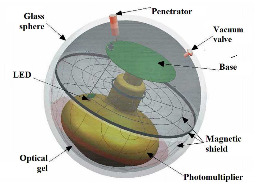
Figure 3.12: ANTARES Optical Module
