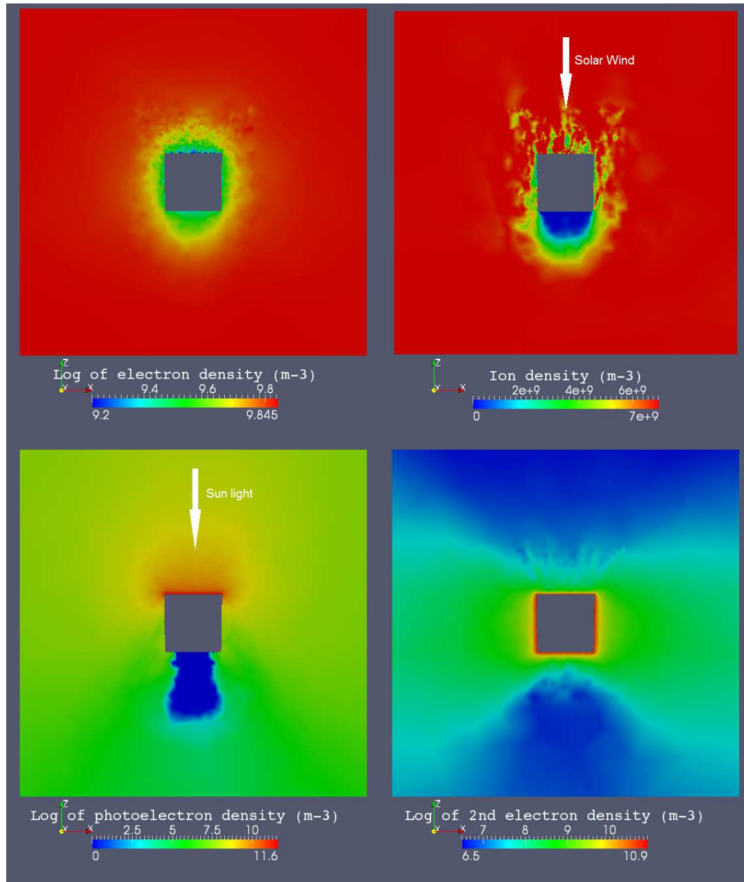
Figure 4.14: Simulation S1 population density maps in the X - Z plane: (a-d) from the upper left figure to the lower right figure. (a) Thermal electrons, (b) Ions, (c) Photoelectrons, (d) Secondary electrons.
