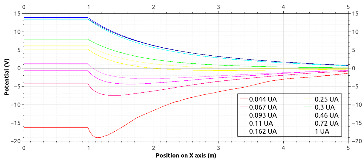
Figure 4.23: Plasma potential along the X axis for all simulations. The spacecraft potential is monotonically increasing with heliocentric distance.
