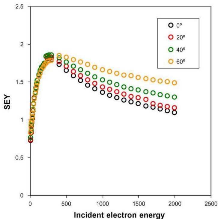
Figure 3.10: SEY: Effect of the incidence angle on the SEY of a smooth Cr surface (roughness R_a = 3 ). From [Balcon et al. (2012)].
