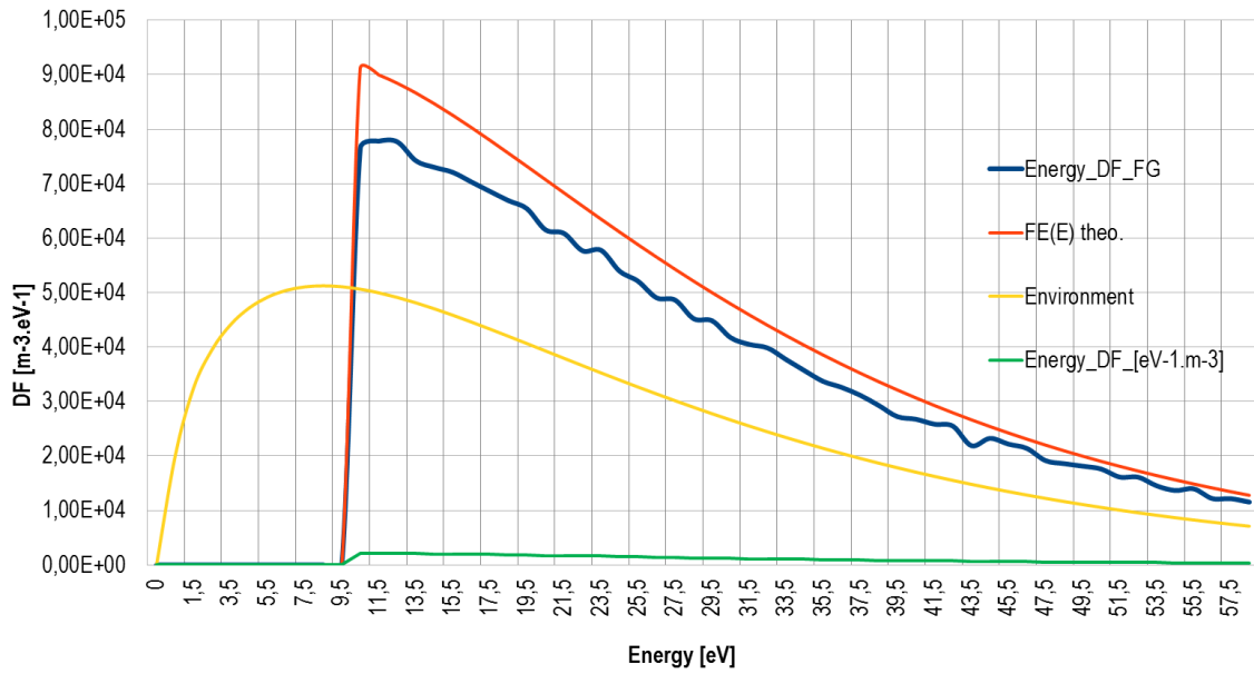
Figure 6.72: CLUS@1 AU - Energy distribution functions of thermal electrons on LEEA.
