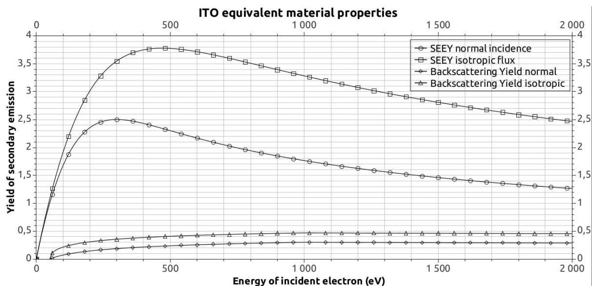
Figure 4.12: Secondary electron emission yield (SEY) and the backscattering yield of ITO material (used in parametric study) vs. incident electron energy (with a normal or isotropic incident flux).
