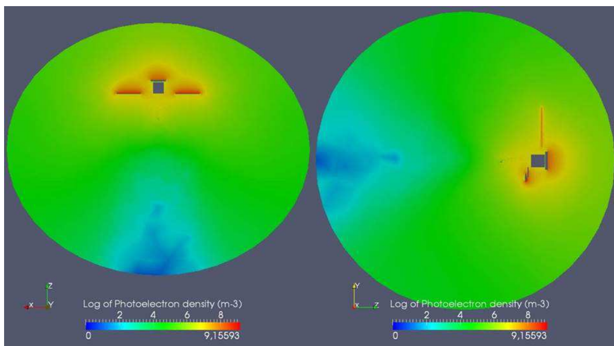
Figure 6.18: SOLO@1 AU - Log of photoelectron density (left: X - Z plane, right: Y - Z plane).
