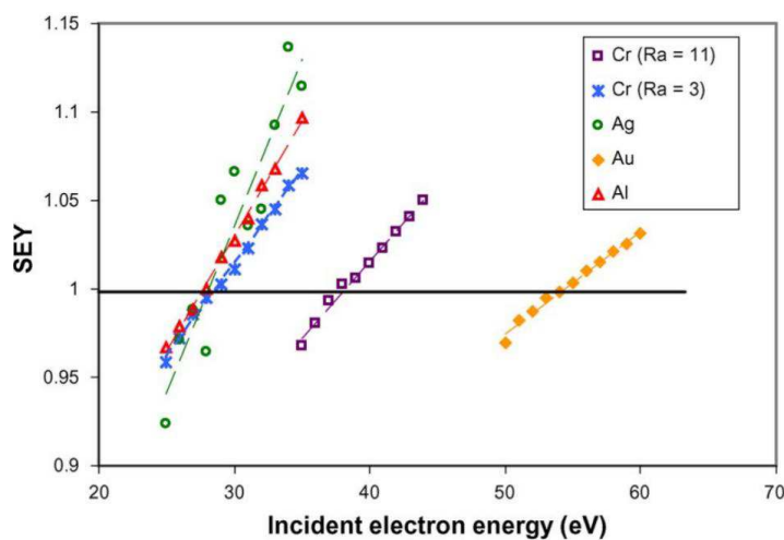
Figure 3.9: SEY of Al, Au, Ag, and Cr as a function of the incident electron energy near the first crossover energy. R_a stands for the roughness of the material (a material less polished than others will present more bumps on its surface and will be considered as rough). From [Balcon et al. (2012)].
