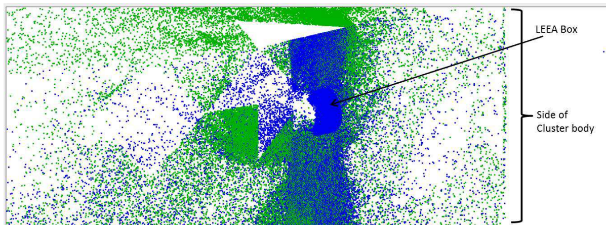
Figure 6.76: CLUS@1 AU - Origin of detected SSEE (green dots) and photoelectrons (blue dots) – Focus on LEEA area.
