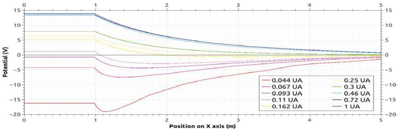
Fig. 6. Plasma potential along X axis for all simulations (the heliocentric distance is monotonically increasing with spacecraft potential).
