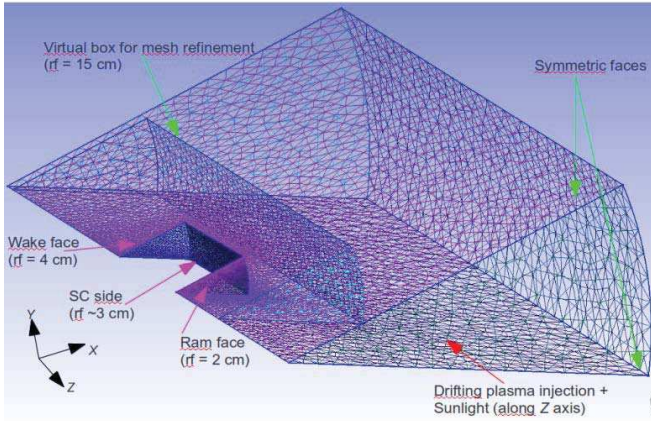
Fig. 1. Geometry cut model of the cylinder (covered with ITO material) and the simulation box + the associated mesh (“rf” = mesh refinement).
