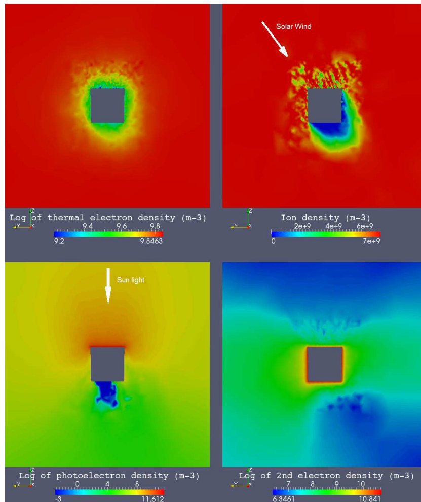
Fig. 18. Simulation S5 population density maps: (a–d) from the upper left figure to the lower right figure. (a) Thermal electrons, (b) Ions, (c) Photoelectrons, (d) Secondary electrons.
