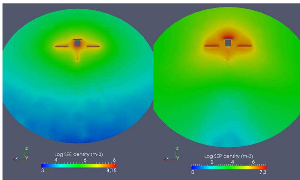
Figure 6.34: SOLO@1 AU-FW - Log of SSEE density (left) and SEEP (right).
