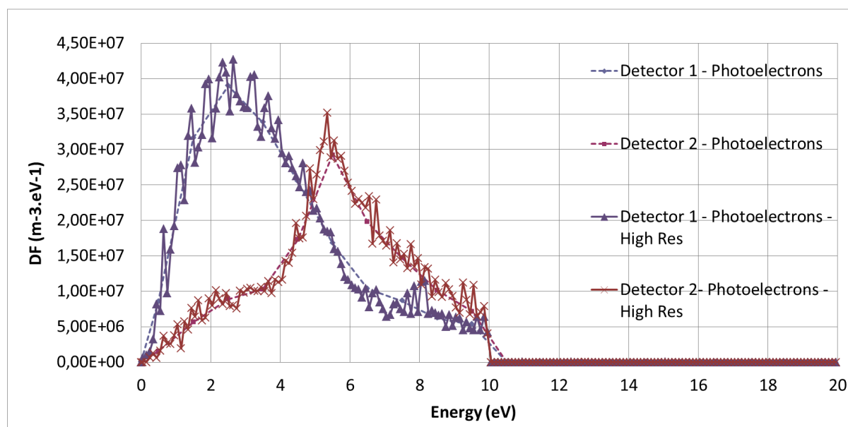
Figure 5.23: Case 5: measured energy distribution functions of photoelectrons. Dashed lines: low energy resolution of 1 eV. Full lines: high energy resolution of 0.1 eV.
