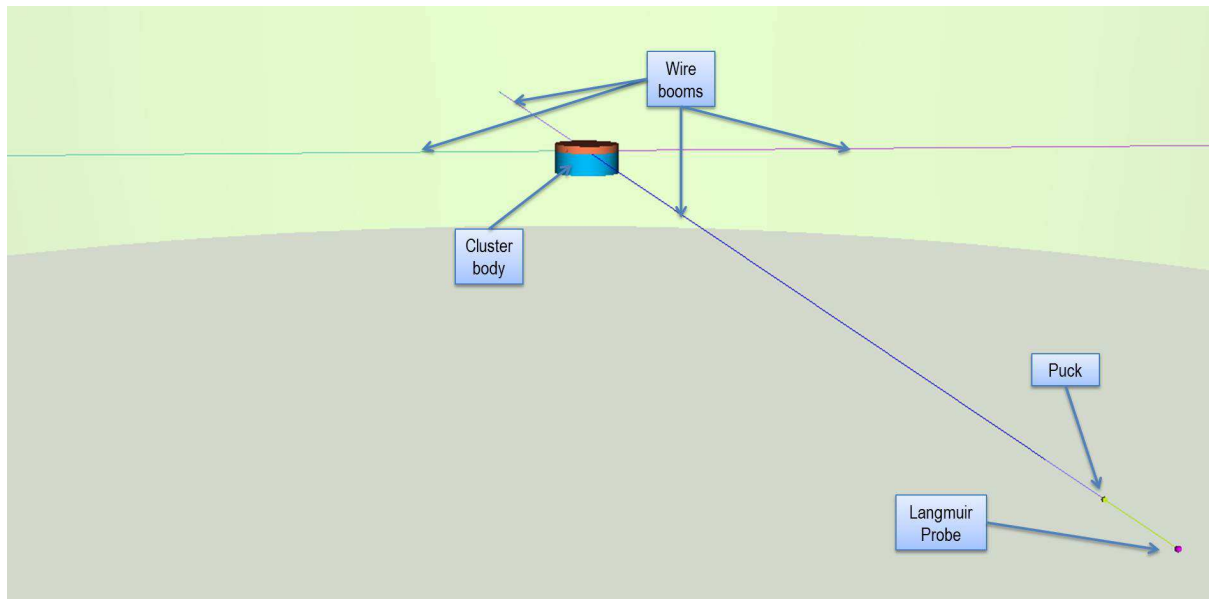
Figure 6.54: GMSH model - Cluster geometry, plain view.
