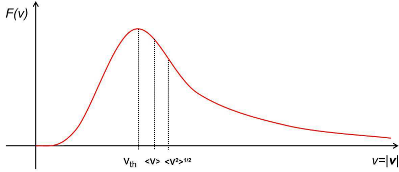
Figure 2.1: Plot of equation 2.8 illustrating the aspect of the Maxwellian distribution function. The thermal, mean and root mean square velocities are identified on the abscissa axis
