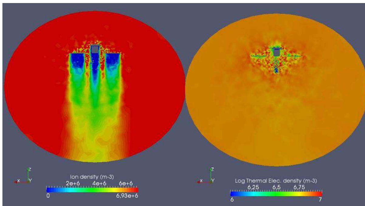
Figure 6.17: SOLO@1 AU - Ions and thermal electrons density (in the X - Z plane).
