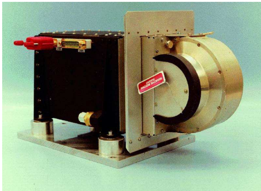
Figure 6.58: Photography of PEACE-LEEAA ( source : Mullard Space Science Laboratory).
