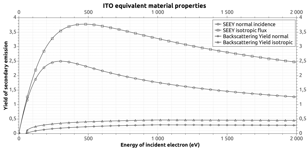
Fig. 10. Secondary electron emission yield (SEEE) and the backscattering yield of ITO material (used in parametric study) vs. incident electron energy (with a normal or isotropic incoming flux).
