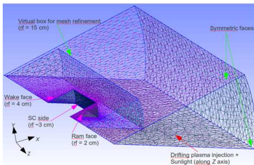
Figure 4.19: Geometry cut model of the cylinder (covered with ITO material) and the simulation box + the associated mesh ("rf" = mesh refinement).
