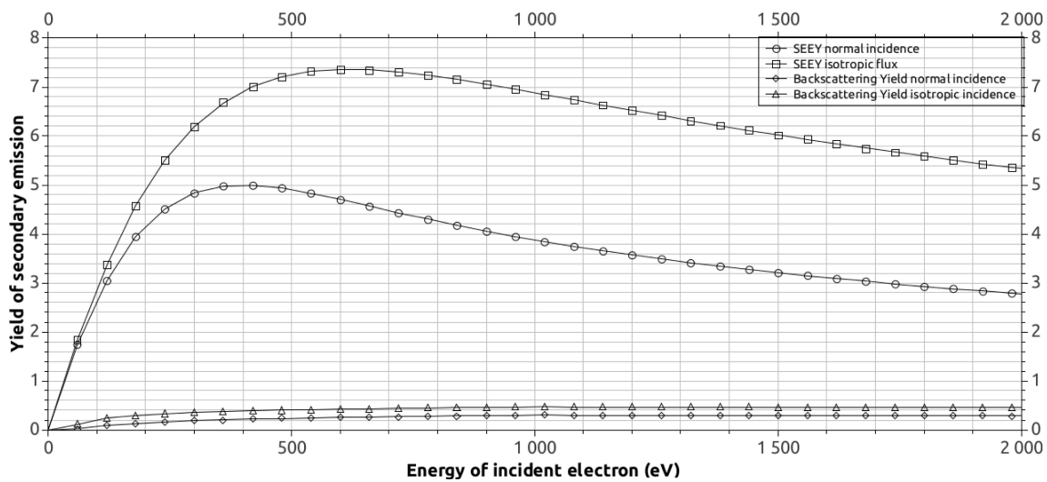
Fig. 2. Cross comparison simulation B (SPIS): Secondary Electron Emission Yield (SEY) and the backscattering yield vs. incident electron energy (with a normal or isotropic incoming flux).
