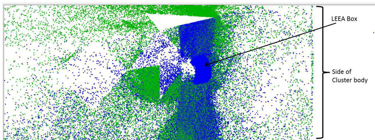
Figure 6.76: CLUS@1 AU - Origin of detected SSEE (green dots) and photoelectrons (blue dots) - Focus on LEAA area.
