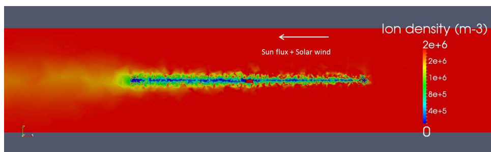
Figure 6.67: CLUS@1 AU – Ion density around Cluster in the Z - X plane.
