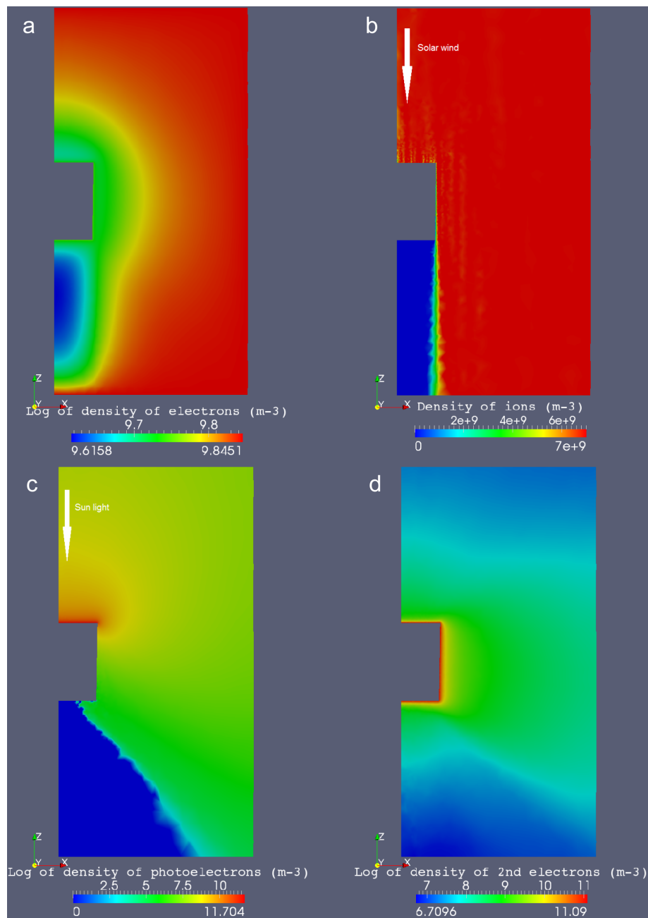
Fig. 8. Cross comparison simulation B (SPIS): population density maps ( T_{ph} = 3 eV): (a–d) from the upper left figure to the lower right figure. (a) Thermal electrons, (b) Ions, (c) Photoelectrons, (d) Secondary electrons.
