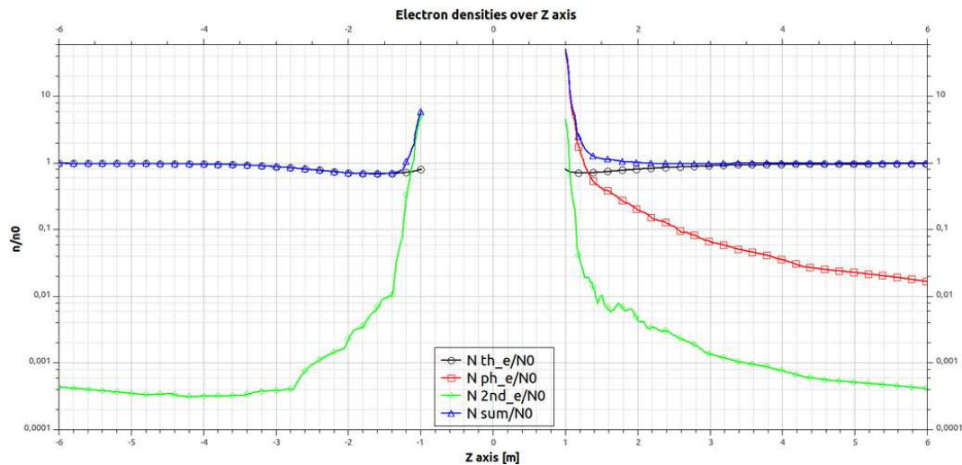
Fig. 15. Simulation S2: plot along the z-axis of electrons over n_0 , the plasma density: 7 \times 10^9 \text{ m}^{-3} .
