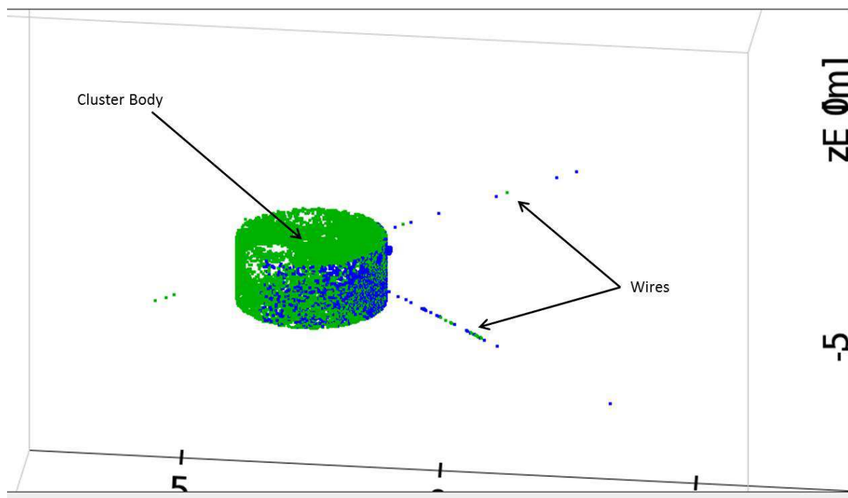
Figure 6.75: CLUS@1 AU - Origin of detected secondary electrons (green dots) and photoelectrons (blue dots) by LEAA.
