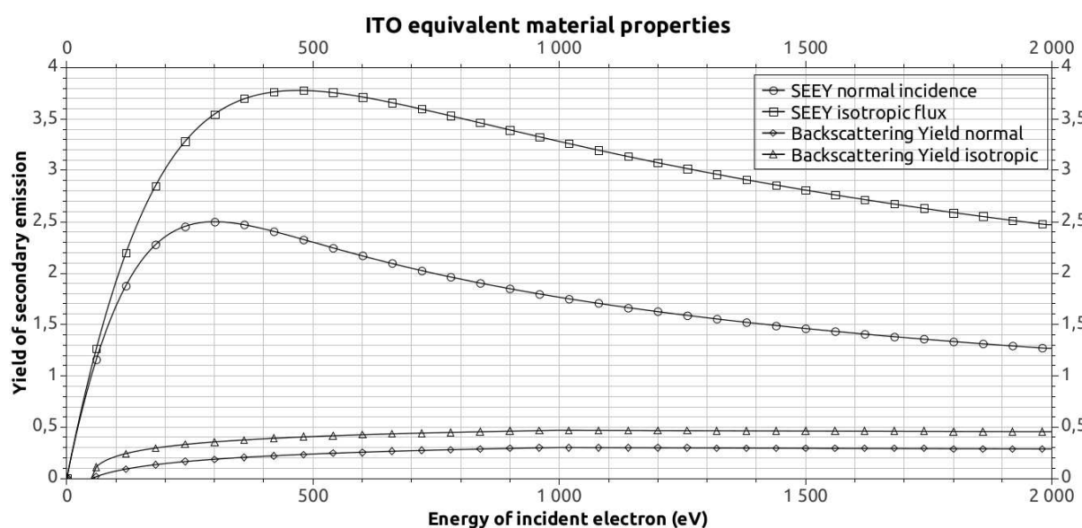
Figure 4.12: Secondary electron emission yield (SEAY) and the backscattering yield of ITO material (used in parametric study) vs. incident electron energy (with a normal or isotropic incident flux).
