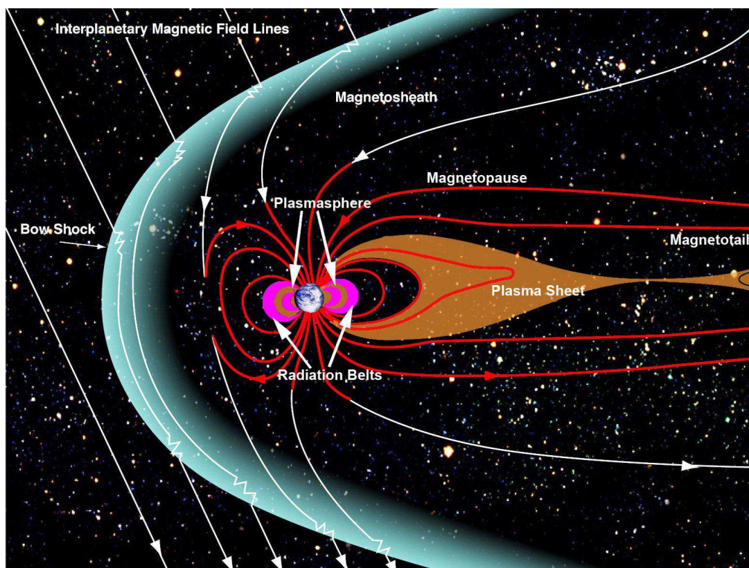
Figure 2.10: Main components of the Earth magnetosphere structure ( Original bitmap from NASA )
