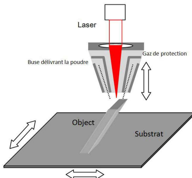
Figure I.12. Schéma illustrant la technologie Laser Engineered Net Shaping [49]
