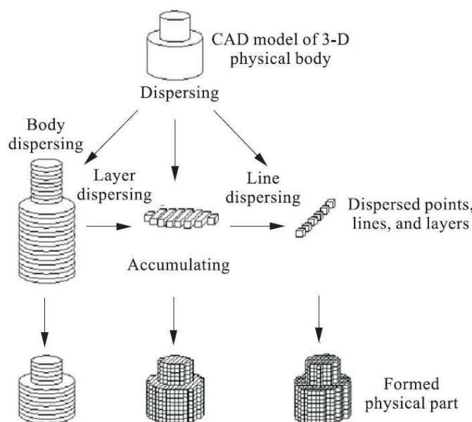
Figure I.4. Illustration du principe de la fabrication additive [21]
