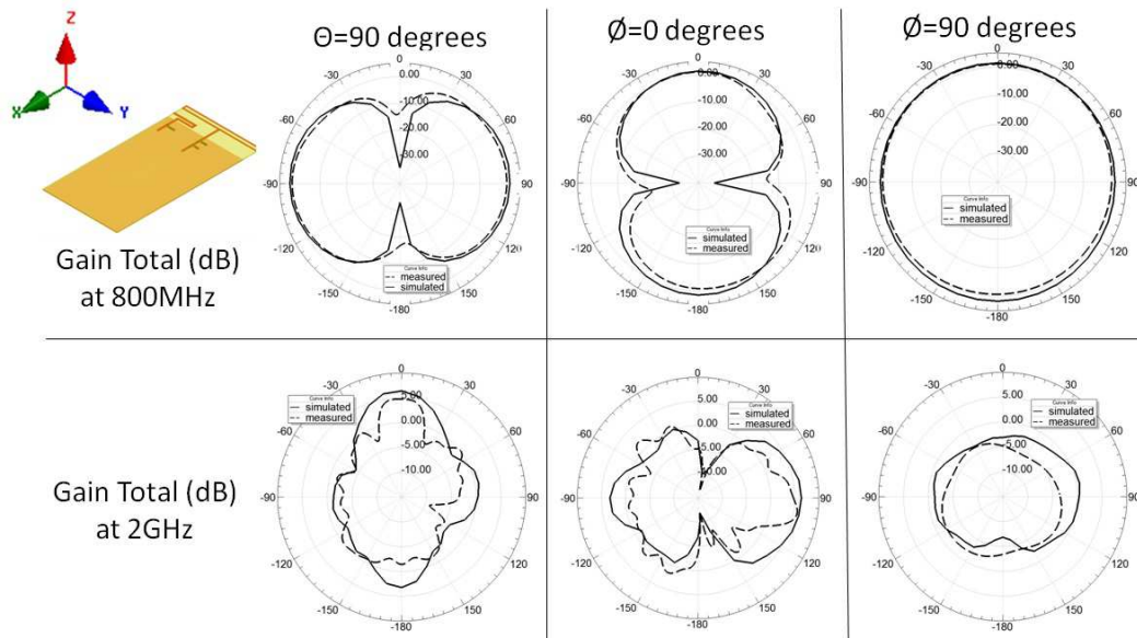
Figure 93 Simulated and Measured Total Gain Patterns for Different Cut Planes
