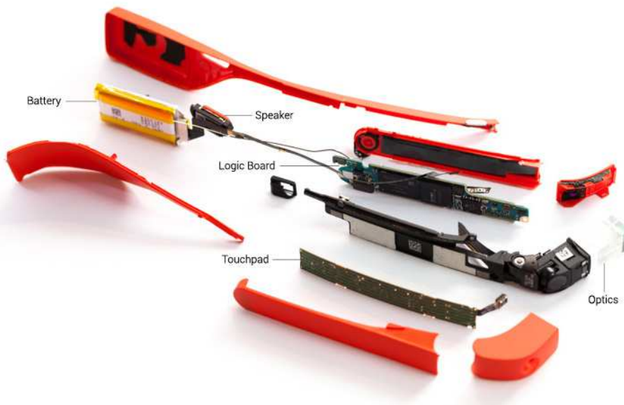
Figure 144 Teardown of the Google Glass
