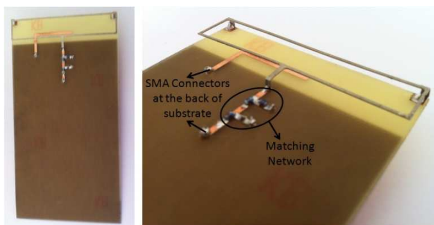
Figure 76 Manufactured Prototype of the Hollow CE Antenna
