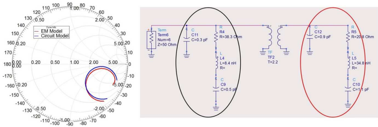
Figure 29 Circuit Model of the Combination of Driven and Parasitic Strips
