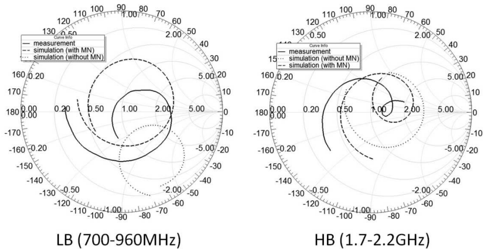
Figure 10 Simulated and Measured Input Impedance for UMTS Antenna, with/without MN
