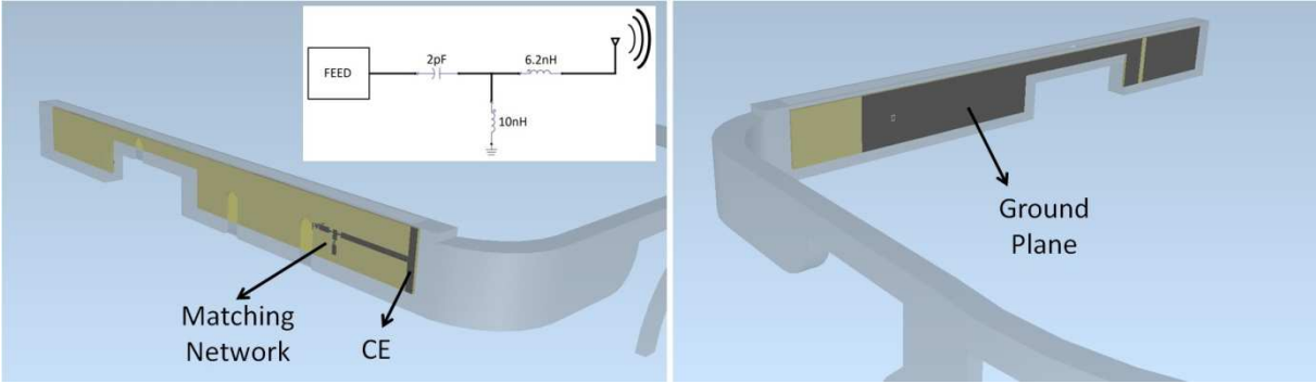
Figure 167 Eyewear-Antenna-2 Model
