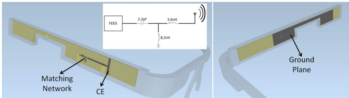
Figure 173 Eyewear-Antenna-3 Model
