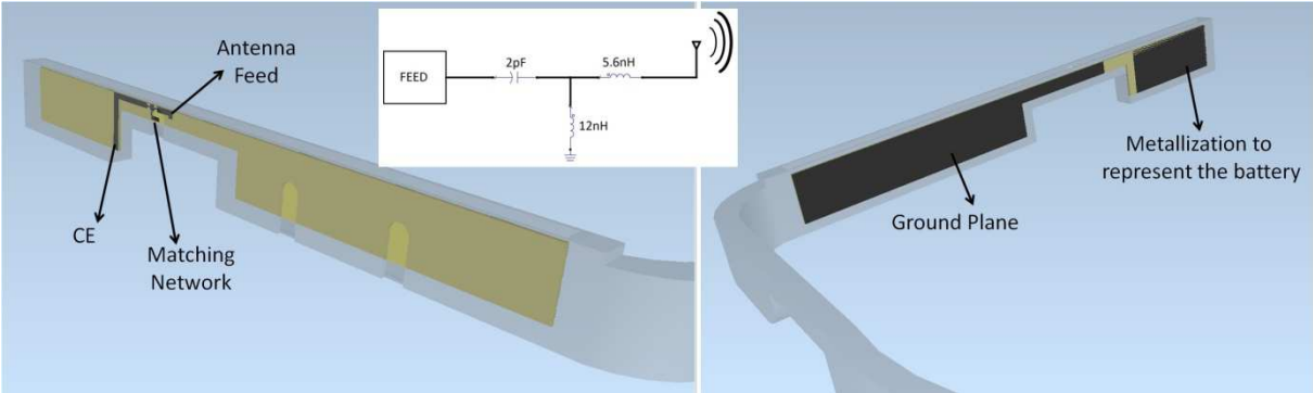
Figure 160 Eyewear-Antenna-1 Model
