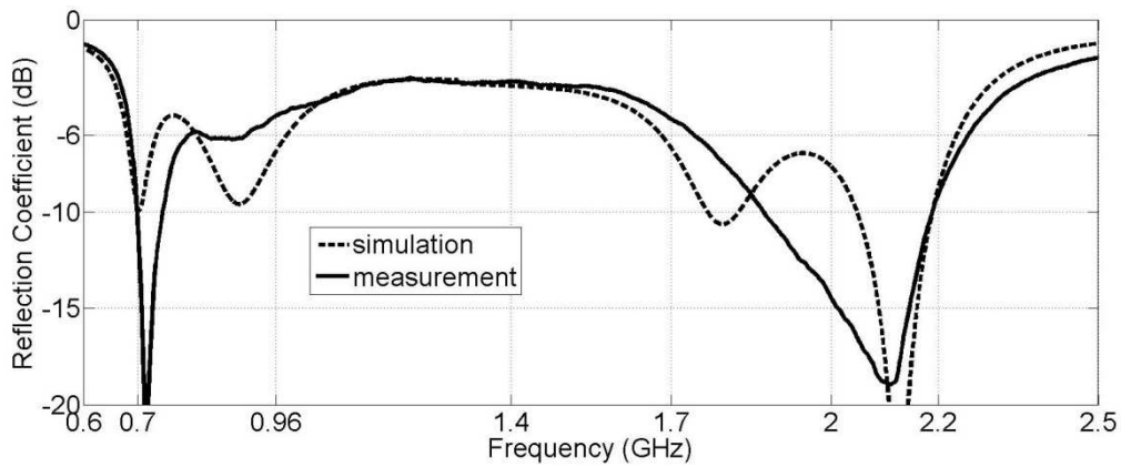
Figure 11 Simulated and Measured Reflection Coefficient for the UMTS Antenna
