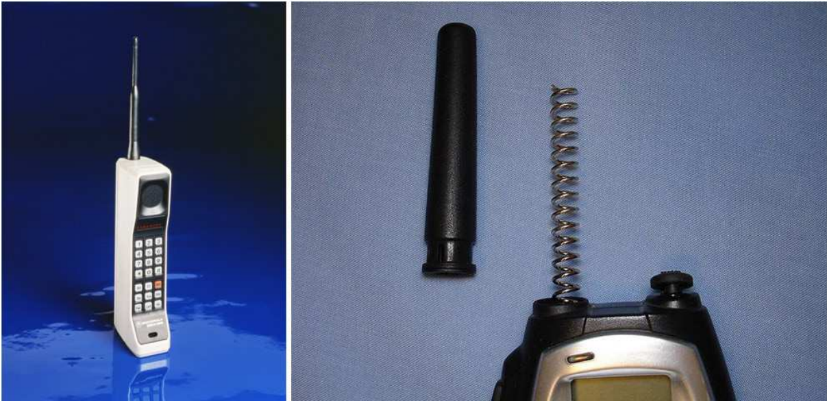
Figure 3 Examples of External Antenna for Mobile Phones
