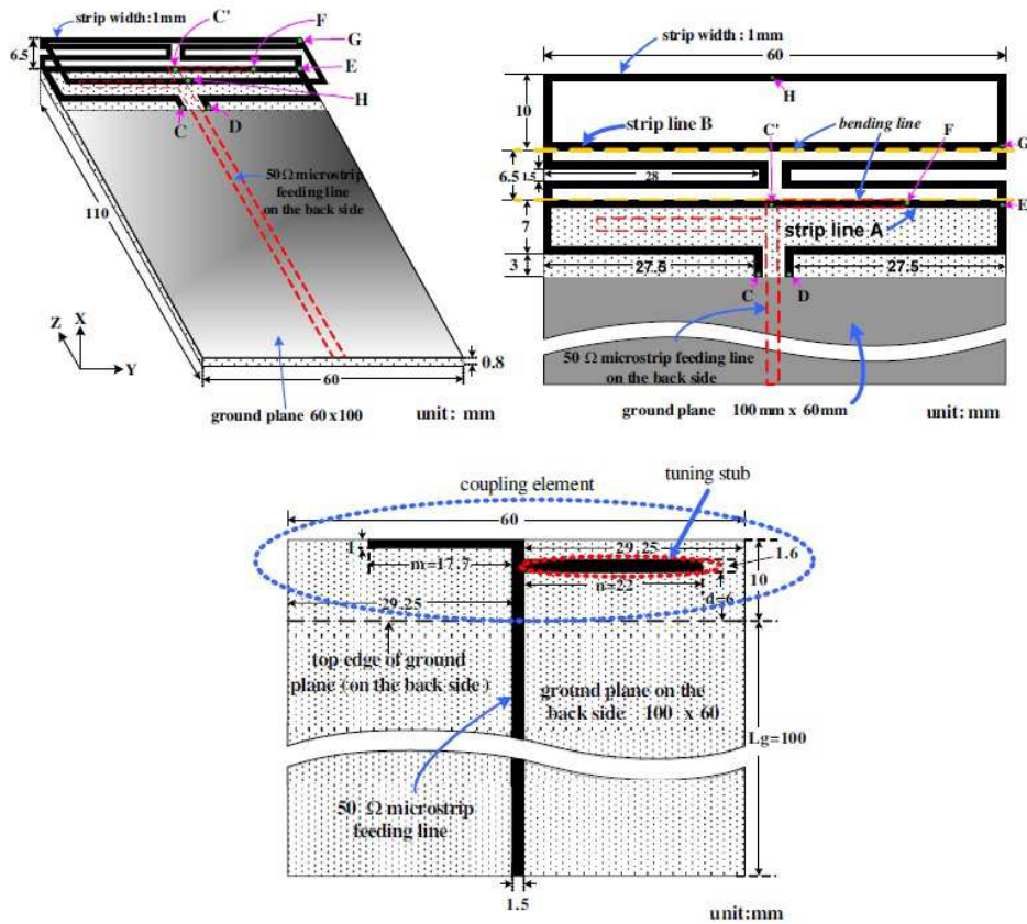
Figure 17 Meandered Loop Antenna in [32]
