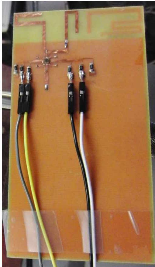
Figure 46 Manufactured Prototype for Antenna Design II
