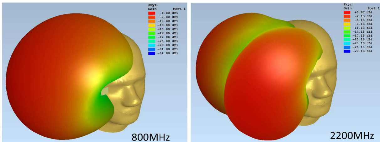
Figure 152 3D Gain Pattern for Position 2
