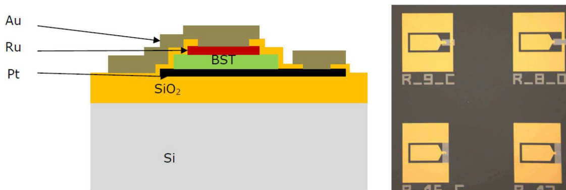
Figure 57 Layout of a BST Capacitor and Photograph of Manufactured Dies
