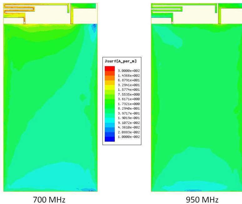
Figure 26 Surface Currents of the Antenna and The Chassis in LB
