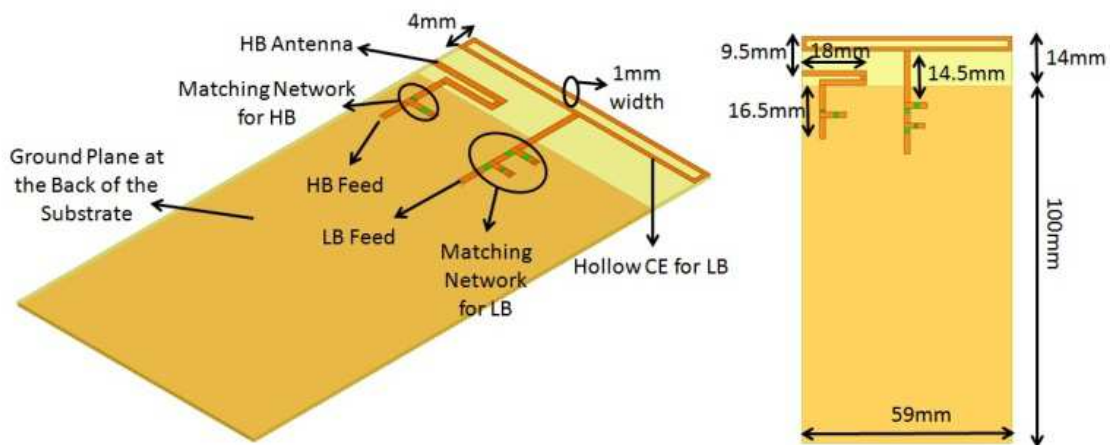
Figure 80 Simulation Model of the Printed CE Antenna
