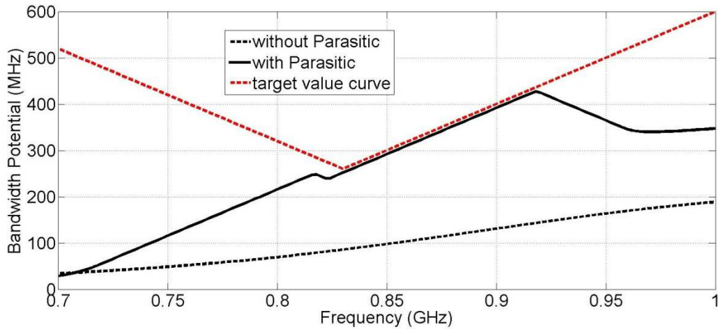
Figure 27 Comparison of BW Potential of the antenna With/Without Parasitic Element
