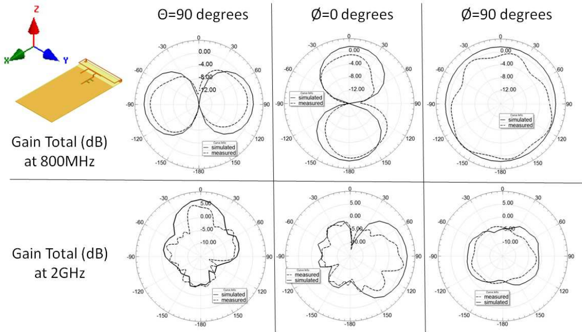
Figure 79 Simulated and Measured Total Gain Patterns for Different Cut Planes
