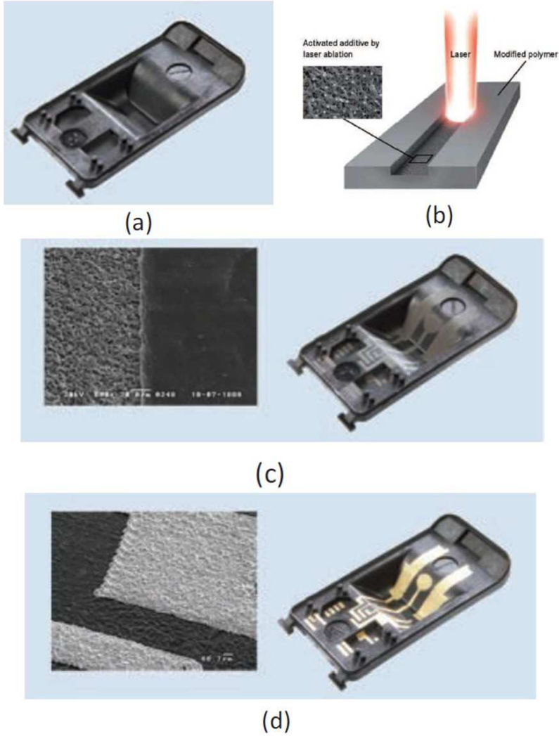
Figure 105 LDS Manufacturing Process
