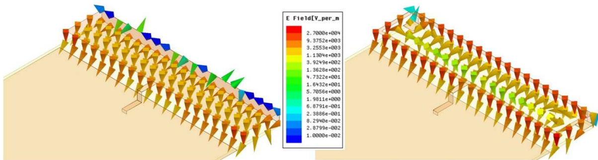
Figure 68 Comparison of the E-field Under the CEs (Plain CE on left, Hollow CE on right)
