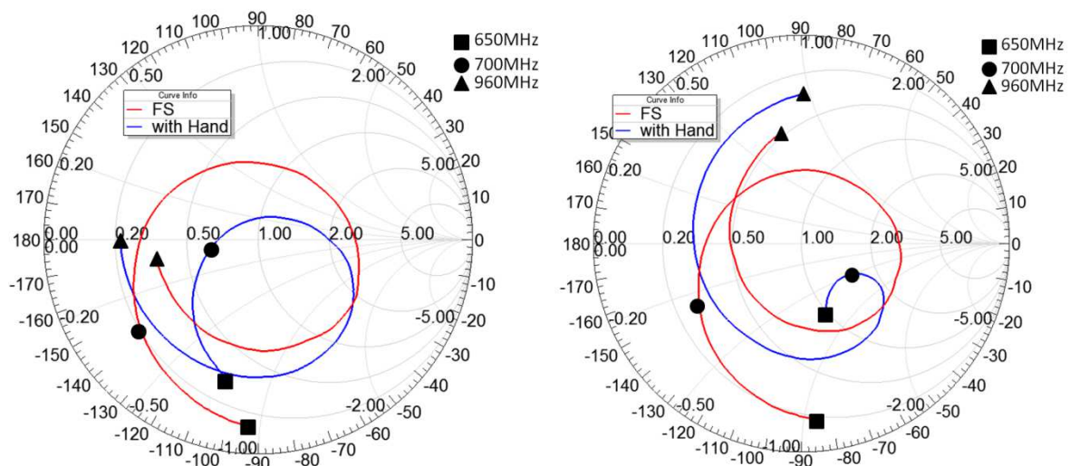
Figure 131 Measured Input Impedance of Hollow CE Antennas in FS and with Hand
