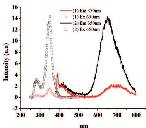
Fig. 10 Excitation and emission spectra of (1) and (2) in solution in dmf ( 3.1 \times 10^{-6} \text{ M} ) at room temperature and aerobic condition. The fine peak at 392 nm on emission spectra of (1) and (2) is attributed to Raman resonance of solvent.
