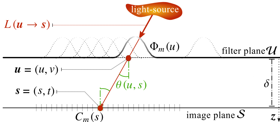
Figure 4.2: Original rendering model for the two-plane setup (cf. Section 2.7.3).
