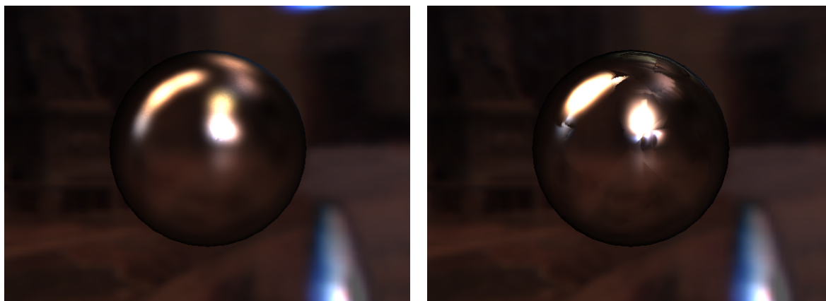
Halton Sequence
