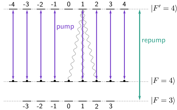
FIGURE 2.10 : Principle of optical pumping into m_F = 0 . A \pi -polarized pump field is applied in order to transfer all the atoms into |F = 4, m_F = 0\rangle , which is a dark-state due to the nullity of the |F, m_F = 0\rangle \rightarrow |F' = F, m'_F = 0\rangle coefficient. If atoms fall in |F = 3\rangle the repump field bring them back into the pumping cycle. The number of levels is however an issue as many cycles are required, leading to a heating of the atoms.
