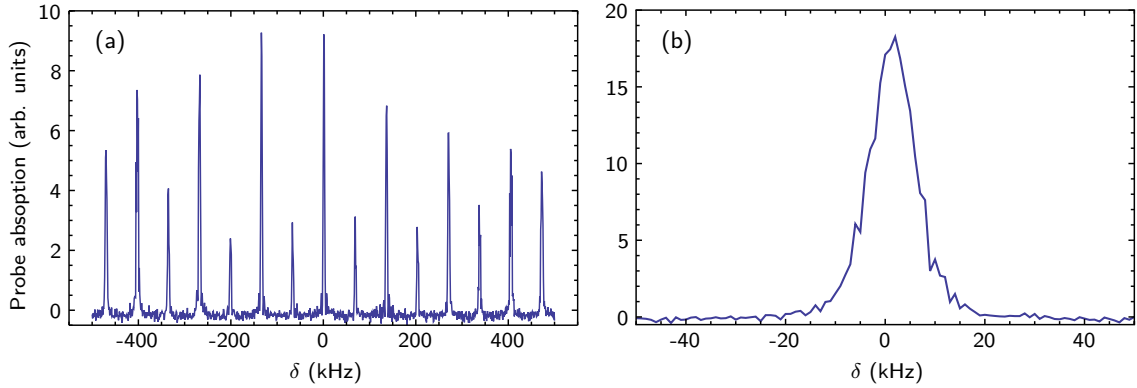
FIGURE 2.9 : Microwave spectroscopy measurement. The absorption of the probe pulse is represented as a function of the microwave pump detuning \delta (a) when applying a DC magnetic field to split the different levels, or (b) after optimization of the compensation coil currents in order to cancel the spurious magnetic field. Typical widths around 20 kHz are routinely obtained.
