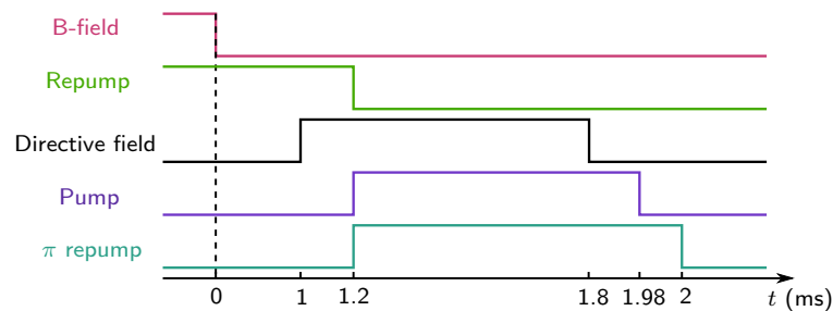
FIGURE 2.13 : Timing of the optical pumping sequence. Pump and repump beams are applied during 800 \mu\text{s} before the memory sequence, while a directive magnetic field defines the quantization axis. For clarity, the scale of the time axis is not respected.
