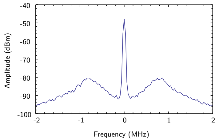
FIGURE A.2 : Beating observed at the spectrum analyzer. Sidebands are observed at 800 kHz around the central peak.
