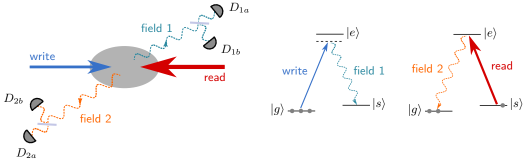
FIGURE 5.1 : DLCZ building block and detection setup for the determination of correlation and autocorrelation functions. A weak write pulse induces a spontaneous Raman transition into field 1. This mode is split by a 50/50 beam splitter and detected by a pair of single-photon counters, D_{1a} and D_{1b} . After a user-defined delay, a strong read pulse enables the transfer of the atomic collective excitation into a photonic mode, called field 2, also detected by a set of two single-photon counters, D_{2a} and D_{2b} .
