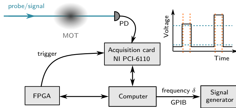
FIGURE B.1 : Principle of Labview managed spectroscopy. Probe or signal pulses are detected by a photodiode, and its output is recorded by an acquisition card and transferred to the computer where it is analyzed with Labview, by setting horizontal or vertical thresholds. The computer communicates also via Labview with the FPGA (Field-programmable gate array), which triggers the acquisition and the shaping of the optical pulses. Finally, the Labview program on the computer commands the frequency detuning \delta to a signal generator via GPIB.
