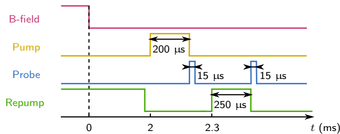
FIGURE 2.8 : Timing of the microwave spectroscopy sequence. After a 200 \mu\text{s} -long microwave pump pulse, a 15 \mu\text{s} -long probe pulse measures the atomic ensemble absorption. An additional probe pulse is sent after a repump stage in order to get a reference for the probe intensity.
