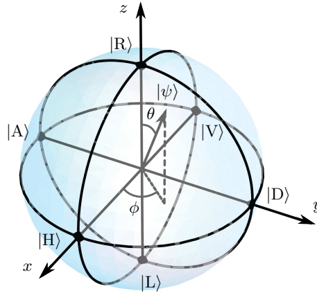
FIGURE 4.6 : Bloch sphere with the |R\rangle and |L\rangle states corresponding to Laguerre-Gaussian modes on the poles, and the general qubit state |\psi\rangle , defining by the angles \theta and \phi . On the equator the |H\rangle , |D\rangle , |V\rangle and |A\rangle states, correspond to Hermite-Gaussian modes.
