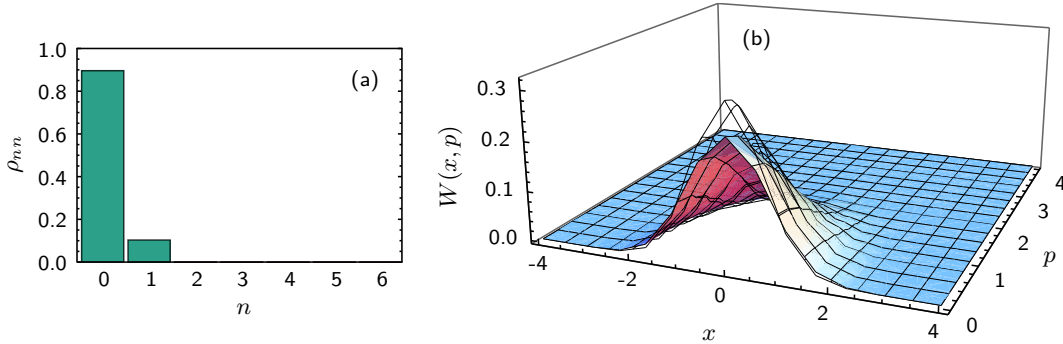
FIGURE 5.9 : Tomography of the retrieved state. (a) Diagonal elements of the reconstructed density matrix and (b) associated Wigner function.
