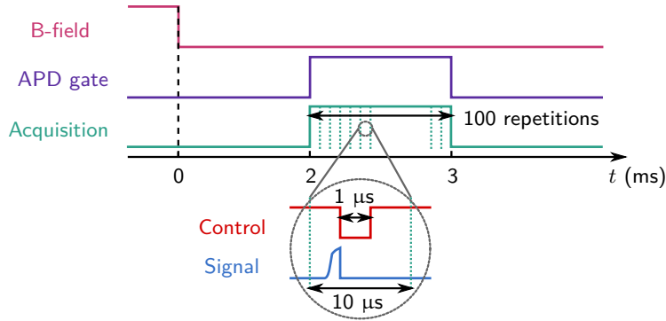
FIGURE C.1 : Timing for the EIT-based memory acquisition. At t = 2 ms, the APD gate and the acquisition trigger signal are switched on, for a duration of 1 ms. During this time, 100 trials of the memory protocol occur, each with a duration of 10 \mu\text{s} . The memory trial involves a control field which is off only during the storage time, and a signal pulse which is sent just before the extinction of the control. The stored signal is then retrieved and detected when the control is turned on again.
