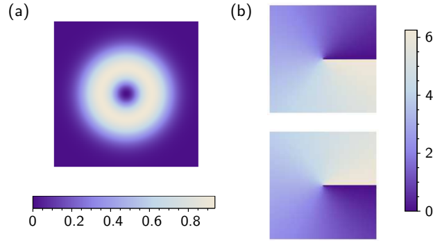
FIGURE D.3 : Laguerre-Gaussian modes LG^{+1} and LG^{-1} . (a) Intensity profiles of the two modes. (b) Phase profile of LG^{+1} and LG^{-1} modes.
