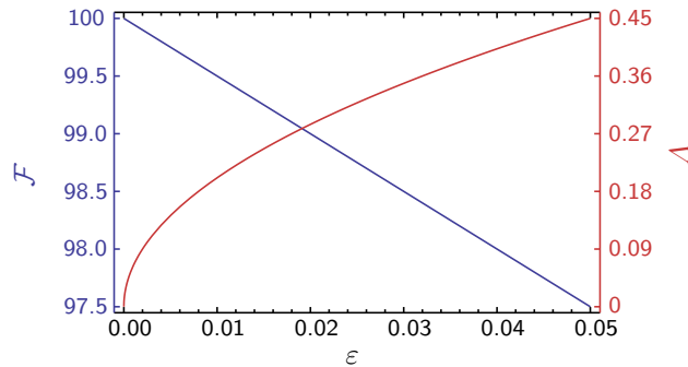
FIGURE E.2 : Fidelity \mathcal{F} and visibility V for the LG states |R\rangle and |L\rangle , as a function of the quantity \varepsilon of LG^l detected on the -l path. The corresponding distinction ratio varies from infinity to -13 dB.
