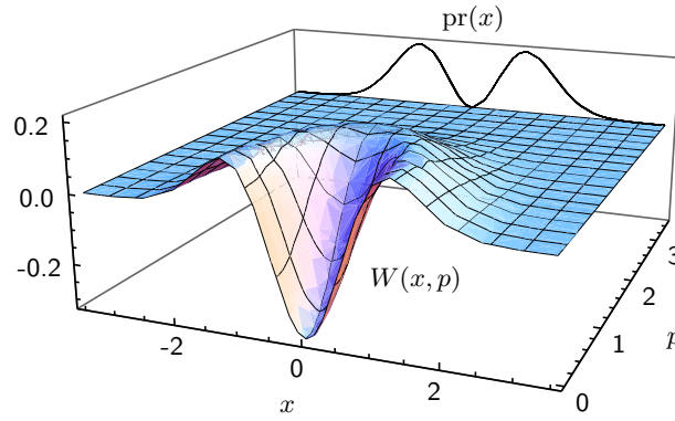
FIGURE 5.5 : The Wigner function W(x, p) and the corresponding probability distribution \text{pr}(x) for a single-photon state.
