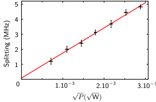
FIGURE 3.7 : Experimental splitting as a function of \sqrt{P} , where P is the control power, fitted by a linear function with a slope of 1670 \pm 100 MHz/ \sqrt{W} .
