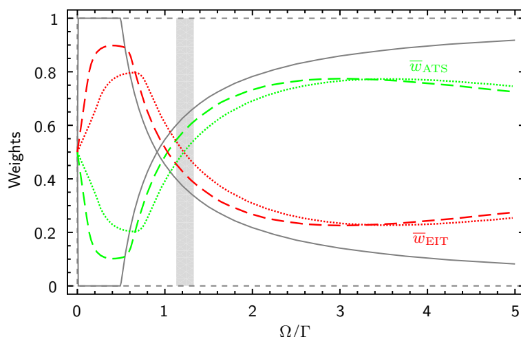
FIGURE 3.11 : Theoretical simulations with Doppler broadening. Per-point weights for a three-level system (gray lines), for a system involving Zeeman structure and residual Doppler broadening of \Gamma_D/2\pi = 0.6 MHz (dashed lines) and 1.3 MHz (dotted lines).
