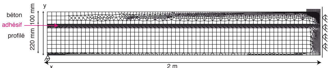
Figure C.1 – Maillage 2D de la poutre AB1
