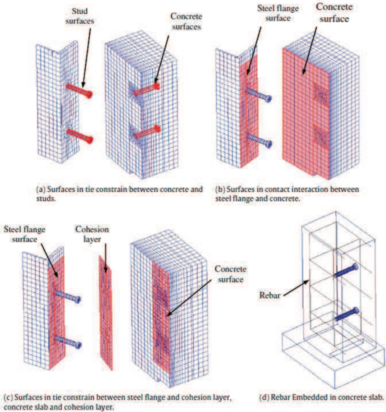
Figure 10.6 – Maillage de l'essai Push Out, surfaces d'interaction (Kim and Nguyen, 2009)
