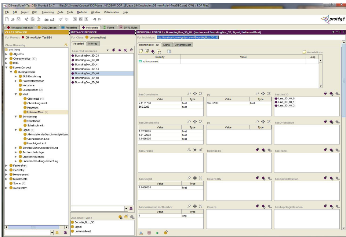
Figure 3.9: OWL represented in the Protégé tool
