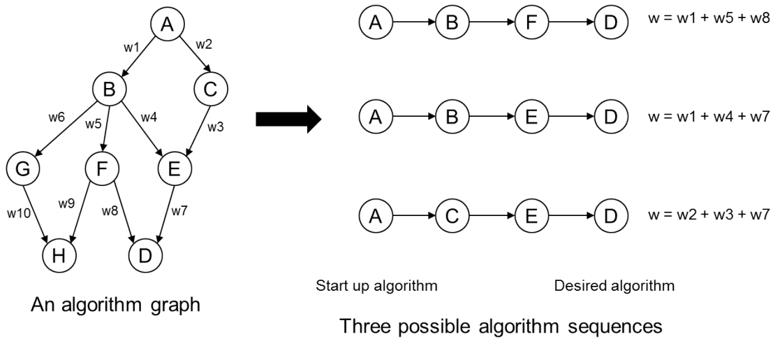
Figure 4.33: Algorithm sequences extracted from the graph. The sequence with minimal weight “w” will be selected.
