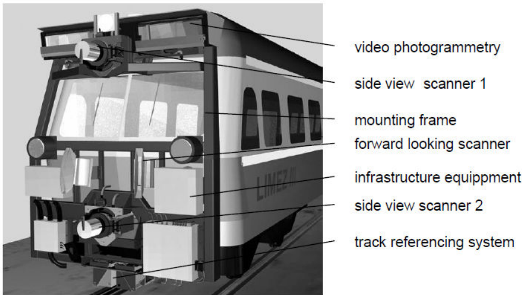
Figure 3.12: LIMEZ III measurement system [Hoefler et al. 2006]
