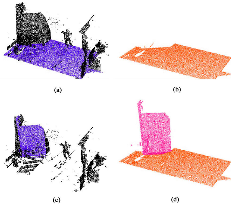
Figure 4.28: Planes extracted by RANSAC algorithm
