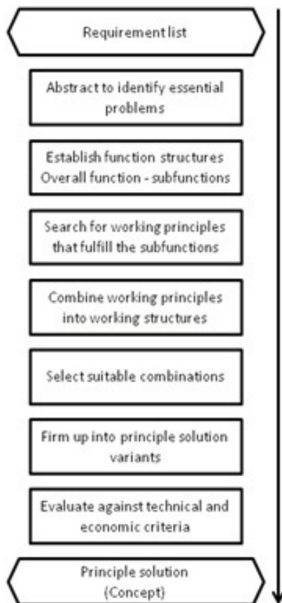
Figure 2.2. The conceptual design phase (Pahl and Beitz, 2007)
