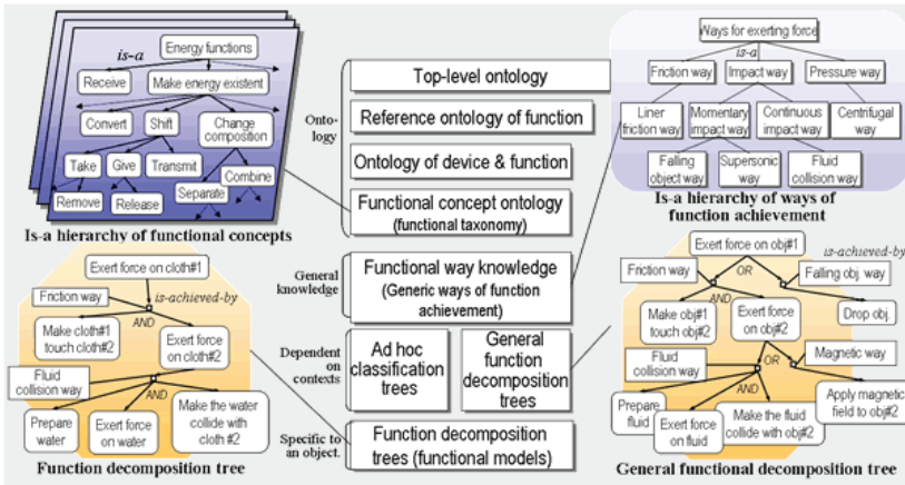
Figure 2.21. Layers of functional ontologies in the FOCUS project (Kitamura et al., 2007)
