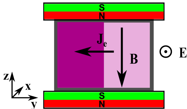
Figure 6.36: Electron drift inside the PEGASES thruster.
