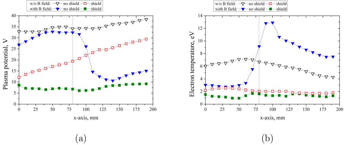
Figure 5.13: (a) Plasma potential and (b) electron temperature distribution along the discharge tube x-axis for 4 operating conditions. The position 0 mm refers to the tube exit. The dashed line indicates the magnetic field peak.
