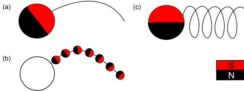
Figure 1.6: (a) Flexible beam attached to a magnetic head. (b) Flexible magnetic micro-bead tail. (c) Rigid helical tail fixed to a magnetic head.
