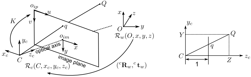
Figure 4.1: Perspective projective model.
