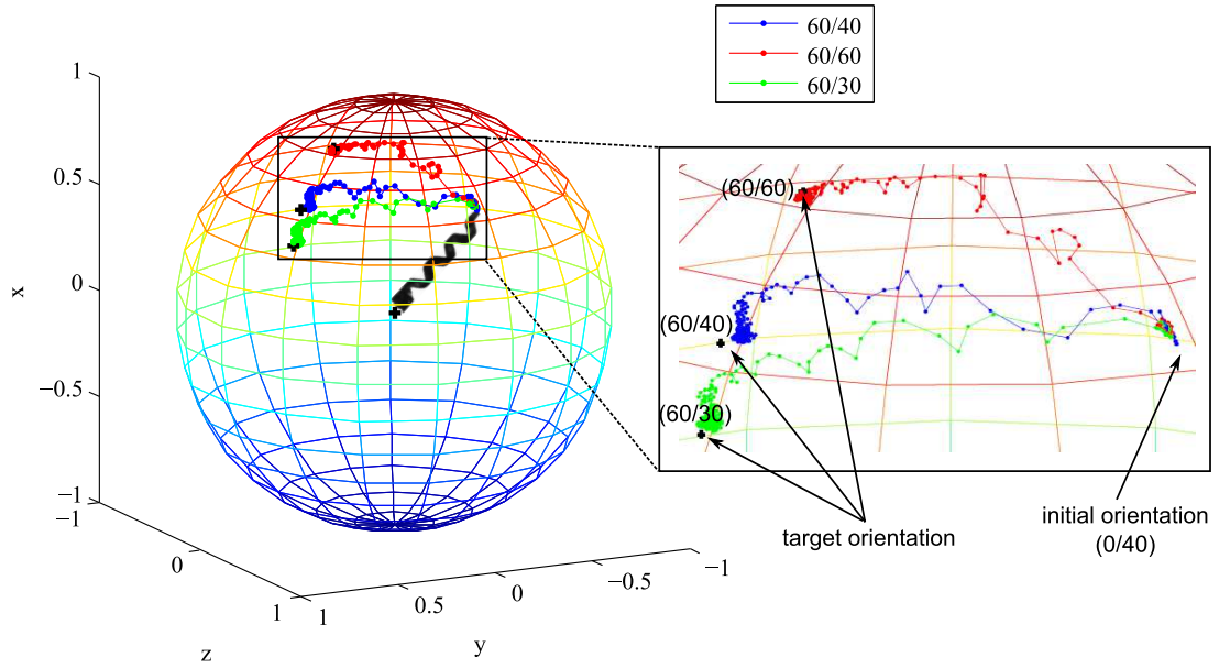
Figure 4.16: Trajectories of the SHM for the visual servoing control for both direction and inclination angles on an unit sphere.
