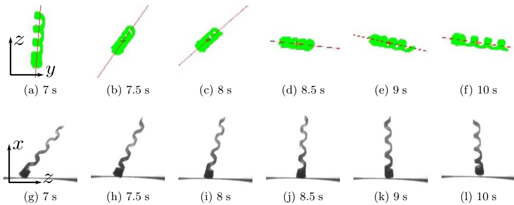
Figure 3.17: Image sequence of 90^\circ angle direction steering with a 45^\circ inclination angle. (a)-(f) show the top view of SHM1-mh8, and (g)-(l) show the side view.
