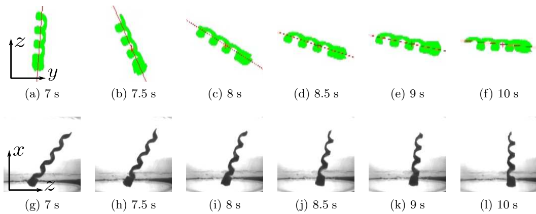
Figure 3.18: Image sequence of -90^\circ angle direction steering with a 45^\circ inclination angle. (a)-(f) show the top view of SHM1-mh8, and (g)-(l) show the side view.
