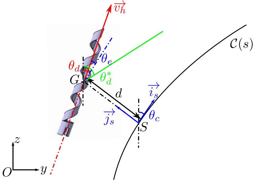
Figure 4.17: Helical swimmer modelling of the 2D path following on the horizontal plane.
