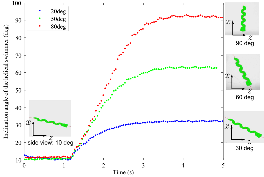
Figure 3.20: Step responses of the inclination angle steering at 30^\circ , 60^\circ , and 90^\circ with the initial inclination angle at 10^\circ .
