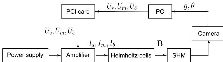
Figure 2.12: Block-diagram of the Helmholtz coils system. The control variables of the system are the output voltages of the PCI card U_s, U_m, and U_b . The frequency and the axis of the rotating magnetic field are controlled. The vision system returns the position ( g ) and orientation ( \theta ) of the SHM.
