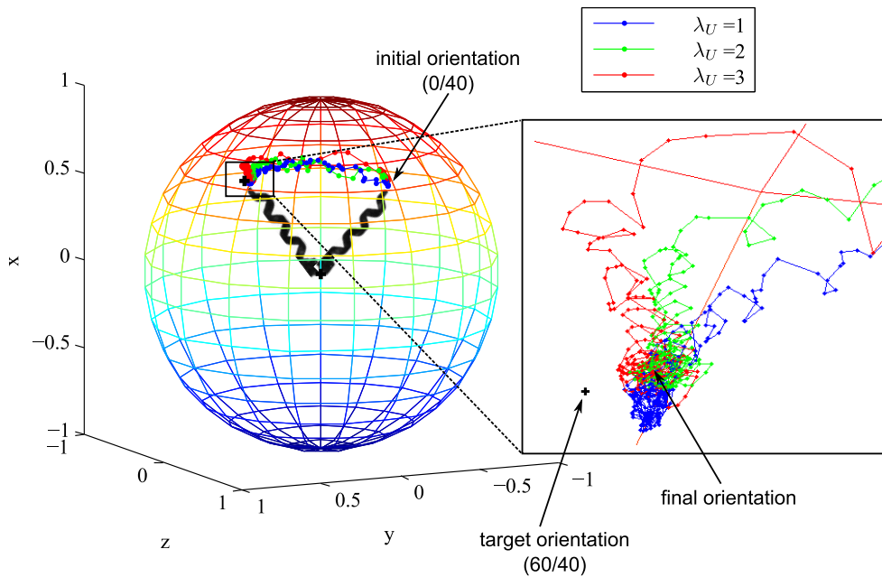
Figure 4.13: Trajectories of SHM1-mh8 for the visual servo control of the direction angle with different control parameters on an unit sphere.
