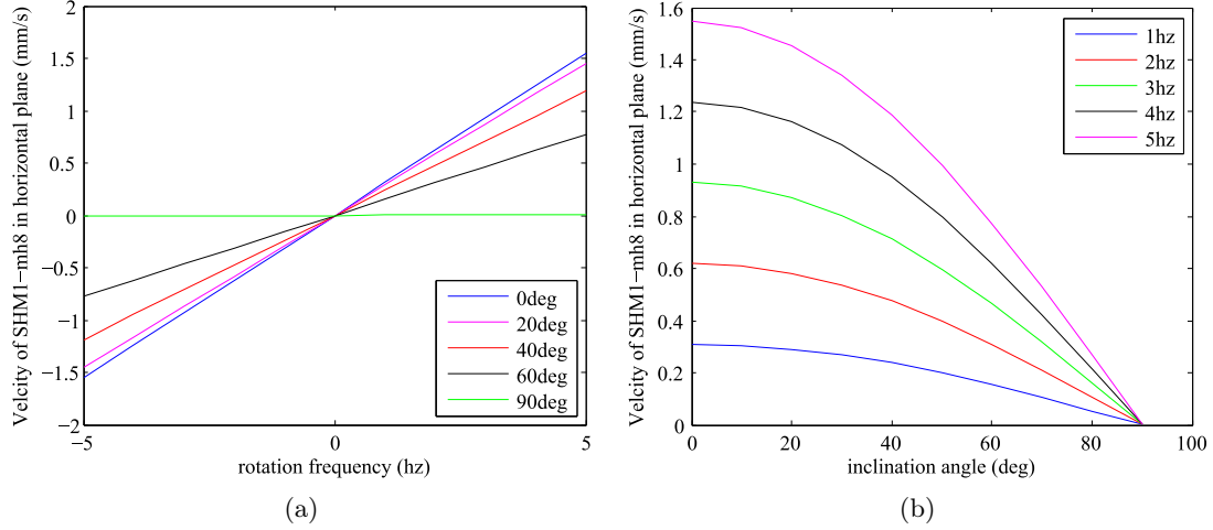
Figure 3.12: Linear advance velocity of SHM1-mh8 sinking down to the bottom on the horizontal plane as a function of (a) the rotation frequency of the magnetic field and (b) the inclination angle based on the propulsion matrix in pure glycerol.
