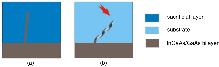
Figure 1.8: (a) InGaAs/GaAs bilayer is patterned by photolithography in a ribbon-like shape for the helical tail. (b) The ribbon-like structure self-forms a helix tethered at one end by releasing the internal stress after wet etching of the sacrificial layer. The red arrow indicates the scrolling direction of the ribbon, i.e., \langle 100 \rangle on a (001) GaAs wafer [Zhang 2010a].
