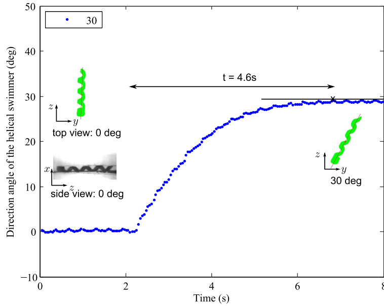
Figure 3.15: Step response to the 30^\circ direction angle steering with a 0^\circ inclination angle.
