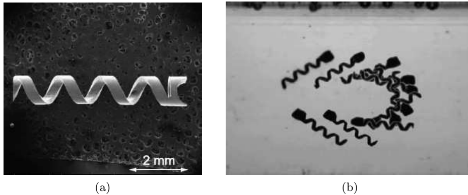
Figure 1.15: (a) Scanning electron micrograph of the fabricated helix. (b) Image sequence of a "U-turn" trajectory [Mahoney 2011].
