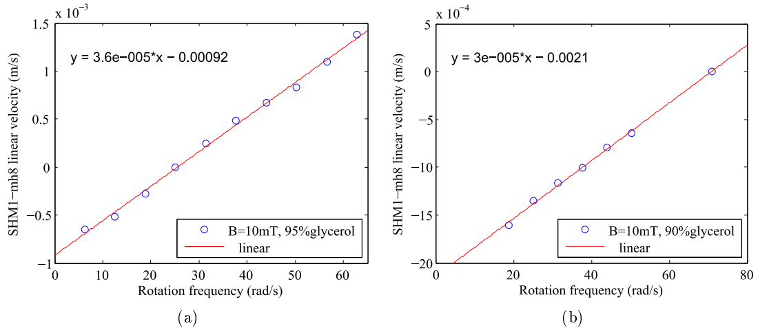
Figure 3.7: Translation velocity of SHM1-mh8 as a function of rotation frequency in (a) 95% glycerol and (b) 90% glycerol solutions with a 10 mT magnetic field. The red line is the linear regression by Matlab.
