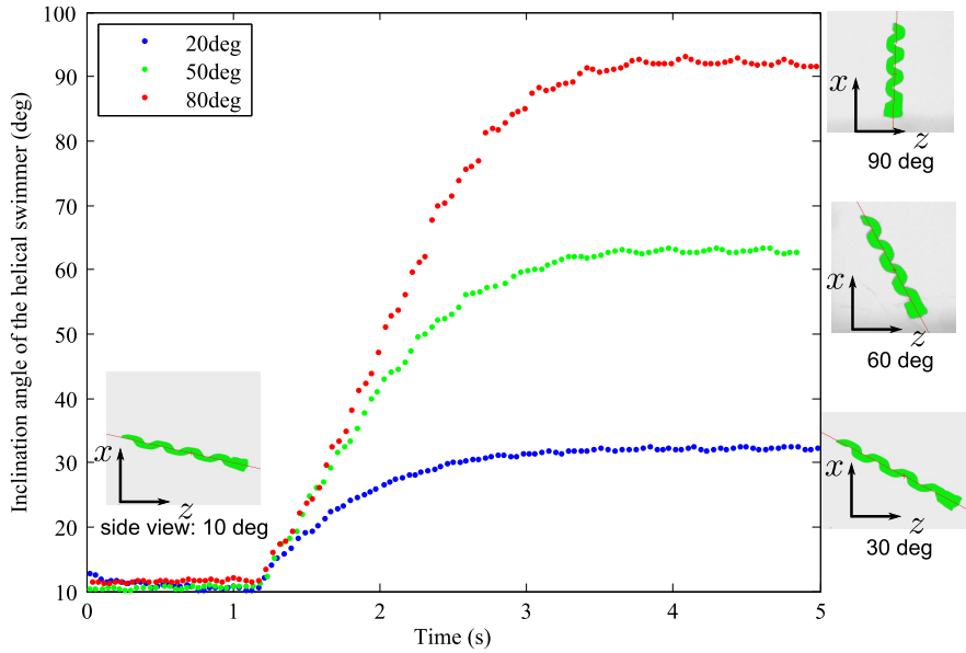
Figure 3.19: Step responses of the inclination angle steering at 30^\circ , 60^\circ , and 90^\circ with the initial inclination angle at 10^\circ .
