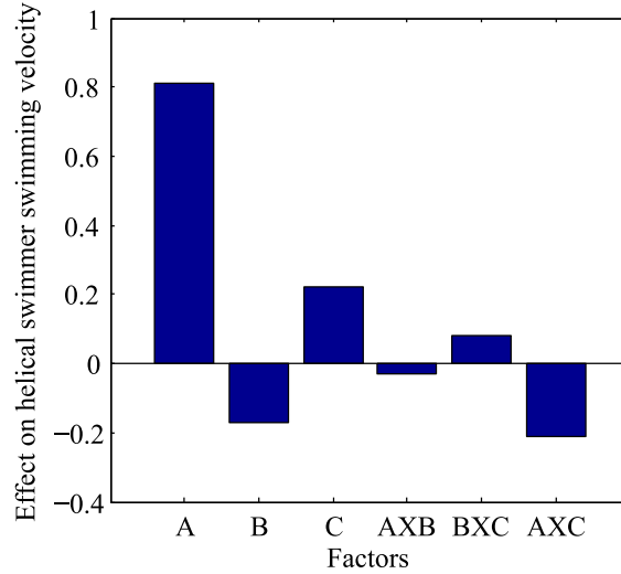
Figure 3.1: Effect of factors and the interactions on swimming velocity.
