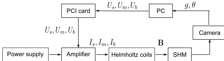
Figure 2.12: Schema of the Helmholtz coils system. The control variables of the system are the output voltages of the PCI card U_s, U_m, U_b . The frequency and the axis of the rotating magnetic field are controlled. The vision system returns the position ( g ) and orientation ( \theta ) of the SHM.
