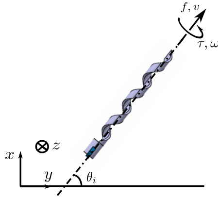
Figure 3.8: Inclination angle \theta_i is defined as the angle between the axis of the SHM and the horizontal plane yOz .
