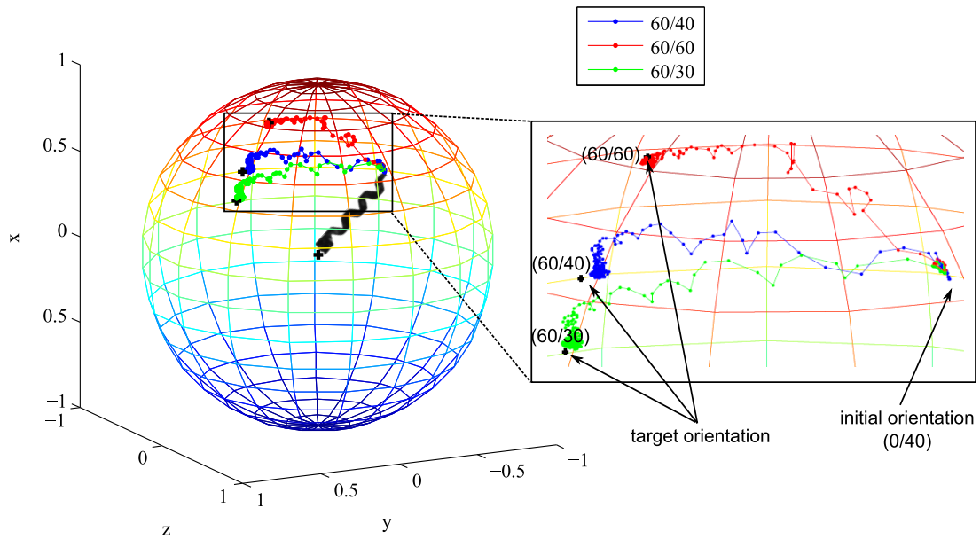
Figure 4.16: Trajectories of the SHM for the visual servo control for both direction and inclination angles on a unit sphere.
