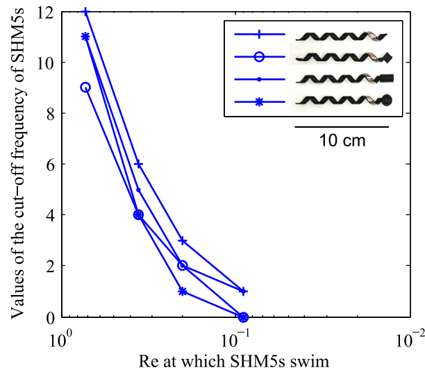
Figure 3.5: Values of the cut-off frequency of SHM5s with the same geometry parameters and magnetic positioning, but with different head shapes.
