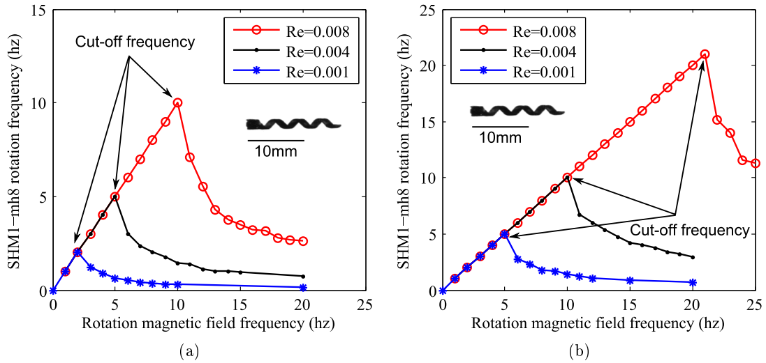
Figure 3.2: Rotation frequency of SHM1-mh8 in a rotating magnetic field generated by a 3D Helmholtz coil pairs with magnetic fields of (a) 5 mT and (b) 10 mT. SHM1-mh8 shows a cut-off frequency with a gentle decline.
