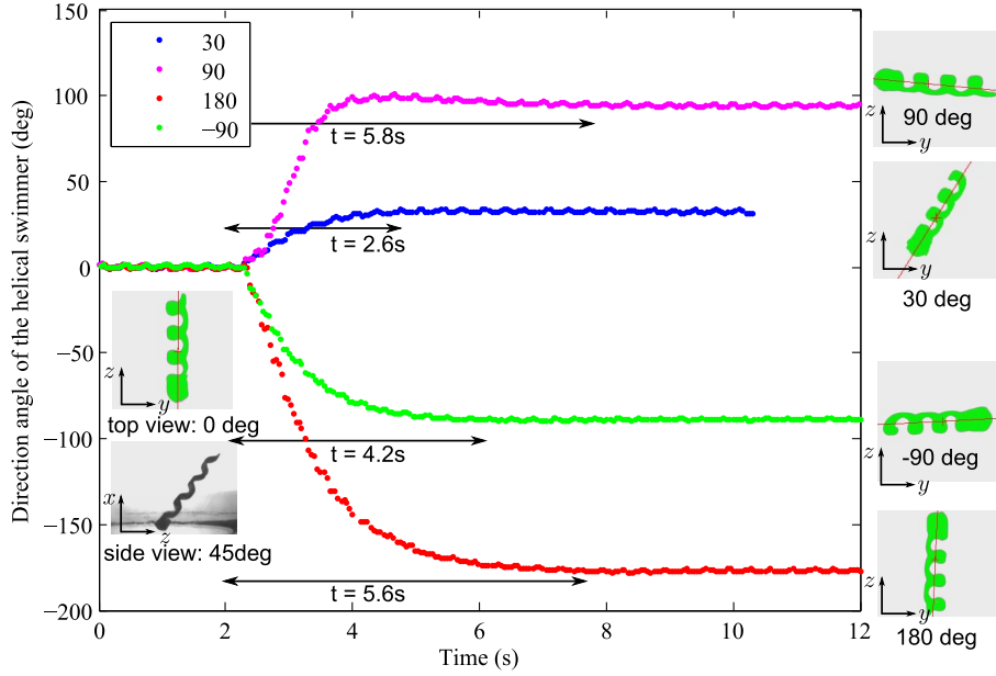
Figure 3.15: Step responses to the 30^\circ , 90^\circ , 180^\circ , and -90^\circ angle direction steering with a 45^\circ inclination angle.
