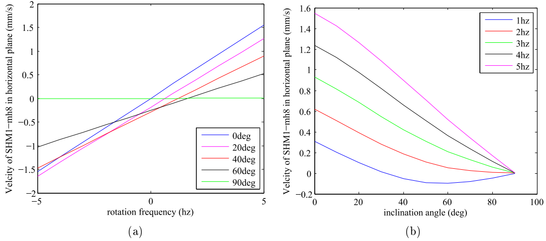
Figure 3.10: Estimated linear advance velocity of floating SHM1-mh8 on the horizontal plane as a function of (a) the rotation frequency of the magnetic field and (b) the inclination angle based on the propulsion matrix in pure glycerol.
