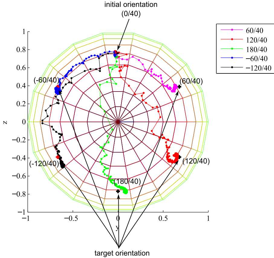
Figure 4.15: Trajectories of SHM1-mh8 for the visual servo control of different direction angles with inclination angle of 40^\circ on an unit sphere.
