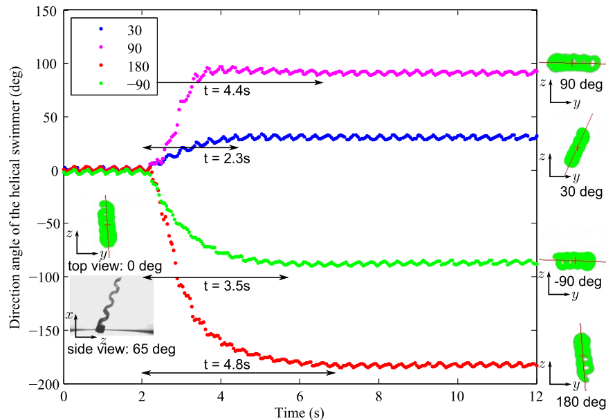
Figure 3.18: Step responses to the 30^\circ , 90^\circ , 180^\circ , and -90^\circ direction angle steering with a 65^\circ inclination angle.
