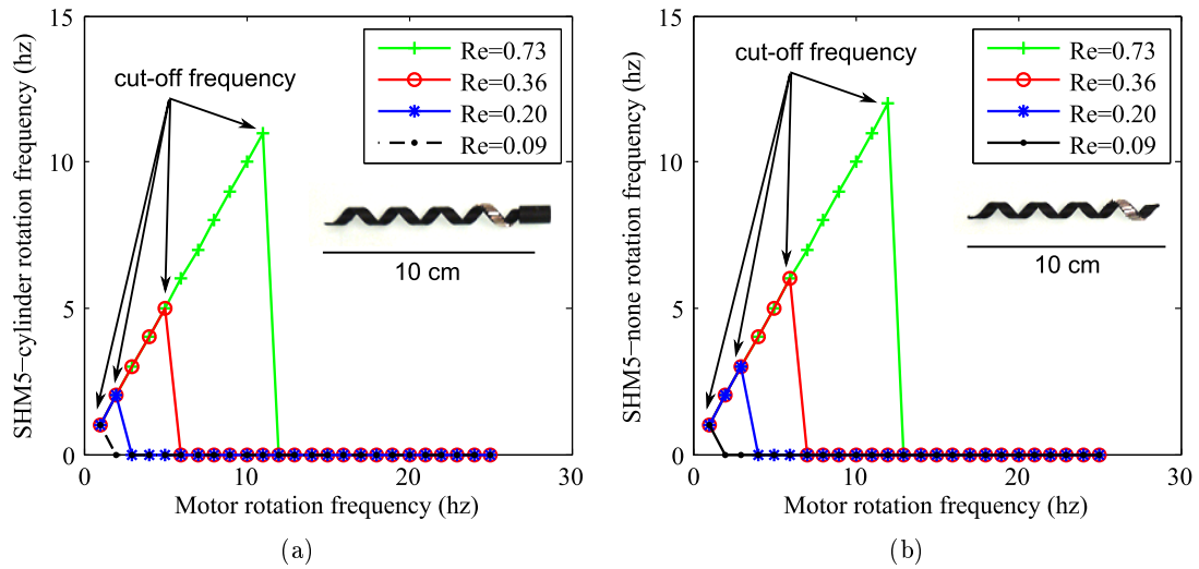
Figure 3.4: Both (a) SHM5-cylinder and (b) SHM5-none with a non-uniformly coated magnetic layer exhibit a cut-off frequency with a brutal stop with a magnetic field about 30 mT generated by a RPMM.
