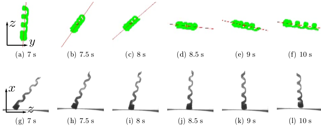
Figure 3.16: Image sequence of 90^\circ angle direction steering with a 45^\circ inclination angle. (a)-(f) show the top view of SHM1-mh8, and (g)-(l) show the side view.
