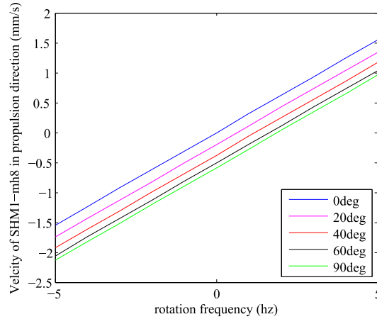
Figure 3.9: Estimated propulsion velocity of SHM1-mh8 in the propulsive direction based on the propulsion matrix in pure glycerol.
