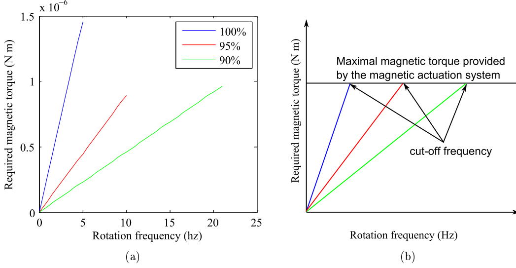
Figure 3.12: (a) Simulated magnetic torque required for the propulsion of SHM1-mh8 in different viscous liquids based on the estimated propulsion matrices. (b) Theoretical magnetic torque required for the propulsion of a helical swimmer in different viscous liquids.
