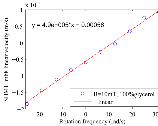
Figure 3.6: Translation velocity of SHM1-mh8 as a function of rotation frequency in glycerol with a 10 mT magnetic field. The red line is the linear regression by Matlab.
