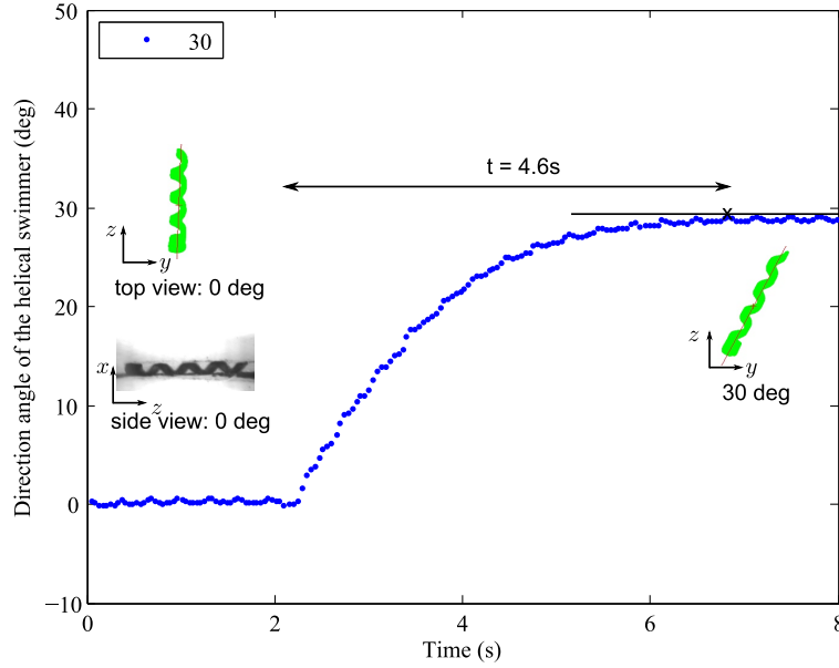
Figure 3.14: Step response to the 30^\circ direction angle steering with a 0^\circ inclination angle.
