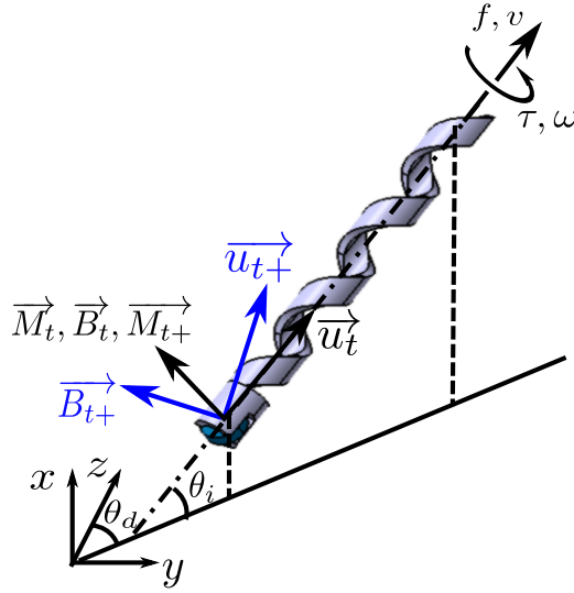
Figure 3.13: Magnetic helical swimmer steering model. The inclination angle and direction angle of steering are respectively \theta_i and \theta_d .
