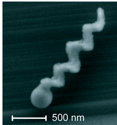
Figure 1.14: SEM image of an individual glass screw with nano-structured helicity [Ghosh 2009].
