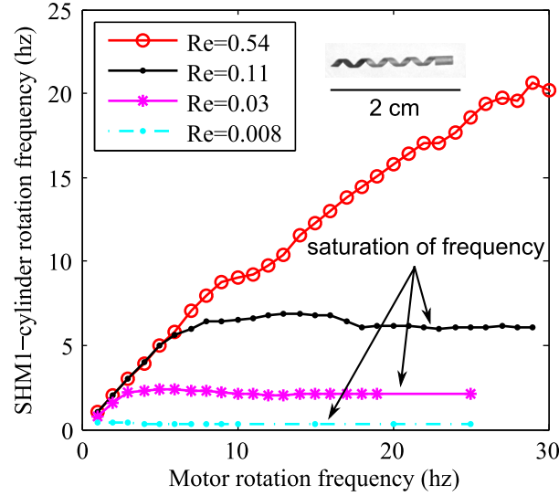
Figure 3.3: SHM1-cylinder with a 20 – 50 \mu\text{m} thick coated magnetic layer shows a saturation of frequency with a magnetic field of about 30 mT generated by a RPMM.
