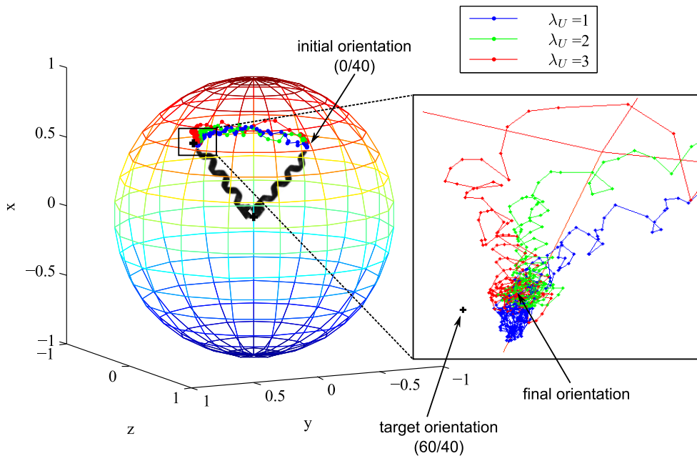
Figure 4.13: Trajectories of SHM1-mh8 for the visual servo control of the direction angle with different control parameters on a unit sphere.
