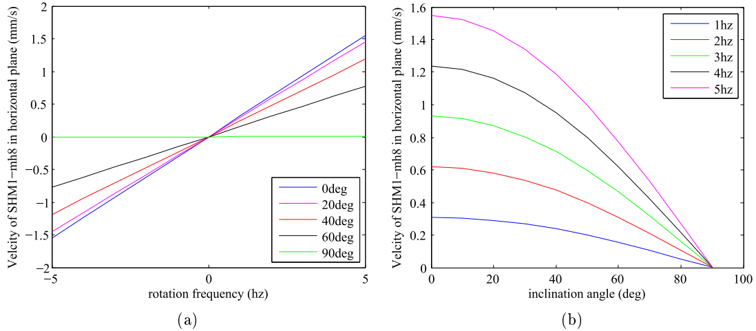
Figure 3.11: Linear advance velocity of SHM1-mh8 sinking down to the bottom on the horizontal plane as a function of (a) the rotation frequency of the magnetic field and (b) the inclination angle based on the propulsion matrix in pure glycerol.
