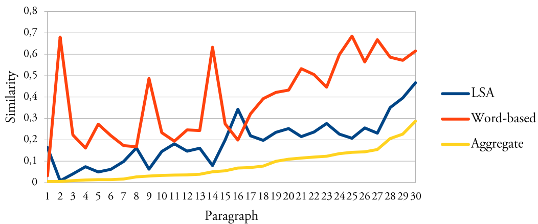
Figure 51. Comparison between the LSA similarity and word-based heuristics.
