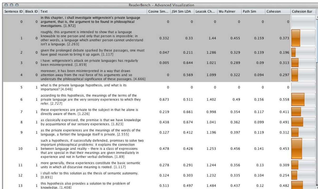
Figure 76. ReaderBench Document advanced visualization.
