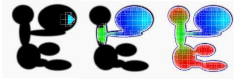
Figure 2.7: Figure extracted from [Droske 2001]. Adaptive grid sampling, progressively constructed as the front progresses. The colors indicates the arrival time of the propagation (from blue (early) to red)
