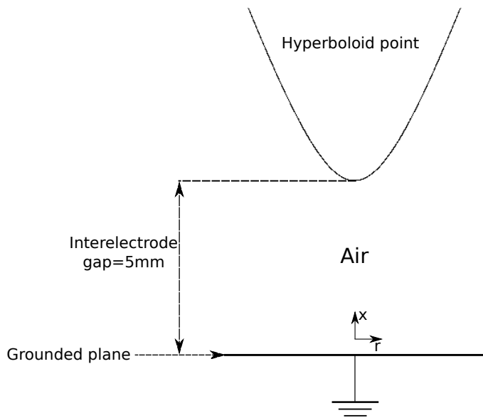
Figure 1.3: Discharge set-up for the TC-1.
