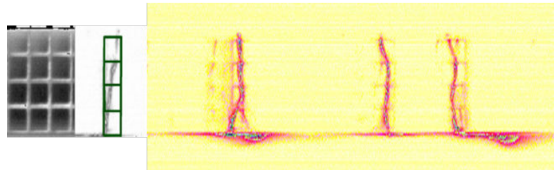
Figure 1: Left : face view of a monolith of cordierite. Right : Light emission from plasma filaments created in a honeycomb monolith of cordierite, with 1 mm 2 channel section. (Tardiveau et al. 2005)
