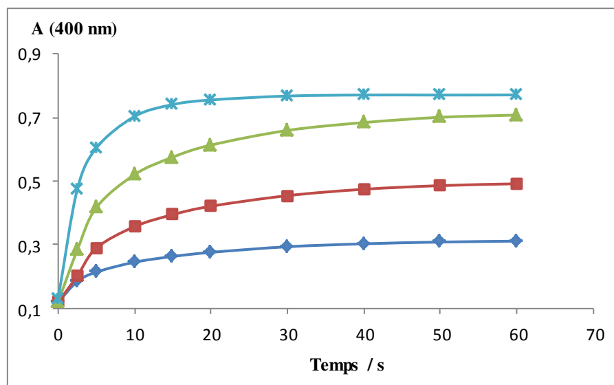
Figure III.14: Suivi cinétique de la complexation rutine - \text{Fe}^{\text{III}} (tampon acétate 0.1 M, pH 5, 25°C). ◆ \text{Fe}^{\text{III}} / rutine = 0,25, ■ \text{Fe}^{\text{III}} / rutine = 0,5, ▲ \text{Fe}^{\text{III}} / rutine = 1, x \text{Fe}^{\text{III}} / rutine = 2. Concentration de rutine = 50 \mu\text{M} .
