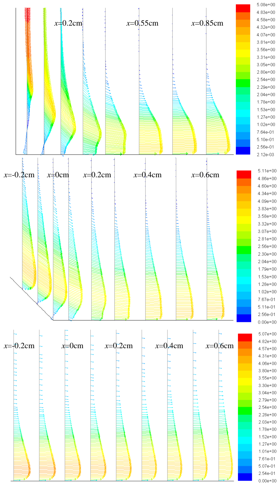
Figure 5.12. Vertical velocity profiles above the fixed plane as a function of the angle of the inclined plane, for 90°, 135° and 180°.
