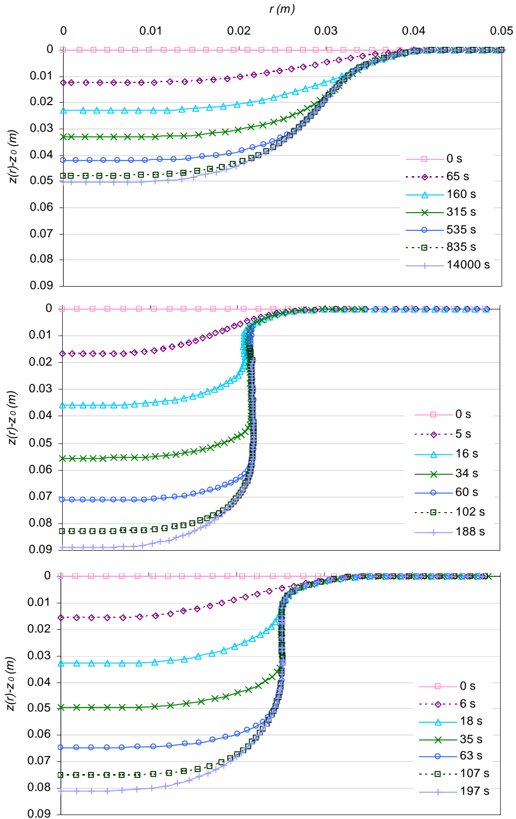
Figure 3.29. Evolution of the soil/water interface as a function of time with, from top to bottom, graphs corresponding to the tests performed on soils A, B and C, model k-\omega .
