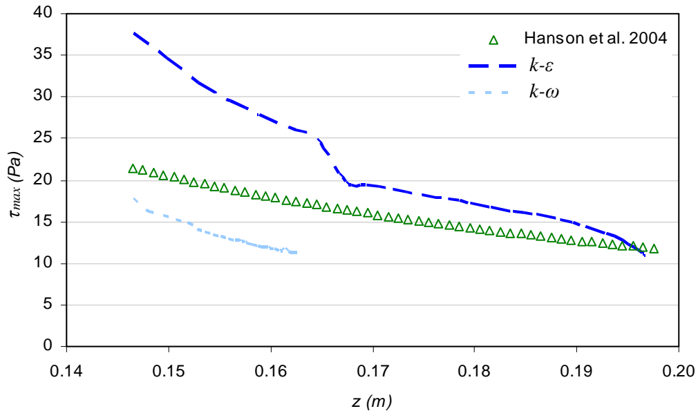
Figure 3.11. Evolution of maximum shear stress as a function of scour depth at different times for models k-\varepsilon and k-\omega in comparison to the results of the model of [Hanson and Cook 2004].
