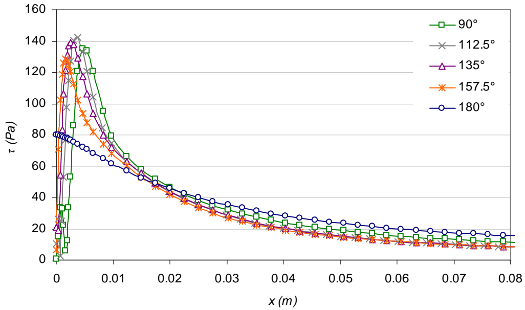
Figure 5.14. Results obtained for the shear stress on the horizontal plane as a function of the inclined plane.
