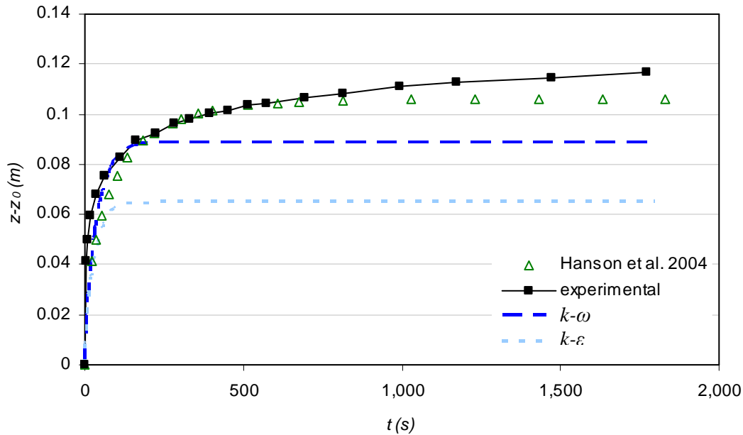
Figure 3.27. Comparison of numerical results for turbulence models k-\omega and k-\varepsilon , with the experimental and semi-empirical results for the test on soil B.
