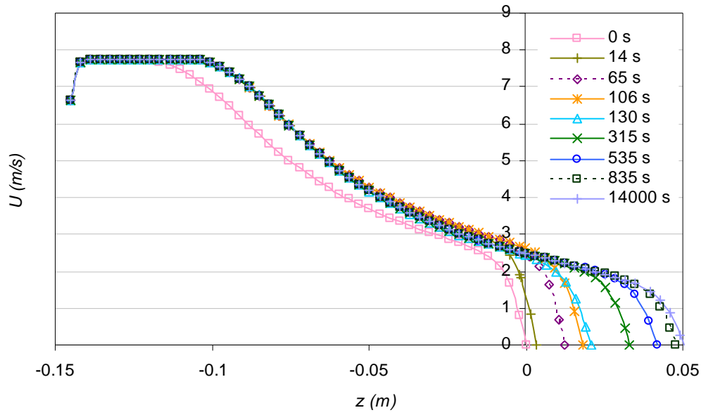
Figure 3.12. Evolution of the velocity field on the jet centreline, model k-\omega .
