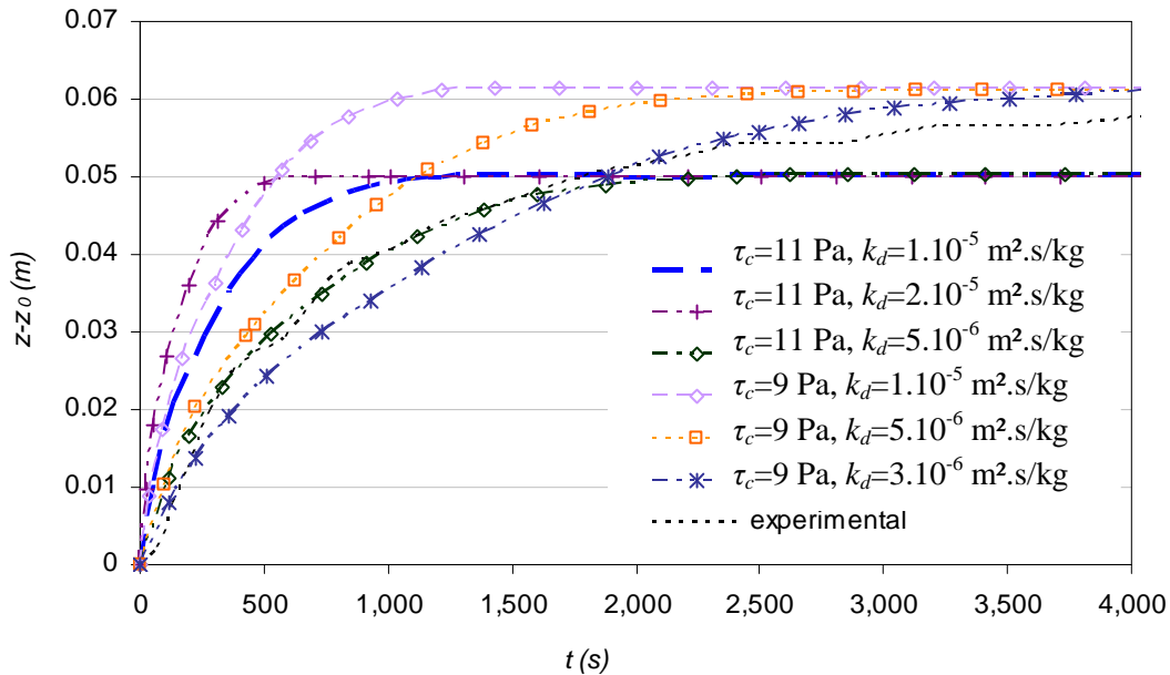
Figure 3.17. Parametric study of the influence of critical shear stress on the evolution of scour depth as a function of time for the turbulence model k-\omega , \tau_c=11 Pa or \tau_c=9 Pa.
