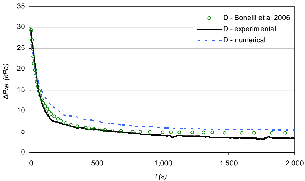
Figure 4.30. Comparison of numerical, experimental and semi-empirical results for the HET on soil D.
