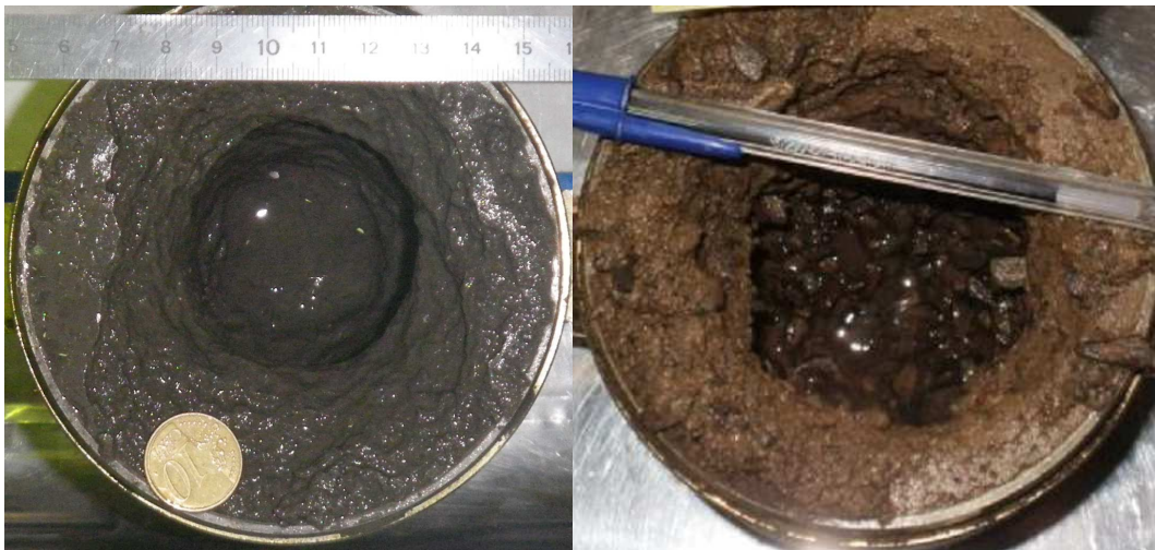
Figure 2.2. Illustration of standard erosion figures obtained following Jet Erosion Tests (C. Moras - geophyConsult).
