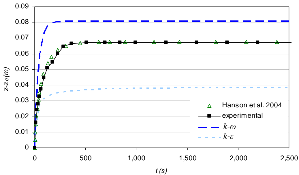
Figure 3.28. Comparison of numerical results for turbulence models k-\omega and k-\varepsilon , with the experimental and semi-empirical results for the test on soil C.
