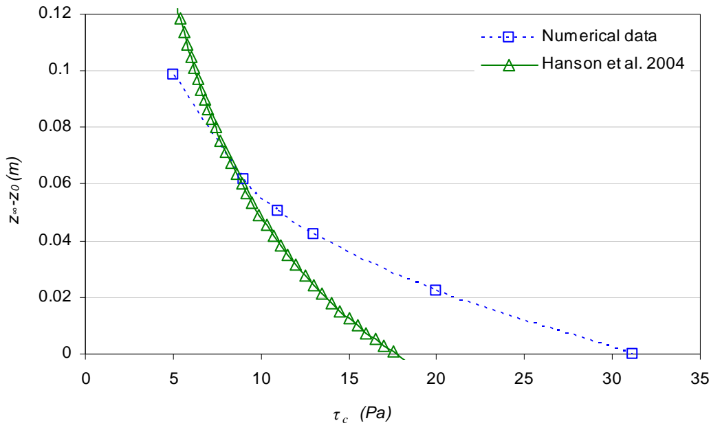
Figure 3.20. Maximum scouring as a function of the critical shear stress, model k-\omega , k_d = 10^{-5} \text{ m}^2 \cdot \text{s/kg} .
