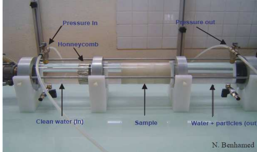
Figure 1.3. Photograph of the experimental Hole Erosion Test device.
