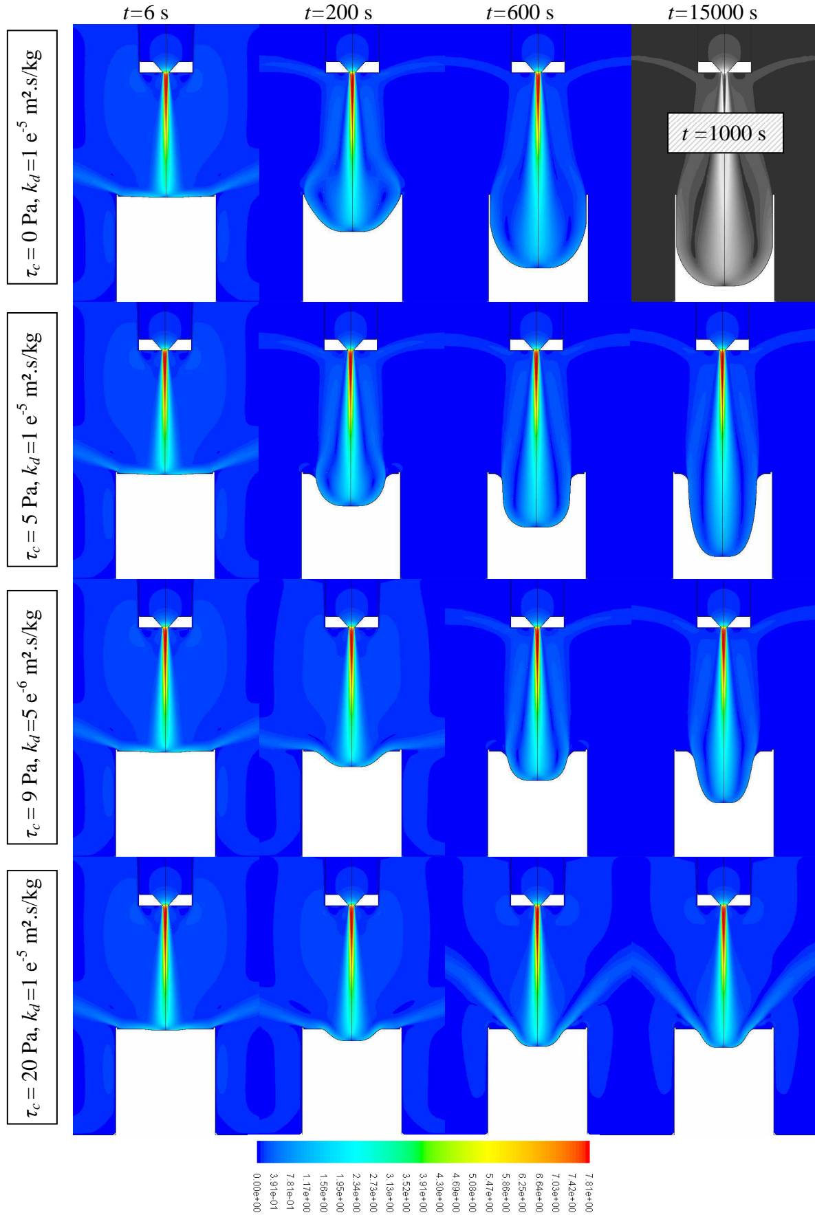
Figure 3.18. Velocity fields relative to the parametric study at times t = 6 s, t = 200 s, t = 600 s and t = 15000 s, model k-\omega .
