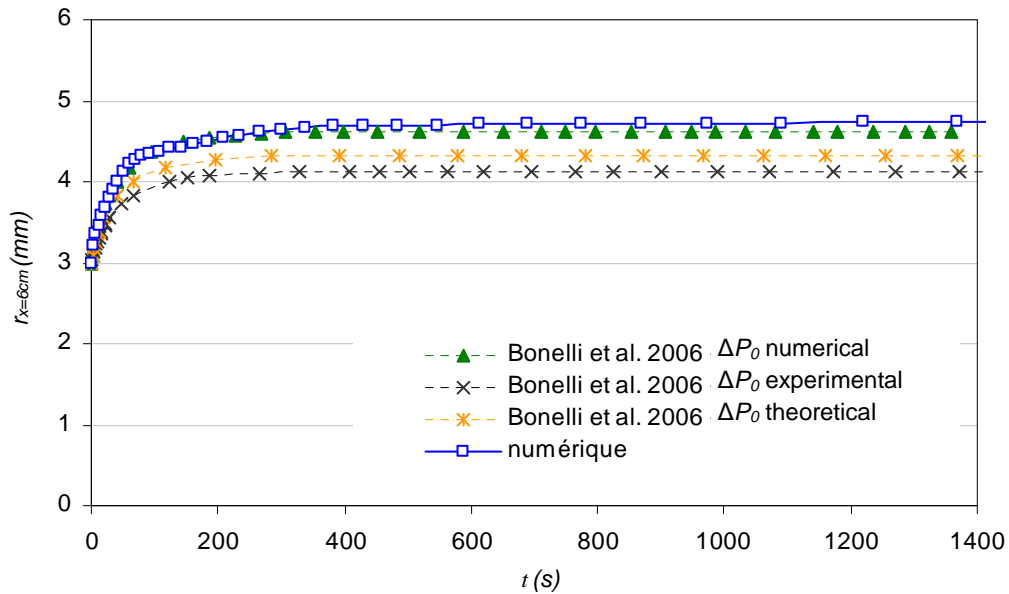
Figure 4.18. Evolution of the radius of the pipe diameter . Comparison of the numerical results and the model of [Bonelli et al. 2006].
