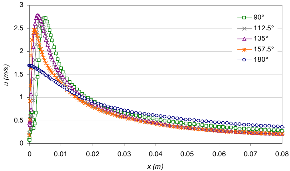
Figure 5.19. Results obtained for the flow velocity above the horizontal plane as a function of the angle of the inclined plane.
