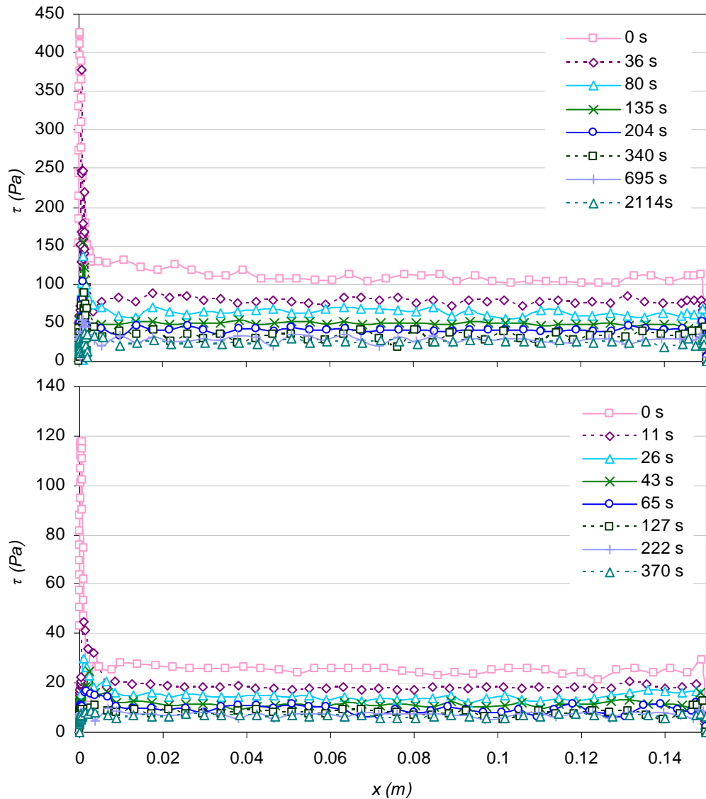
Figure 4.36. Evolution of shear stress at the water/soil interface as a function of time, with from top to bottom the graphs corresponding to the tests carried out on soils D and E.
