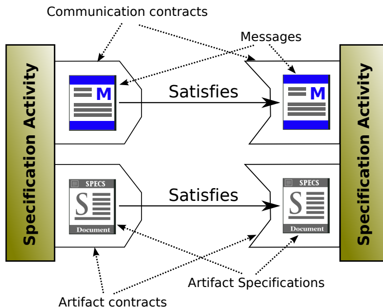
Figure 4.11 – Contracts for Specification Activities
