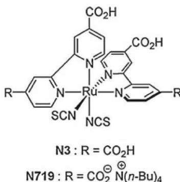
Figure I-19: Structure des colorants N3 et N719 [289].
