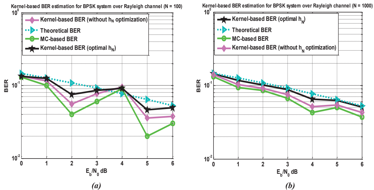
Figure 3.13 — Kernel-based BER estimation for BPSK signal over Rayleigh channel when (a). N = 100 , (b). N = 1000
