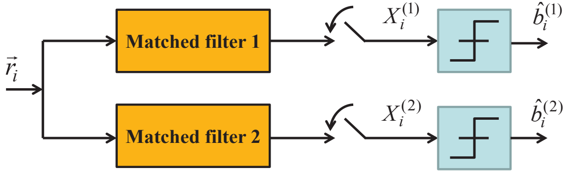
Figure 3.15 — Standard receiver
