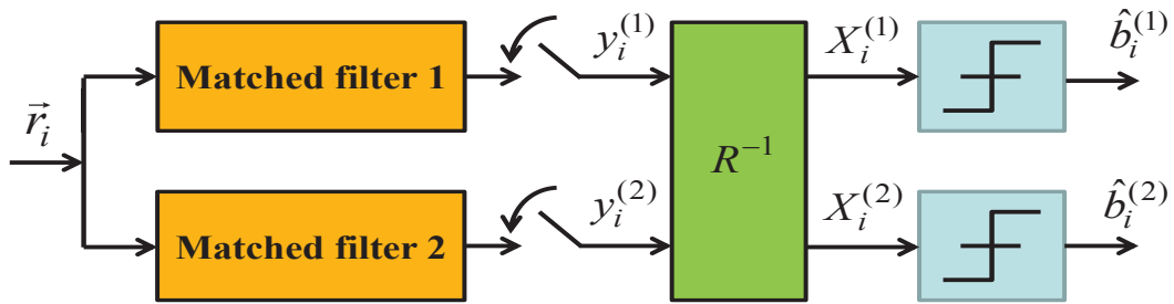
Figure 3.18 — Decorrelator-based receiver
