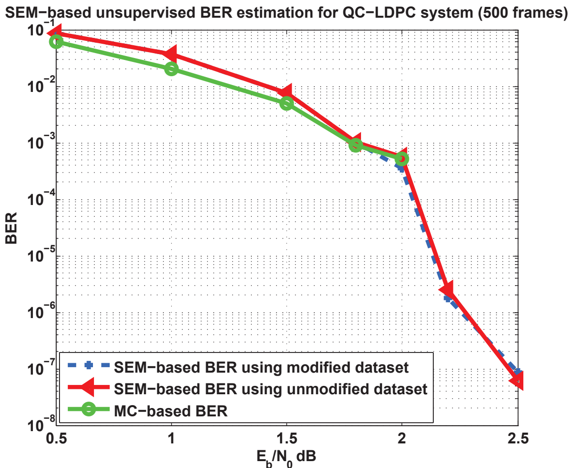
Figure 5.11 — Behavior of the modified SEM-based BER estimation using Kernel method for uniform sources (QC-LDPC system, 500 frames, \pi_+ = \pi_- = 0.5 )
