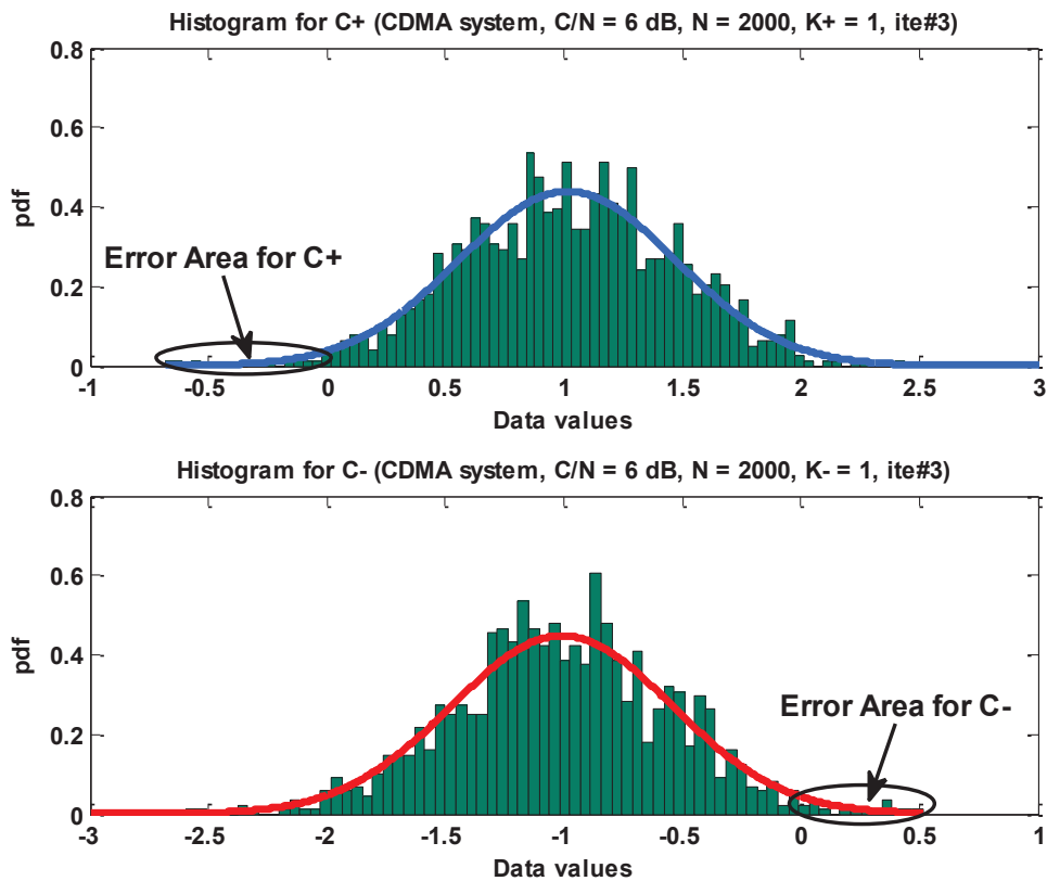
Figure 4.13 — Histograms and GMM-based PDF estimates for CDMA system over AWGN ( SNR = 6\text{ dB} , N = 2000 , K = 1 , T = 3 )
