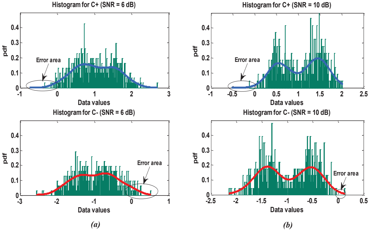
Figure 3.17 — Histograms and Kernel-based PDF estimates for standard CDMA receiver when (a). SNR = 6 \text{ dB} , (b). SNR = 10 \text{ dB} and N = 1000
