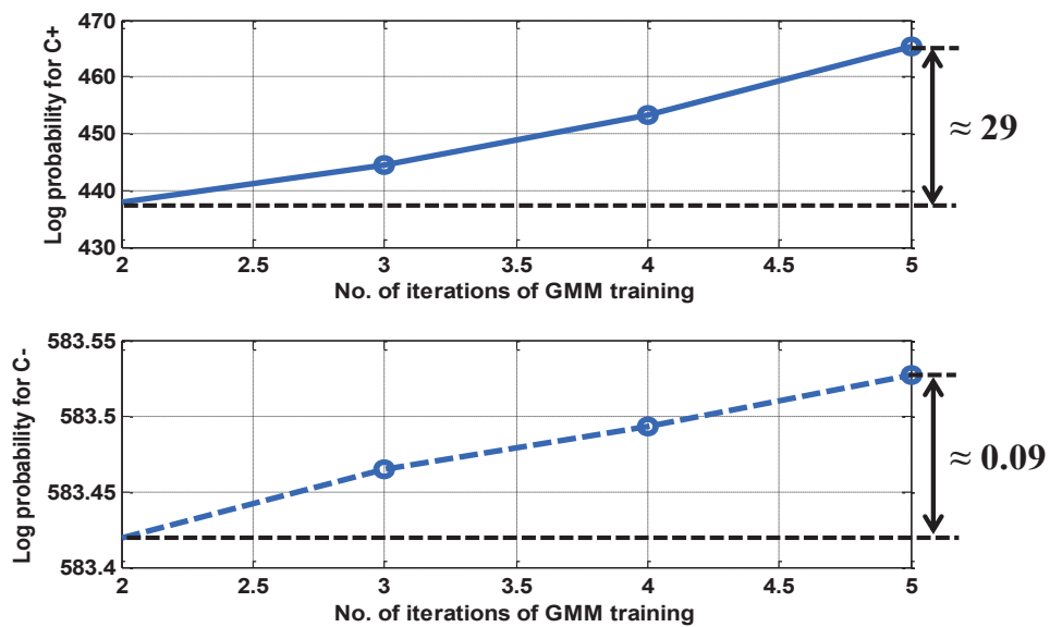
Figure 4.11 — Log-likelihood probabilities for decorrelator-based CDMA system ( N = 2000, K = 5, SNR = 20 \text{ dB}, T = 5 )
