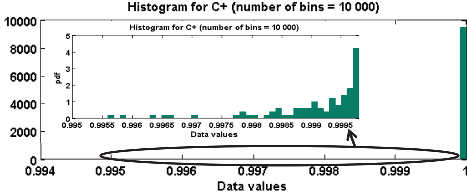
Figure 3.23 — Histogram of the soft output ( C_+ ) for QC-LDPC system when SNR = 2.2 \text{ dB}
