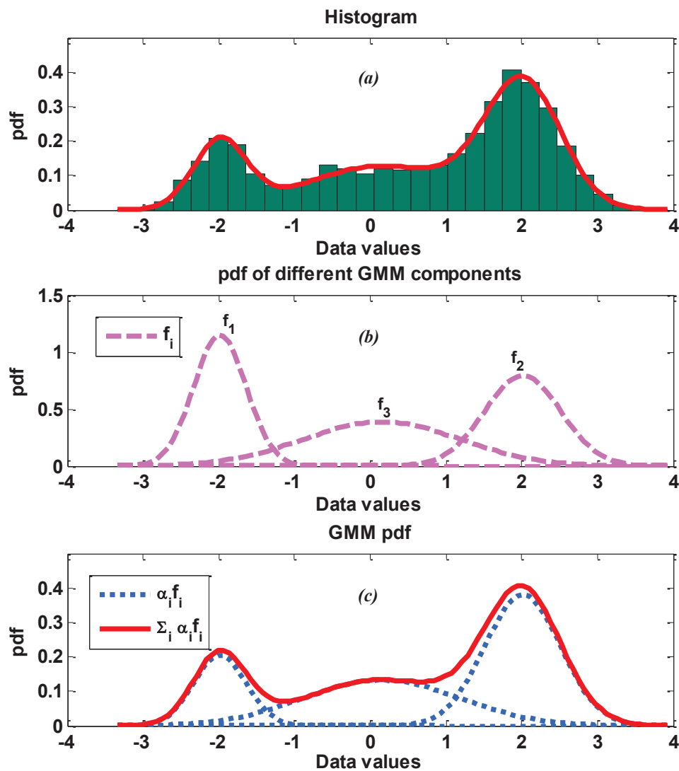
Figure 4.2 — PDF estimates based on GMM with 6000 samples : (a). Histogram compared with the final result of estimated PDF ; (b). PDF of the three Gaussian components ; (c). Final result of estimated PDF
