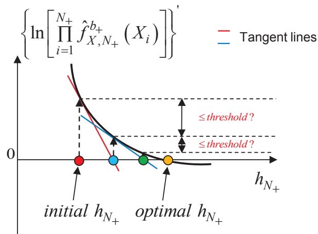
Figure 3.10 — Principal of Newton’s method
