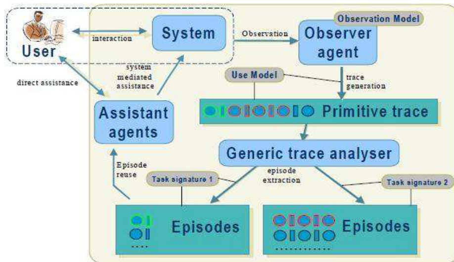
Figure 1 Approche MUSETTE (Champin et al., 2004)
