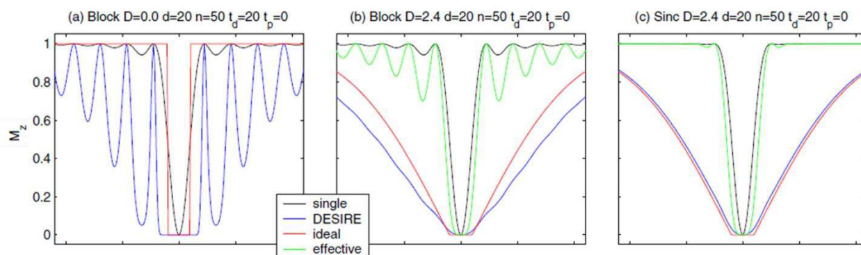
Figure 33. Simulated 1D magnetization profiles, for 20 \mu\text{m} aimed saturation size and 50 pulse repetitions with 20 ms inter-pulse delay. (a) Square pulse shape and no diffusion: the profile difference between the single pulse and the DESIRE pulse train (50 repetitions) is obvious on the sinc sidelobes. (b) With diffusion, the impact of direct saturation on effective resolution is attenuated but not eliminated. (c) The choice of a pulse shape will less intrinsic imperfections (sinc vs square) dramatically improves the agreement between ideal and effective profiles: direct saturation leads to an increase in the effective main lobe width only. From (Weiger et al., 2008b).
