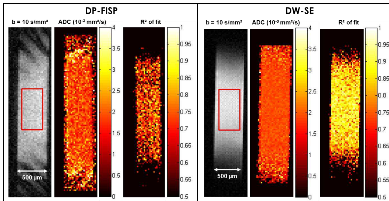
Figure 45. ASW phantom imaged with DP-FISP (left) and DW-SE (right), and parametric maps of ADC and quality of fit ( R^2 ). The resolution is 25 \mu\text{m} isotropic. Statistics over the central square regions: DP-FISP: \text{ADC} = 1.9 \pm 0.3 \cdot 10^{-3} \text{ mm}^2/\text{s} ; R^2 = 0.7 \pm 0.1 . DW-SE: \text{ADC} = 1.9 \pm 0.1 \cdot 10^{-3} \text{ mm}^2/\text{s} ; R^2 = 0.87 \pm 0.05 .
