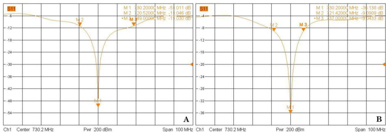
Figure 13. Reflection spectra of the ganglia coil (A) and of the cell coil (B) circuits. The attenuation at the resonant frequency (730.2 MHz) is sufficient to assume zero reflection (> 20 dB from baseline). The quality factor is determined by measuring the bandwidth at half reflection (-3 dB from baseline), but the measurement is somewhat biased by the presence of a second resonance, likely originating from the circuit board tracks forming a loop.
