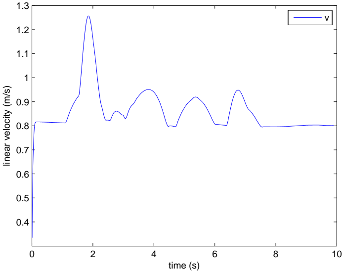
Figure 5.22: Linear velocity control with only S_{rep}(\theta, \omega)
