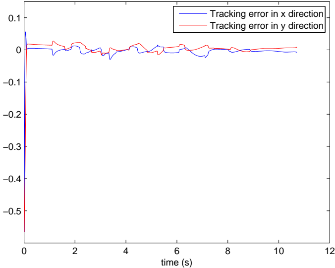
Figure 5.29: Tracking errors with both S_{rep}(\theta, \omega) and S_{rep}(\mathbf{P}, \mathbf{v})
