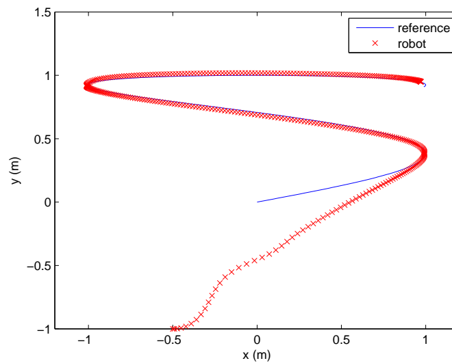
Figure 4.1: Trajectory tracking result without noise
