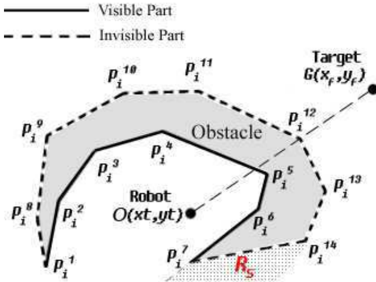
Figure 3.6: Complex Environment
