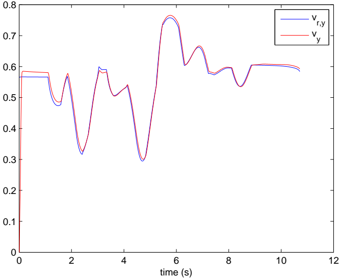
Figure 5.28: Velocity tracking in y direction with both S_{rep}(\theta, \omega) and S_{rep}(\mathbf{P}, \mathbf{v})
