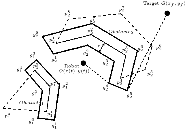
Figure 6.2: Polygon generation
