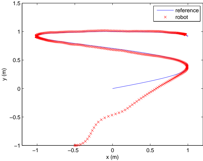
Figure 4.10: Trajectory tracking result with white Gaussian noise SNR = 30dB
