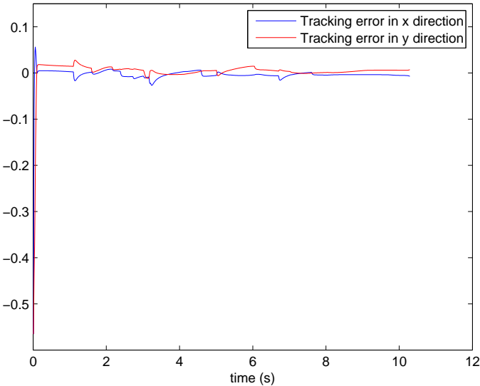
Figure 5.21: Tracking errors with only S_{rep}(\theta, \omega)
