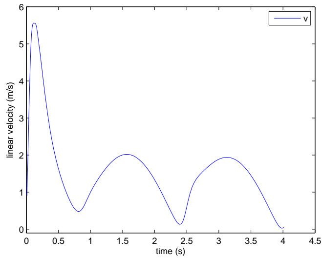
Figure 4.5: Linear velocity control without noise
